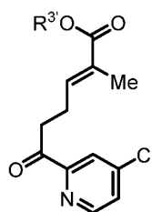
Compound 18
