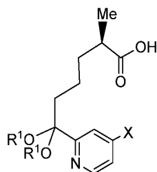
Compound 27
