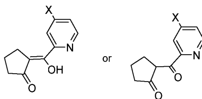
Compound 3a
