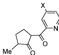
Compound 23b
