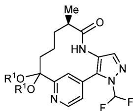
Compound 11;
