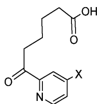
Compound 4
