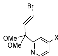
Compound 31
