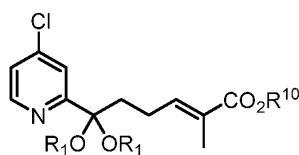
Compound 19
