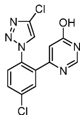
Compound 14
