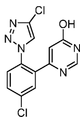
Compound 14
