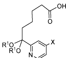
Compound 6
