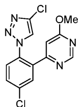
Compound 47;
