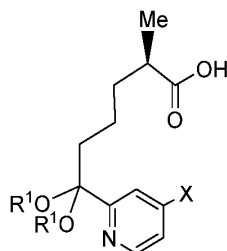
Compound 7
