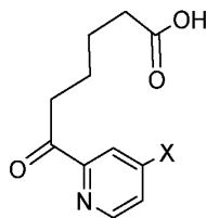
Compound 4;
