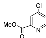
Compound 2a
