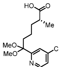
Compound 21
