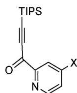
Compound 29
