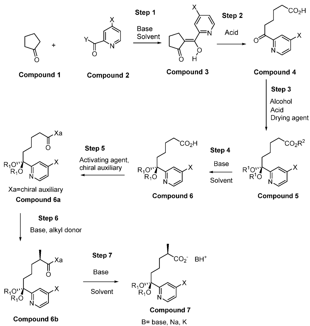
Scheme 1
