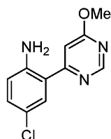
Compound 45;
