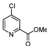
Compound 2a
