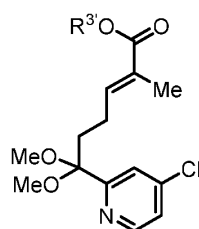
Compound 19
