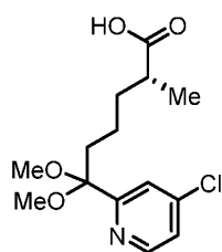
Compound 21
