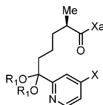
Compound 6b
