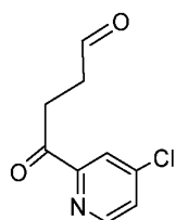
Compound 17
