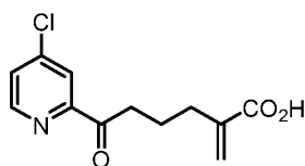
Compound 18b;
