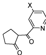
Compound 3b
