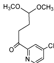
Compound 16
