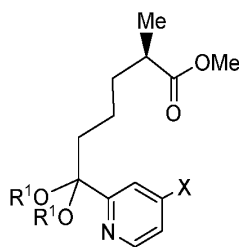
Compound 26
