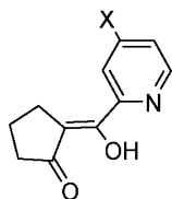
Compound 3a
