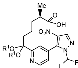
Compound 9;
