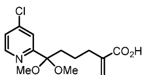
Compound 20b;
