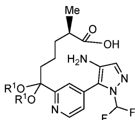
Compound 10;
