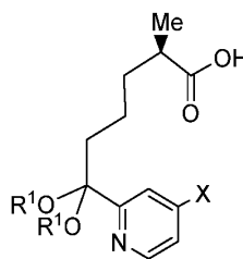
Compound 7
