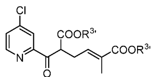
Compound 39;
