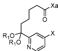
Compound 6a
