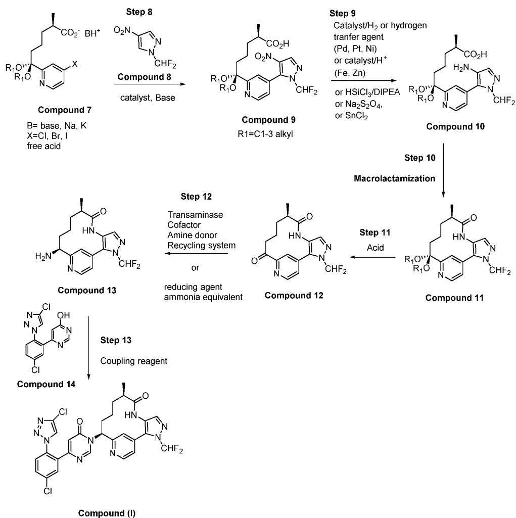
Scheme 2
