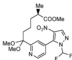
Compound 33.
