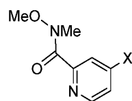
Compound 28
