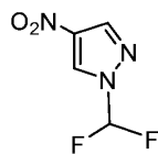
Compound 8
