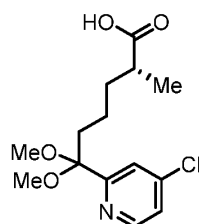
Compound 21.
