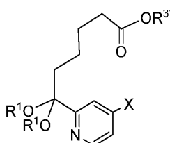
Compound 5
