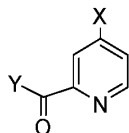
Compound 2
