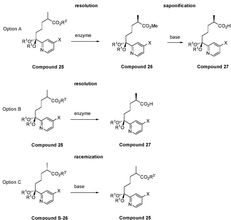
Scheme 7
