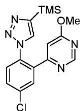
Compound 46;
