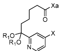
Compound 6a
