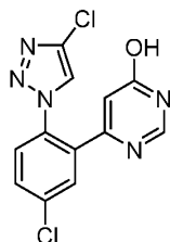
Compound 14
