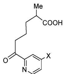
Compound 24
