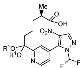
Compound 9
