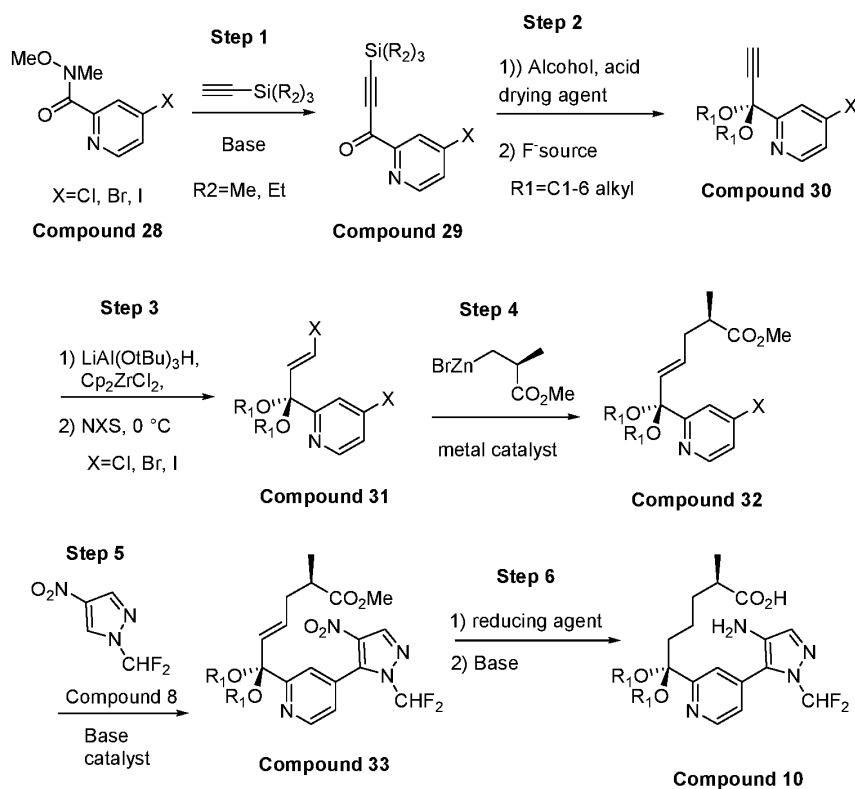
Scheme 8
