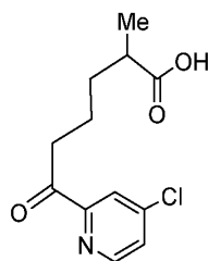
Compound 34.
