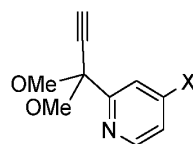
Compound 30
