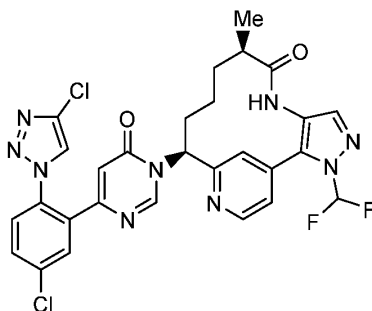
Compound (I).
