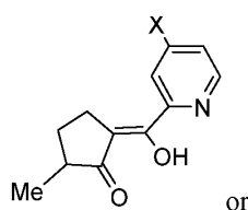
Compound 23a
