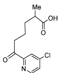
Compound 34.
