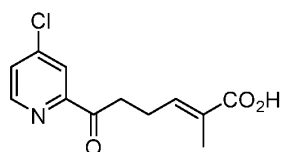
Compound 18a;
