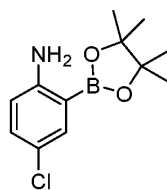
Compound 43
