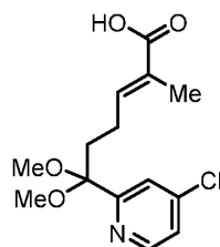
Compound 20
