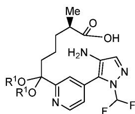
Compound 10
