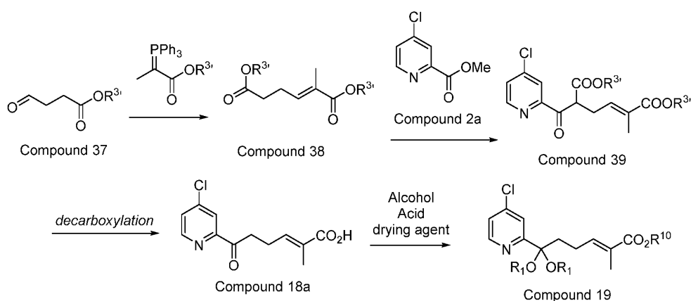
15 Scheme 4
