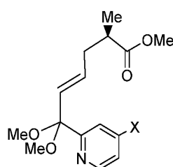
Compound 32
