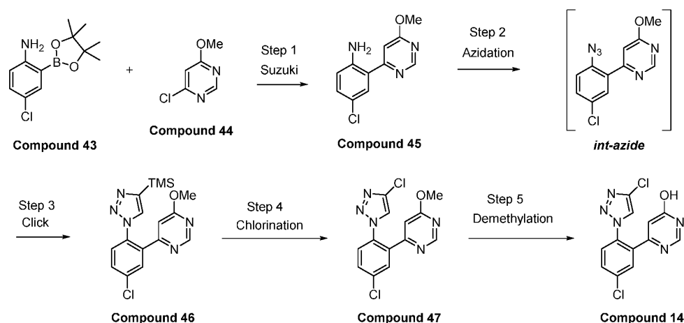
Scheme 9
