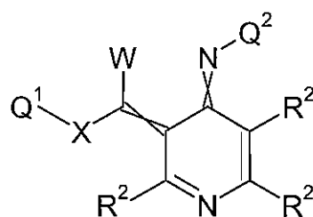
Formula 5.E.3
