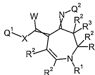
Formula 5.H.3
