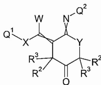
Formula 3.D.2
