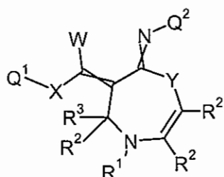
Formula 7.E.4
