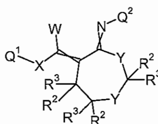
Formula 7.E.5
