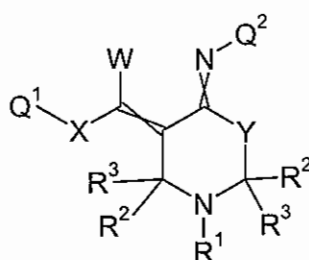
Formula 7.D.5
