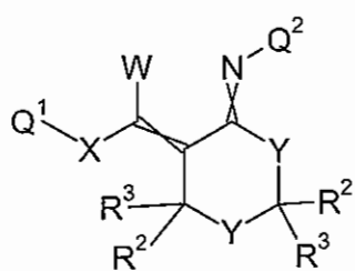
Formula 7.D.1
