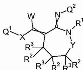
Formula 8.E.10
