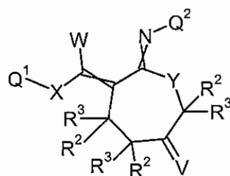
Formula 3.E.2
