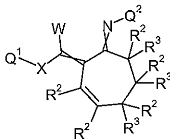
Formula 1.D.5
