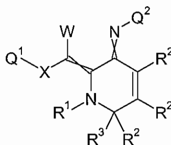
Formula 5.R.2
