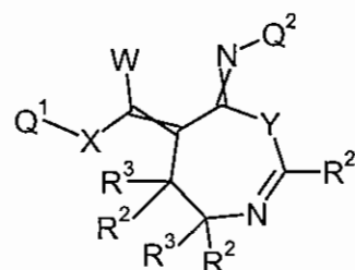
Formula 7.E.7
