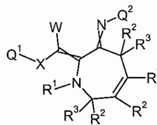
Formula 5.S.3
