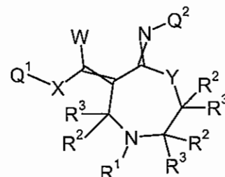
Formula 7.E.3
