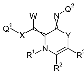
Formula 7.M.2
