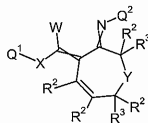
Formula 4.G.3
