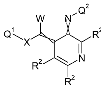
Formula 5.D.3
