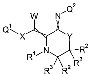
Formula 7.M.1
