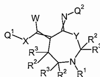
Formula 7.E.6
