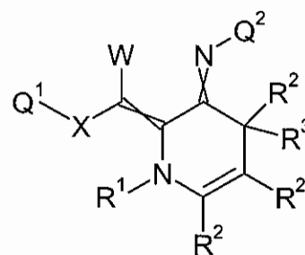
Formula 5.R.3
