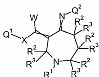
Formula 5.I.1
