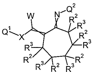
Formula 1.D.1
