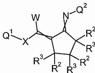
Formula 1.B.1
