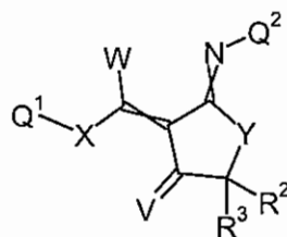
Formula 3.A.2
