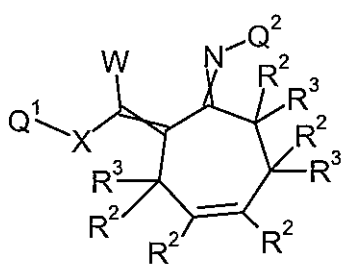
Formula 1.D.4
