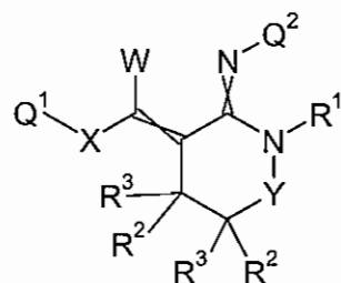
Formula 8.D.7
