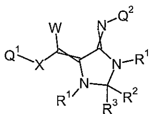
Formula 8.L.1
