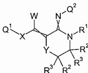
Formula 8.I.1
