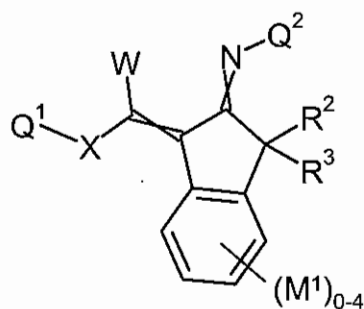
Formula 1.B.4
