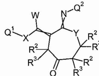
Formula 3.F.3
