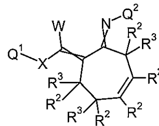
Formula 1.D.3
