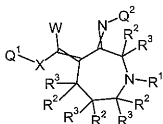
Formula 5.G.1
