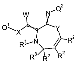
Formula 7.N.2
