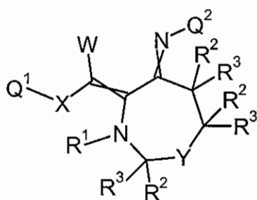
Formula 6.L.1
