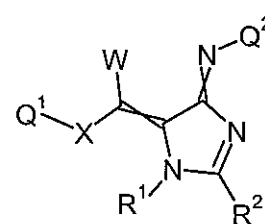
Formula 8.L.3
