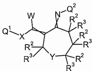
Formula 4.I.1
