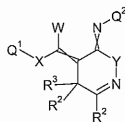
Formula 7.D.3
