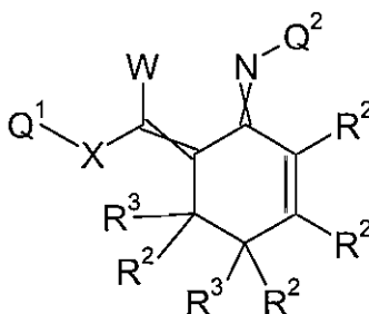
Formula 1.C.2
