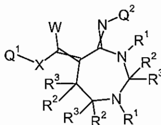
Formula 8.E.8
