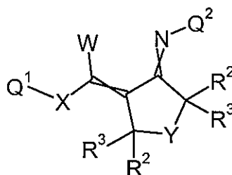
Formula 4.B.1
