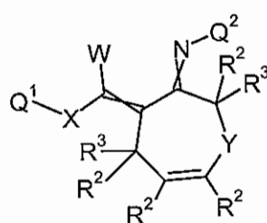
Formula 4.G.2
