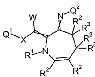
Formula 5.S.2
