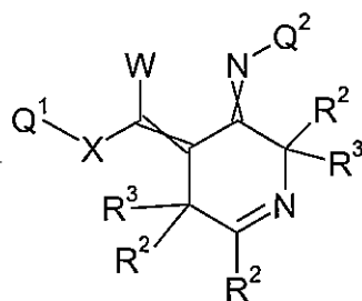
Formula 5.D.4
