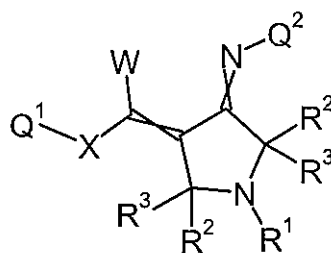
Formula 5.B.1
