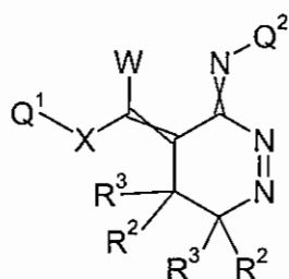
Formula 8.D.1
