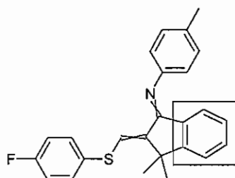
Example 1-21
