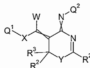
Formula 8.D.6
