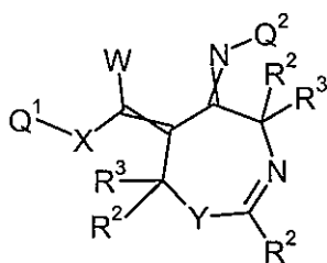
Formula 6.D.4
