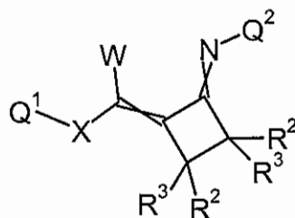
Formula 1.A.1
