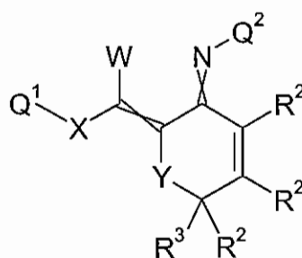
Formula 4.M.2
