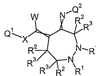
Formula 6.D.6
