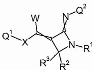
Formula 5.K.1
