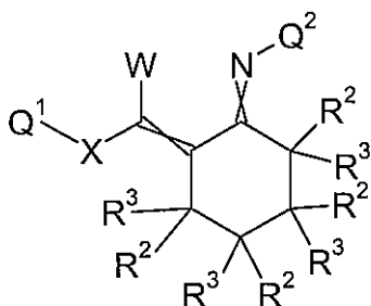
Formula 1.C.1
