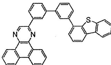
2mDBTBPDBq-II
