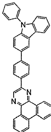
PCPDBq
