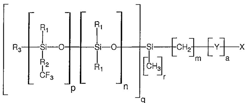
Formula I
