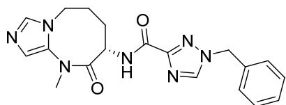
(S)-1-benzyl-N-(1-methyl-2-oxo-1,2,3,4,5,6-hexahydroimidazo[1,5-a][1,3]diazocin-3-yl)-1H-1,2,4-triazole-3-carboxamide
