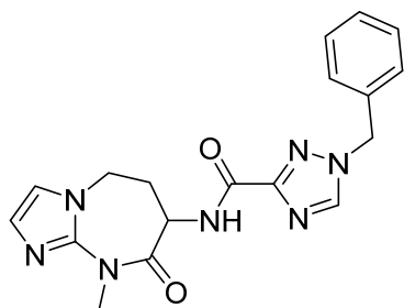
1-benzyl-N-(9-methyl-8-oxo-6,7,8,9-tetrahydro-5H-imidazo[1,2-a][1,3]diazepin-7-yl)-1H-1,2,4-triazole-3-carboxamide
