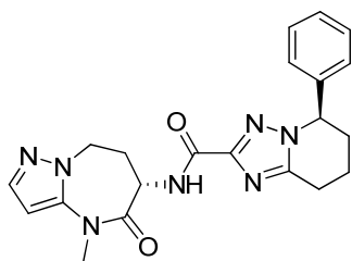
rac-(5R)-5-phenyl-N-[rac-(6S)-4-methyl-5-oxo-7,8-dihydro-6H-pyrazolo[1,5-a][1,3]diazepin-6-yl]-5,6,7,8-tetrahydro-[1,2,4]triazolo[1,5-a]pyridine-2-carboxamide
