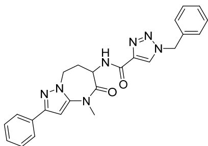
1-benzyl-N-(4-methyl-5-oxo-2-phenyl-5,6,7,8-tetrahydro-4H-pyrazolo[1,5-a][1,3]diazepin-6-yl)-1H-1,2,3-triazole-4-carboxamide
