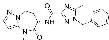
(S)-1-benzyl-5-methyl-N-(4-methyl-5-oxo-5,6,7,8-tetrahydro-4H-pyrazolo[1,5-a][1,3]diazepin-6-yl)-1H-1,2,4-triazole-3-carboxamide
