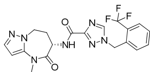
N-(6S)-4-methyl-5-oxo-7,8-dihydro-6H-pyrazolo[1,5-a][1,3]diazepin-6-yl-1-[[2-(trifluoromethyl)phenyl]methyl]-1,2,4-triazole-3-carboxamide
