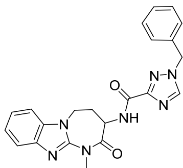
1-benzyl-N-(1-methyl-2-oxo-2,3,4,5-tetrahydro-1H-benzo[4,5]imidazo[1,2-a][1,3]diazepin-3-yl)-1H-1,2,4-triazole-3-carboxamide
