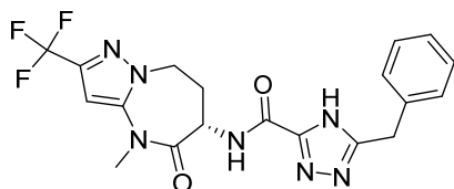
(S)-5-benzyl-N-(4-methyl-5-oxo-2-(trifluoromethyl)-5,6,7,8-tetrahydro-4H-pyrazolo[1,5-a][1,3]diazepin-6-yl)-4H-1,2,4-triazole-3-carboxamide
