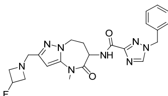
1-benzyl-N-[2-[(3-fluoroazetidin-1-yl)methyl]-4-methyl-5-oxo-7,8-dihydro-6H-pyrazolo[1,5-a][1,3]diazepin-6-yl]-1,2,4-triazole-3-carboxamide
