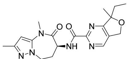
N-((S)-2,4-dimethyl-5-oxo-5,6,7,8-tetrahydro-4H-pyrazolo[1,5-a][1,3]diazepin-6-yl)-7-ethyl-7-methyl-5,7-dihydrofuro[3,4-d]pyrimidine-2-carboxamide
