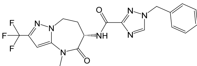
(S)-1-benzyl-N-(4-methyl-5-oxo-2-(trifluoromethyl)-5,6,7,8-tetrahydro-4H-pyrazolo[1,5-a][1,3]diazepin-6-yl)-1H-1,2,4-triazole-3-carboxamide,
