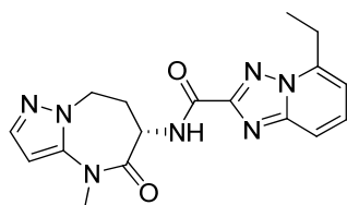
5-ethyl-N-[rac-(6S)-4-methyl-5-oxo-7,8-dihydro-6H-pyrazolo[1,5-a][1,3]diazepin-6-yl]-[1,2,4]triazolo[1,5-a]pyridine-2-carboxamide
