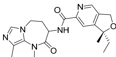
(1R)-N-(1,9-dimethyl-2-oxo-2,3,4,5-tetrahydro-1H-imidazo[1,5-a][1,3]diazepin-3-yl)-1-ethyl-1-methyl-1,3-dihydrofuro[3,4-c]pyridine-6-carboxamide
