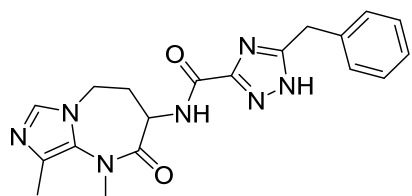
5-benzyl-N-(1,9-dimethyl-2-oxo-2,3,4,5-tetrahydro-1H-imidazo[1,5-a][1,3]diazepin-3-yl)-1H-1,2,4-triazole-3-carboxamide
