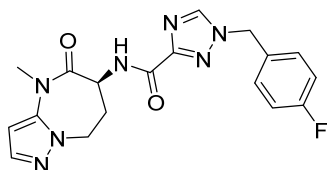
1-[(4-fluorophenyl)methyl]-N-[rac-(6S)-4-methyl-5-oxo-7,8-dihydro-6H-pyrazolo[1,5-a][1,3]diazepin-6-yl]-1,2,4-triazole-3-carboxamide
