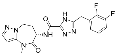
(S)-5-(2,3-difluorobenzyl)-N-(4-methyl-5-oxo-5,6,7,8-tetrahydro-4H-pyrazolo[1,5-a][1,3]diazepin-6-yl)-4H-1,2,4-triazole-3-carboxamide
