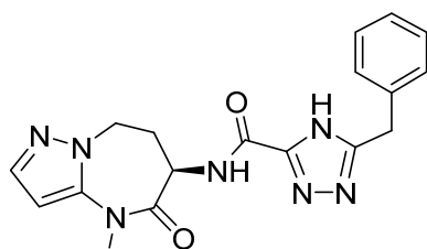
(R)-5-benzyl-N-(4-methyl-5-oxo-5,6,7,8-tetrahydro-4H-pyrazolo[1,5-a][1,3]diazepin-6-yl)-4H-1,2,4-triazole-3-carboxamide
