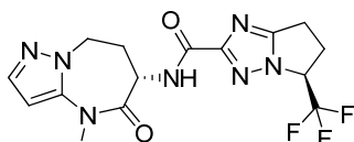
(5S)-N-[(6S)-4-methyl-5-oxo-7,8-dihydro-6H-pyrazolo[1,5-a][1,3]diazepin-6-yl]-5-(trifluoromethyl)-6,7-dihydro-5H-pyrrolo[1,2-b][1,2,4]triazole-2-carboxamide
