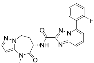
5-(2-fluorophenyl)-N-[(6S)-4-methyl-5-oxo-7,8-dihydro-6H-pyrazolo[1,5-a][1,3]diazepin-6-yl]-[1,2,4]triazolo[1,5-a]pyridine-2-carboxamide
