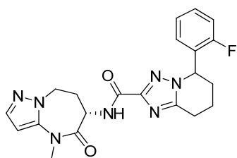
5-(2-fluorophenyl)-N-[rac-(6S)-4-methyl-5-oxo-7,8-dihydro-6H-pyrazolo[1,5-a][1,3]diazepin-6-yl]-5,6,7,8-tetrahydro-[1,2,4]triazolo[1,5-a]pyridine-2-carboxamide
