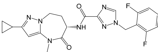
(S)-N-(2-cyclopropyl-4-methyl-5-oxo-5,6,7,8-tetrahydro-4H-pyrazolo[1,5-a][1,3]diazepin-6-yl)-1-(2,6-difluorobenzyl)-1H-1,2,4-triazole-3-carboxamide,
