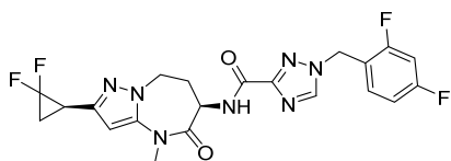
1-(2,4-difluorobenzyl)-N-((R)-2-((R)-2,2-difluorocyclopropyl)-4-methyl-5-oxo-5,6,7,8-tetrahydro-4H-pyrazolo[1,5-a][1,3]diazepin-6-yl)-1H-1,2,4-triazole-3-carboxamide
