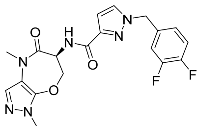
(S)-1-(3,4-difluorobenzyl)-N-(1,4-dimethyl-5-oxo-4,5,6,7-tetrahydro-1H-pyrazolo[3,4-b][1,4]oxazepin-6-yl)-1H-pyrazole-3-carboxamide
