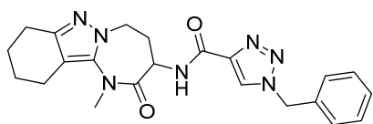
1-benzyl-N-(1-methyl-2-oxo-2,3,4,5,8,9,10,11-octahydro-1H-[1,3]diazepino[1,2-b]indazol-3-yl)-1H-1,2,3-triazole-4-carboxamide
