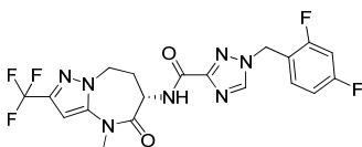
1-[(2,4-difluorophenyl)methyl]-N-(6S)-4-methyl-5-oxo-2-(trifluoromethyl)-7,8-dihydro-6H-pyrazolo[1,5-a][1,3]diazepin-6-yl-1,2,4-triazole-3-carboxamide
