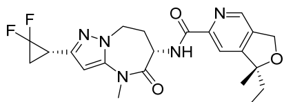
(R)-N-((S)-2-((S)-2,2-difluorocyclopropyl)-4-methyl-5-oxo-5,6,7,8-tetrahydro-4H-pyrazolo[1,5-a][1,3]diazepin-6-yl)-1-ethyl-1-methyl-1,3-dihydrofuro[3,4-c]pyridine-6-carboxamide
