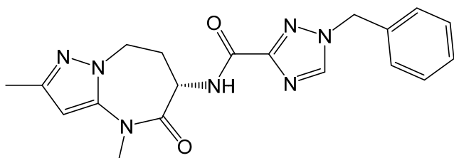
(S)-1-benzyl-N-(2,4-dimethyl-5-oxo-5,6,7,8-tetrahydro-4H-pyrazolo[1,5-a][1,3]diazepin-6-yl)-1H-1,2,4-triazole-3-carboxamide,
