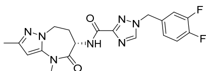
(S)-1-(3,4-difluorobenzyl)-N-(2,4-dimethyl-5-oxo-5,6,7,8-tetrahydro-4H-pyrazolo[1,5-a][1,3]diazepin-6-yl)-1H-1,2,4-triazole-3-carboxamide
