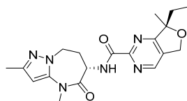
rac-(7R)-7-ethyl-7-methyl-N-[rac-(6S)-2,4-dimethyl-5-oxo-7,8-dihydro-6H-pyrazolo[1,5-a][1,3]diazepin-6-yl]-5H-furo[3,4-d]pyrimidine-2-carboxamide
