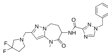
1-benzyl-N-[2-[(3,3-difluoropyrrolidin-1-yl)methyl]-4-methyl-5-oxo-7,8-dihydro-6H-pyrazolo[1,5-a][1,3]diazepin-6-yl]-1,2,4-triazole-3-carboxamide
