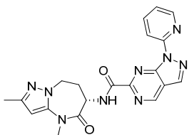
(5R)-5-phenyl-N-[(6S)-4-methyl-5-oxo-7,8-dihydro-6H-pyrazolo[1,5-a][1,3]diazepin-6-yl]-6,7-dihydro-5H-pyrrolo[1,2-b][1,2,4]triazole-2-carboxamide
