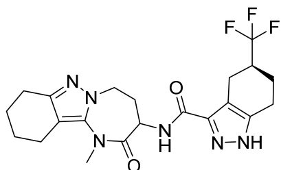
(5S)-N-(1-methyl-2-oxo-2,3,4,5,8,9,10,11-octahydro-1H-[1,3]diazepino[1,2-b]indazol-3-yl)-5-(trifluoromethyl)-4,5,6,7-tetrahydro-1H-indazole-3-carboxamide
