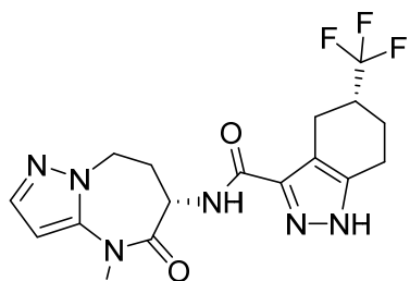
(R)-N-((S)-4-methyl-5-oxo-5,6,7,8-tetrahydro-4H-pyrazolo[1,5-a][1,3]diazepin-6-yl)-5-(trifluoromethyl)-4,5,6,7-tetrahydro-1H-indazole-3-carboxamide
