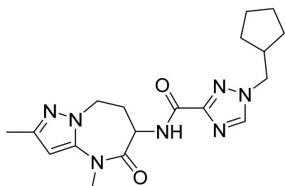
1-(cyclopentylmethyl)-N-(2,4-dimethyl-5-oxo-5,6,7,8-tetrahydro-4H-pyrazolo[1,5-a][1,3]diazepin-6-yl)-1H-1,2,4-triazole-3-carboxamide
