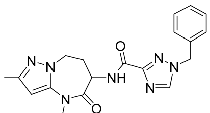
1-benzyl-N-(2,4-dimethyl-5-oxo-5,6,7,8-tetrahydro-4H-pyrazolo[1,5-a][1,3]diazepin-6-yl)-1H-1,2,4-triazole-3-carboxamide
