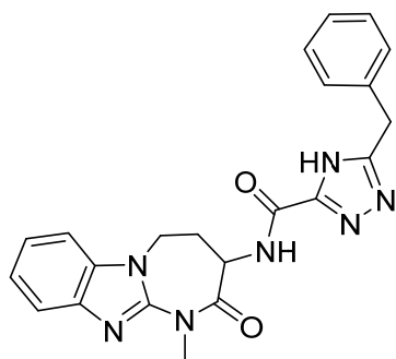
5-benzyl-N-(1-methyl-2-oxo-2,3,4,5-tetrahydro-1H-benzo[4,5]imidazo[1,2-a][1,3]diazepin-3-yl)-4H-1,2,4-triazole-3-carboxamide
