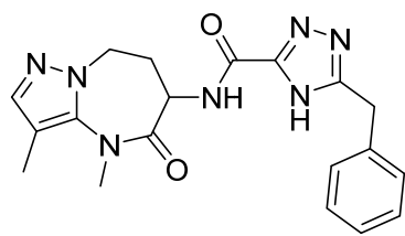
5-benzyl-N-(3,4-dimethyl-5-oxo-5,6,7,8-tetrahydro-4H-pyrazolo[1,5-a][1,3]diazepin-6-yl)-4H-1,2,4-triazole-3-carboxamide
