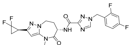
1-(2,4-difluorobenzyl)-N-((S)-2-((R)-2,2-difluorocyclopropyl)-4-methyl-5-oxo-5,6,7,8-tetrahydro-4H-pyrazolo[1,5-a][1,3]diazepin-6-yl)-1H-1,2,4-triazole-3-carboxamide
