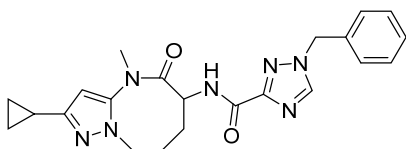
1-benzyl-N-(2-cyclopropyl-4-methyl-5-oxo-4,5,6,7,8,9-hexahydropyrazolo[1,5-a][1,3]diazocin-6-yl)-1H-1,2,4-triazole-3-carboxamide
