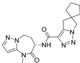
(S)-N-(4-methyl-5-oxo-5,6,7,8-tetrahydro-4H-pyrazolo[1,5-a][1,3]diazepin-6-yl)-4'H,6'H-spiro[cyclopentane-1,5'-pyrrolo[1,2-c][1,2,3]triazole]-3'-carboxamide
