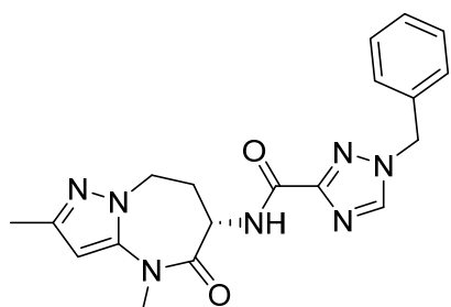
(S)-1-benzyl-N-(2,4-dimethyl-5-oxo-5,6,7,8-tetrahydro-4H-pyrazolo[1,5-a][1,3]diazepin-6-yl)-1H-1,2,4-triazole-3-carboxamide
