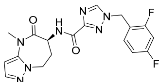
1-[(2,4-difluorophenyl)methyl]-N-[rac-(6S)-4-methyl-5-oxo-7,8-dihydro-6H-pyrazolo[1,5-a][1,3]diazepin-6-yl]-1,2,4-triazole-3-carboxamide
