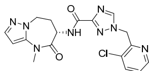
1-[(3-chloro-2-pyridyl)methyl]-N-(6S)-4-methyl-5-oxo-7,8-dihydro-6H-pyrazolo[1,5-a][1,3]diazepin-6-yl-1,2,4-triazole-3-carboxamide
