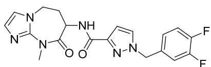
1-(3,4-difluorobenzyl)-N-(9-methyl-8-oxo-6,7,8,9-tetrahydro-5H-imidazo[1,2-a][1,3]diazepin-7-yl)-1H-pyrazole-3-carboxamide
