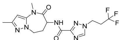
N-(2,4-dimethyl-5-oxo-5,6,7,8-tetrahydro-4H-pyrazolo[1,5-a][1,3]diazepin-6-yl)-1-(3,3,3-trifluoropropyl)-1H-1,2,4-triazole-3-carboxamide
