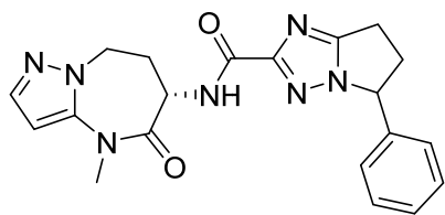
N-((S)-4-methyl-5-oxo-5,6,7,8-tetrahydro-4H-pyrazolo[1,5-a][1,3]diazepin-6-yl)-5-phenyl-6,7-dihydro-5H-pyrrolo[1,2-b][1,2,4]triazole-2-carboxamide
