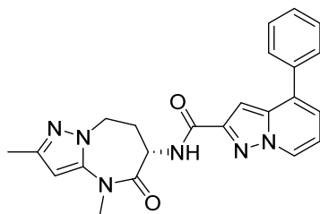
(S)-N-(2,4-dimethyl-5-oxo-5,6,7,8-tetrahydro-4H-pyrazolo[1,5-a][1,3]diazepin-6-yl)-4-phenylpyrazolo[1,5-a]pyridine-2-carboxamide
