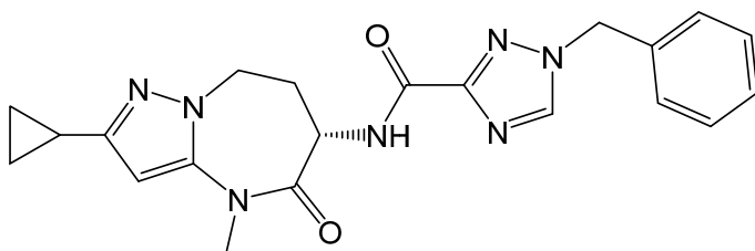
(S)-1-benzyl-N-(2-cyclopropyl-4-methyl-5-oxo-5,6,7,8-tetrahydro-4H-pyrazolo[1,5-a][1,3]diazepin-6-yl)-1H-1,2,4-triazole-3-carboxamide.
