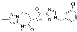
1-[(3-chlorophenyl)methyl]-N-(6S)-2,4-dimethyl-5-oxo-7,8-dihydro-6H-pyrazolo[1,5-a][1,3]diazepin-6-yl-1,2,4-triazole-3-carboxamide
