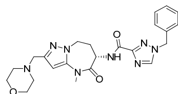
1-benzyl-N-[(6S)-4-methyl-2-(morpholinomethyl)-5-oxo-7,8-dihydro-6H-pyrazolo[1,5-a][1,3]diazepin-6-yl]-1,2,4-triazole-3-carboxamide
