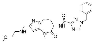
1-benzyl-N-[2-[(2-methoxyethylamino)methyl]-4-methyl-5-oxo-7,8-dihydro-6H-pyrazolo[1,5-a][1,3]diazepin-6-yl]-1,2,4-triazole-3-carboxamide
