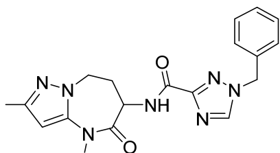
1-benzyl-N-(2,4-dimethyl-5-oxo-5,6,7,8-tetrahydro-4H-pyrazolo[1,5-a][1,3]diazepin-6-yl)-1H-1,2,4-triazole-3-carboxamide
