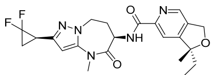
(R)-N-((R)-2-((R)-2,2-difluorocyclopropyl)-4-methyl-5-oxo-5,6,7,8-tetrahydro-4H-pyrazolo[1,5-a][1,3]diazepin-6-yl)-1-ethyl-1-methyl-1,3-dihydrofuro[3,4-c]pyridine-6-carboxamide
