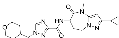
N-(2-cyclopropyl-4-methyl-5-oxo-5,6,7,8-tetrahydro-4H-pyrazolo[1,5-a][1,3]diazepin-6-yl)-1-((tetrahydro-2H-pyran-4-yl)methyl)-1H-1,2,4-triazole-3-carboxamide
