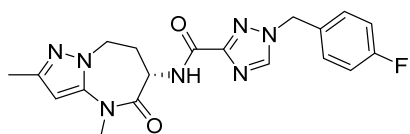
(S)-N-(2,4-dimethyl-5-oxo-5,6,7,8-tetrahydro-4H-pyrazolo[1,5-a][1,3]diazepin-6-yl)-1-(4-fluorobenzyl)-1H-1,2,4-triazole-3-carboxamide
