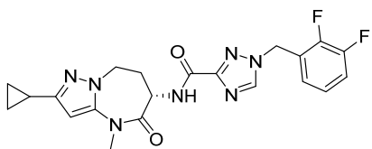
(S)-N-(2-cyclopropyl-4-methyl-5-oxo-5,6,7,8-tetrahydro-4H-pyrazolo[1,5-a][1,3]diazepin-6-yl)-1-(2,3-difluorobenzyl)-1H-1,2,4-triazole-3-carboxamide
