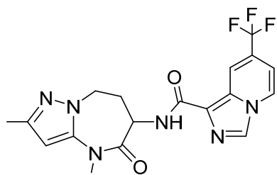
N-(2,4-dimethyl-5-oxo-5,6,7,8-tetrahydro-4H-pyrazolo[1,5-a][1,3]diazepin-6-yl)-7-(trifluoromethyl)imidazo[1,5-a]pyridine-1-carboxamide
