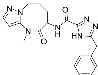
5-benzyl-N-(4-methyl-5-oxo-4,5,6,7,8,9-hexahydropyrazolo[1,5-a][1,3]diazocin-6-yl)-4H-1,2,4-triazole-3-carboxamide
