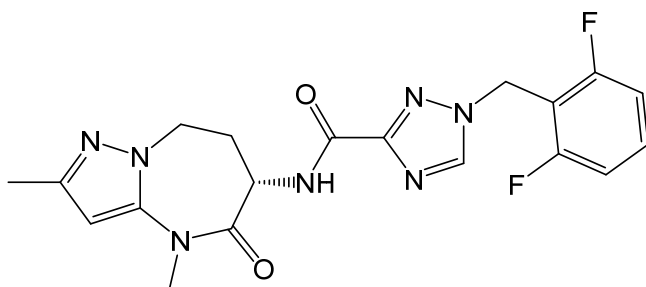
(S)-1-(2,6-difluorobenzyl)-N-(2,4-dimethyl-5-oxo-5,6,7,8-tetrahydro-4H-pyrazolo[1,5-a][1,3]diazepin-6-yl)-1H-1,2,4-triazole-3-carboxamide,
