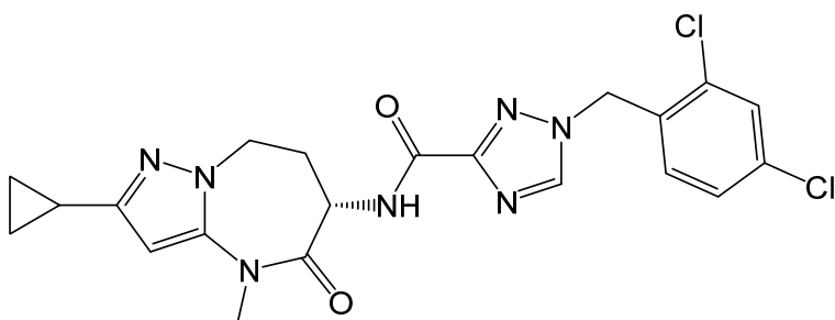
(S)-N-(2-cyclopropyl-4-methyl-5-oxo-5,6,7,8-tetrahydro-4H-pyrazolo[1,5-a][1,3]diazepin-6-yl)-1-(2,3-difluorobenzyl)-1H-1,2,4-triazole-3-carboxamide,
