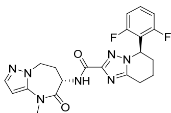
rac-(5R)-5-(2,6-difluorophenyl)-N-[rac-(6S)-4-methyl-5-oxo-7,8-dihydro-6H-pyrazolo[1,5-a][1,3]diazepin-6-yl]-5,6,7,8-tetrahydro-[1,2,4]triazolo[1,5-a]pyridine-2-carboxamide
