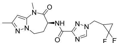
1-((2,2-difluorocyclopropyl)methyl)-N-((S)-2,4-dimethyl-5-oxo-5,6,7,8-tetrahydro-4H-pyrazolo[1,5-a][1,3]diazepin-6-yl)-1H-1,2,4-triazole-3-carboxamide
