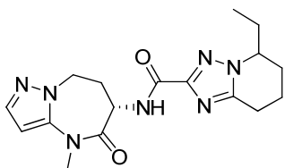
5-ethyl-N-[(6S)-4-methyl-5-oxo-7,8-dihydro-6H-pyrazolo[1,5-a][1,3]diazepin-6-yl]-5,6,7,8-tetrahydro-[1,2,4]triazolo[1,5-a]pyridine-2-
