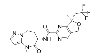
rac-(7S)-7-methyl-N-[rac-(6S)-2,4-dimethyl-5-oxo-7,8-dihydro-6H-pyrazolo[1,5-a][1,3]diazepin-6-yl]-7-(2,2,2-trifluoroethyl)-5H-furo[3,4-d]pyrimidine-2-carboxamide
