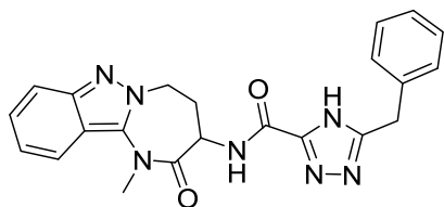
5-benzyl-N-(1-methyl-2-oxo-2,3,4,5-tetrahydro-1H-[1,3]diazepino[1,2-b]indazol-3-yl)-4H-1,2,4-triazole-3-carboxamide
