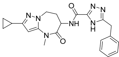
5-benzyl-N-(2-cyclopropyl-4-methyl-5-oxo-5,6,7,8-tetrahydro-4H-pyrazolo[1,5-a][1,3]diazepin-6-yl)-4H-1,2,4-triazole-3-carboxamide
