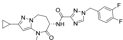
(S)-N-(2-cyclopropyl-4-methyl-5-oxo-5,6,7,8-tetrahydro-4H-pyrazolo[1,5-a][1,3]diazepin-6-yl)-1-(3,4-difluorobenzyl)-1H-1,2,4-triazole-3-carboxamide
