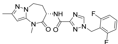
(S)-1-(2,6-difluorobenzyl)-N-(2,4-dimethyl-5-oxo-5,6,7,8-tetrahydro-4H-pyrazolo[1,5-a][1,3]diazepin-6-yl)-1H-1,2,4-triazole-3-carboxamide
