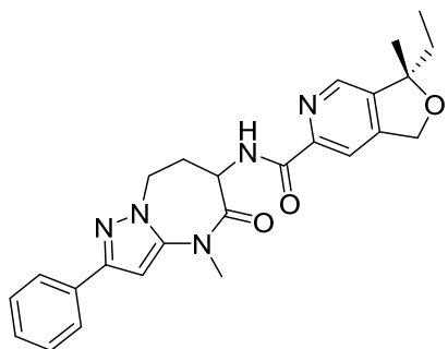
(3R)-3-ethyl-3-methyl-N-(4-methyl-5-oxo-2-phenyl-5,6,7,8-tetrahydro-4H-pyrazolo[1,5-a][1,3]diazepin-6-yl)-1,3-dihydrofuro[3,4-c]pyridine-6-carboxamide
