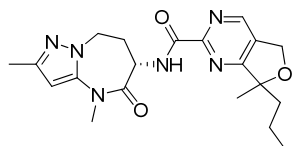
7-methyl-7-propyl-N-[(6S)-2,4-dimethyl-5-oxo-7,8-dihydro-6H-pyrazolo[1,5-a][1,3]diazepin-6-yl]-5H-furo[3,4-d]pyrimidine-2-carboxamide
