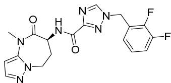
1-[(2,3-difluorophenyl)methyl]-N-[rac-(6S)-4-methyl-5-oxo-7,8-dihydro-6H-pyrazolo[1,5-a][1,3]diazepin-6-yl]-1,2,4-triazole-3-carboxamide
