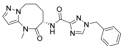
(S)-1-benzyl-N-(4-methyl-5-oxo-4,5,6,7,8,9-hexahydropyrazolo[1,5-a][1,3]diazocin-6-yl)-1H-1,2,4-triazole-3-carboxamide
