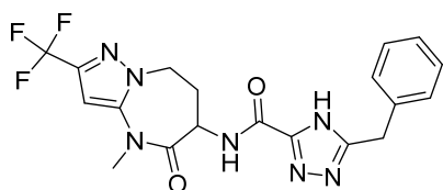
5-benzyl-N-(4-methyl-5-oxo-2-(trifluoromethyl)-5,6,7,8-tetrahydro-4H-pyrazolo[1,5-a][1,3]diazepin-6-yl)-4H-1,2,4-triazole-3-carboxamide
