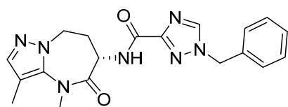
(S)-1-benzyl-N-(3,4-dimethyl-5-oxo-5,6,7,8-tetrahydro-4H-pyrazolo[1,5-a][1,3]diazepin-6-yl)-1H-1,2,4-triazole-3-carboxamide
