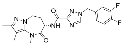
(S)-1-(3,4-difluorobenzyl)-N-(2,3,4-trimethyl-5-oxo-5,6,7,8-tetrahydro-4H-pyrazolo[1,5-a][1,3]diazepin-6-yl)-1H-1,2,4-triazole-3-carboxamide
