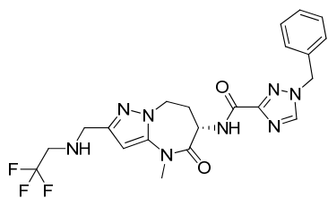
1-benzyl-N-[(6S)-4-methyl-5-oxo-2-[(2,2,2-trifluoroethylamino)methyl]-7,8-dihydro-6H-pyrazolo[1,5-a][1,3]diazepin-6-yl]-1,2,4-triazole-3-carboxamide
