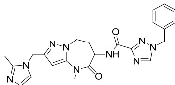
1-benzyl-N-[4-methyl-2-[(2-methylimidazol-1-yl)methyl]-5-oxo-7,8-dihydro-6H-pyrazolo[1,5-a][1,3]diazepin-6-yl]-1,2,4-triazole-3-carboxamide
