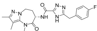
(S)-5-(4-fluorobenzyl)-N-(2,3,4-trimethyl-5-oxo-5,6,7,8-tetrahydro-4H-pyrazolo[1,5-a][1,3]diazepin-6-yl)-4H-1,2,4-triazole-3-carboxamide
