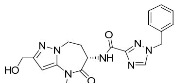
1-benzyl-N-[(6S)-2-(hydroxymethyl)-4-methyl-5-oxo-7,8-dihydro-6H-pyrazolo[1,5-a][1,3]diazepin-6-yl]-1,2,4-triazole-3-carboxamide
