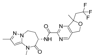
7-methyl-N-[(6S)-2,4-dimethyl-5-oxo-7,8-dihydro-6H-pyrazolo[1,5-a][1,3]diazepin-6-yl]-7-(2,2,2-trifluoroethyl)-5H-furo[3,4-d]pyrimidine-2-carboxamide
