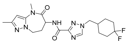
1-((4,4-difluorocyclohexyl)methyl)-N-(2,4-dimethyl-5-oxo-5,6,7,8-tetrahydro-4H-pyrazolo[1,5-a][1,3]diazepin-6-yl)-1H-1,2,4-triazole-3-carboxamide
