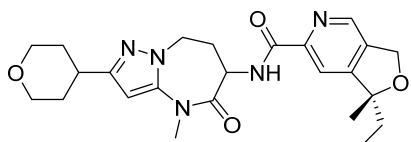
(1R)-1-ethyl-1-methyl-N-(4-methyl-5-oxo-2-(tetrahydro-2H-pyran-4-yl)-5,6,7,8-tetrahydro-4H-pyrazolo[1,5-a][1,3]diazepin-6-yl)-1,3-dihydrofuro[3,4-c]pyridine-6-carboxamide
