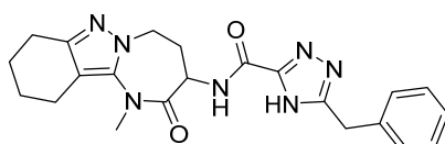
5-benzyl-N-(1-methyl-2-oxo-2,3,4,5,8,9,10,11-octahydro-1H-[1,3]diazepino[1,2-b]indazol-3-yl)-4H-1,2,4-triazole-3-carboxamide
