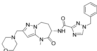
1-benzyl-N-[(6S)-4-methyl-2-(morpholinomethyl)-5-oxo-7,8-dihydro-6H-pyrazolo[1,5-a][1,3]diazepin-6-yl]-1,2,4-triazole-3-carboxamide
