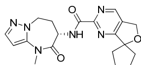
N-[rac-(6S)-4-methyl-5-oxo-7,8-dihydro-6H-pyrazolo[1,5-a][1,3]diazepin-6-yl]spiro[5H-furo[3,4-d]pyrimidine-7,1'-cyclopentane]-2-carboxamide
