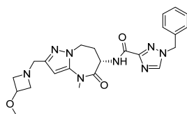
(S)-1-benzyl-N-(2-((3-methoxyazetidin-1-yl)methyl)-4-methyl-5-oxo-5,6,7,8-tetrahydro-4H-pyrazolo[1,5-a][1,3]diazepin-6-yl)-1H-1,2,4-triazole-3-carboxamide
