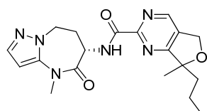
7-methyl-7-propyl-N-[(6S)-4-methyl-5-oxo-7,8-dihydro-6H-pyrazolo[1,5-a][1,3]diazepin-6-yl]-5H-furo[3,4-d]pyrimidine-2-carboxamide
