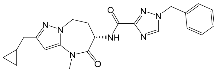
(S)-1-benzyl-N-(2-(cyclopropylmethyl)-4-methyl-5-oxo-5,6,7,8-tetrahydro-4H-pyrazolo[1,5-a][1,3]diazepin-6-yl)-1H-1,2,4-triazole-3-carboxamide,
