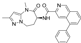
5-phenyl-N-[(6S)-2,4-dimethyl-5-oxo-7,8-dihydro-6H-pyrazolo[1,5-a][1,3]diazepin-6-yl]isoquinoline-3-carboxamide
