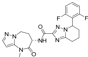
5-(2,6-difluorophenyl)-N-[rac-(6S)-4-methyl-5-oxo-7,8-dihydro-6H-pyrazolo[1,5-a][1,3]diazepin-6-yl]-5,6,7,8-tetrahydro-[1,2,4]triazolo[1,5-a]pyridine-2-carboxamide
