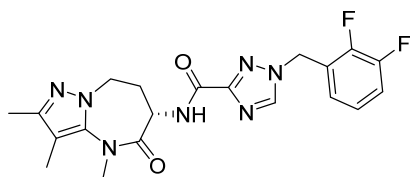
(S)-1-(2,3-difluorobenzyl)-N-(2,3,4-trimethyl-5-oxo-5,6,7,8-tetrahydro-4H-pyrazolo[1,5-a][1,3]diazepin-6-yl)-1H-1,2,4-triazole-3-carboxamide
