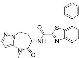
7-phenyl-N-[rac-(6S)-4-methyl-5-oxo-7,8-dihydro-6H-pyrazolo[1,5-a][1,3]diazepin-6-yl]-1,3-benzothiazole-2-carboxamide
