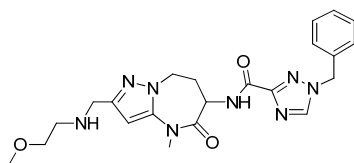
1-benzyl-N-[2-[(2-methoxyethylamino)methyl]-4-methyl-5-oxo-7,8-dihydro-6H-pyrazolo[1,5-a][1,3]diazepin-6-yl]-1,2,4-triazole-3-carboxamide
