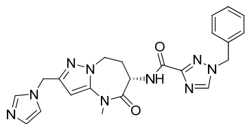
(S)-1-benzyl-N-[2-(imidazol-1-ylmethyl)-4-methyl-5-oxo-7,8-dihydro-6H-pyrazolo[1,5-a][1,3]diazepin-6-yl]-1,2,4-triazole-3-carboxamide
