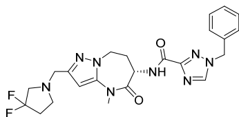
(S)-1-benzyl-N-(2-((3,3-difluoropyrrolidin-1-yl)methyl)-4-methyl-5-oxo-5,6,7,8-tetrahydro-4H-pyrazolo[1,5-a][1,3]diazepin-6-yl)-1H-1,2,4-triazole-3-carboxamide
