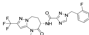
1-[(2-fluorophenyl)methyl]-N-(6S)-4-methyl-5-oxo-2-(trifluoromethyl)-7,8-dihydro-6H-pyrazolo[1,5-a][1,3]diazepin-6-yl-1,2,4-triazole-3-carboxamide
