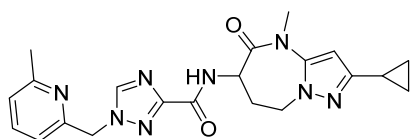
N-(2-cyclopropyl-4-methyl-5-oxo-5,6,7,8-tetrahydro-4H-pyrazolo[1,5-a][1,3]diazepin-6-yl)-1-((6-methylpyridin-2-yl)methyl)-1H-1,2,4-triazole-3-carboxamide
