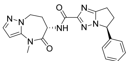
(S)-N-((S)-4-methyl-5-oxo-5,6,7,8-tetrahydro-4H-pyrazolo[1,5-a][1,3]diazepin-6-yl)-5-phenyl-6,7-dihydro-5H-pyrrolo[1,2-b][1,2,4]triazole-2-carboxamide
