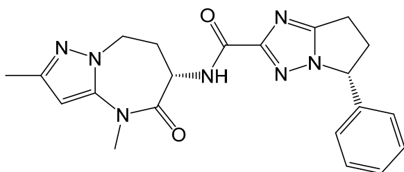
(5R)-5-phenyl-N-[(6S)-2,4-dimethyl-5-oxo-7,8-dihydro-6H-pyrazolo[1,5-a][1,3]diazepin-6-yl]-6,7-dihydro-5H-pyrrolo[1,2-b][1,2,4]triazole-2-carboxamide, and
