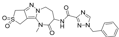
1-benzyl-N-(1-methyl-9,9-dioxido-2-oxo-1,2,3,4,5,10-hexahydro-8H-thieno[3',4':3,4]pyrazolo[1,5-a][1,3]diazepin-3-yl)-1H-1,2,4-triazole-3-carboxamide
