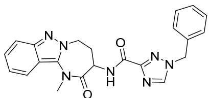
1-benzyl-N-(1-methyl-2-oxo-2,3,4,5-tetrahydro-1H-[1,3]diazepino[1,2-b]indazol-3-yl)-1H-1,2,4-triazole-3-carboxamide
