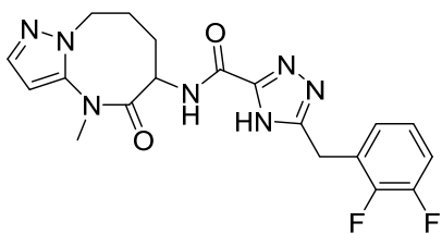
5-(2,3-difluorobenzyl)-N-(4-methyl-5-oxo-4,5,6,7,8,9-hexahydropyrazolo[1,5-a][1,3]diazocin-6-yl)-4H-1,2,4-triazole-3-carboxamide
