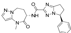
rac-(5S)-5-phenyl-N-[rac-(6S)-4-methyl-5-oxo-7,8-dihydro-6H-pyrazolo[1,5-a][1,3]diazepin-6-yl]-6,7-dihydro-5H-pyrrolo[1,2-b][1,2,4]triazole-2-carboxamide
