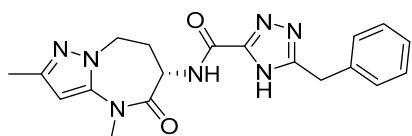
(S)-5-benzyl-N-(2,4-dimethyl-5-oxo-5,6,7,8-tetrahydro-4H-pyrazolo[1,5-a][1,3]diazepin-6-yl)-4H-1,2,4-triazole-3-carboxamide
