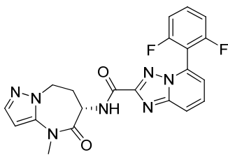
5-(2,6-difluorophenyl)-N-[(6S)-4-methyl-5-oxo-7,8-dihydro-6H-pyrazolo[1,5-a][1,3]diazepin-6-yl]-[1,2,4]triazolo[1,5-a]pyridine-2-carboxamide
