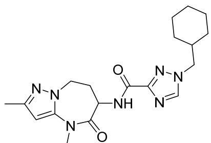
1-(cyclohexylmethyl)-N-(2,4-dimethyl-5-oxo-5,6,7,8-tetrahydro-4H-pyrazolo[1,5-a][1,3]diazepin-6-yl)-1H-1,2,4-triazole-3-carboxamide
