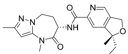
(R)-N-((S)-2,4-dimethyl-5-oxo-5,6,7,8-tetrahydro-4H-pyrazolo[1,5-a][1,3]diazepin-6-yl)-1-ethyl-1-methyl-1,3-dihydrofuro[3,4-c]pyridine-6-carboxamide
