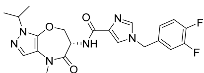
(S)-1-(3,4-difluorobenzyl)-N-(1-isopropyl-4-methyl-5-oxo-4,5,6,7-tetrahydro-1H-pyrazolo[3,4-b][1,4]oxazepin-6-yl)-1H-imidazole-4-carboxamide
