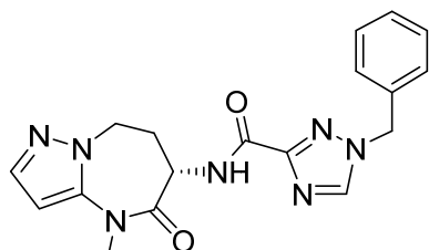
(S)-1-benzyl-N-(4-methyl-5-oxo-5,6,7,8-tetrahydro-4H-pyrazolo[1,5-a][1,3]diazepin-6-yl)-1H-1,2,4-triazole-3-carboxamide
