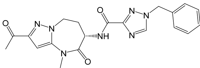
(S)-N-(2-acetyl-4-methyl-5-oxo-5,6,7,8-tetrahydro-4H-pyrazolo[1,5-a][1,3]diazepin-6-yl)-1-benzyl-1H-1,2,4-triazole-3-carboxamide,
