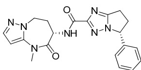
(5R)-N-[(6S)-4-methyl-5-oxo-7,8-dihydro-6H-pyrazolo[1,5-a][1,3]diazepin-6-yl]-5-phenyl-6,7-dihydro-5H-pyrrolo[1,2-b][1,2,4]triazole-2-carboxamide
