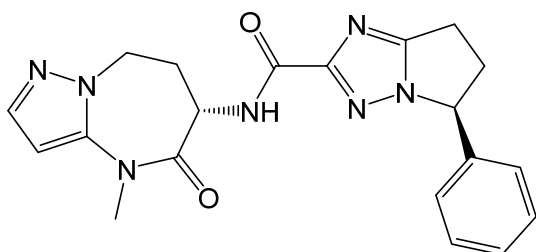
(S)-N-((S)-4-methyl-5-oxo-5,6,7,8-tetrahydro-4H-pyrazolo[1,5-a][1,3]diazepin-6-yl)-5-phenyl-6,7-dihydro-5H-pyrrolo[1,2-b][1,2,4]triazole-2-carboxamide,
