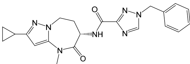
(S)-1-benzyl-N-(2-cyclopropyl-4-methyl-5-oxo-5,6,7,8-tetrahydro-4H-pyrazolo[1,5-a][1,3]diazepin-6-yl)-1H-1,2,4-triazole-3-carboxamide,
