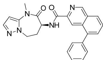
5-phenyl-N-[(6S)-4-methyl-5-oxo-7,8-dihydro-6H-pyrazolo[1,5-a][1,3]diazepin-6-yl]isoquinoline-3-carboxamide
