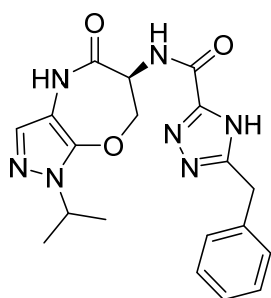
(S)-5-benzyl-N-(1-isopropyl-5-oxo-4,5,6,7-tetrahydro-1H-pyrazolo[3,4-b][1,4]oxazepin-6-yl)-4H-1,2,4-triazole-3-carboxamide
