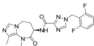
1-[(2,6-difluorophenyl)methyl]-N-(3R)-1,9-dimethyl-2-oxo-4,5-dihydro-3H-imidazo[1,5-a][1,3]diazepin-3-yl-1,2,4-triazole-3-carboxamide
