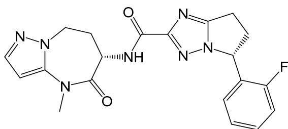
(R)-5-(2-fluorophenyl)-N-((S)-4-methyl-5-oxo-5,6,7,8-tetrahydro-4H-pyrazolo[1,5-a][1,3]diazepin-6-yl)-6,7-dihydro-5H-pyrrolo[1,2-b][1,2,4]triazole-2-carboxamide,
