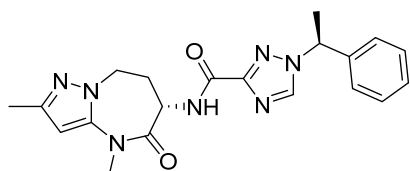
N-((S)-2,4-dimethyl-5-oxo-5,6,7,8-tetrahydro-4H-pyrazolo[1,5-a][1,3]diazepin-6-yl)-1-((S)-1-phenylethyl)-1H-1,2,4-triazole-3-carboxamide
