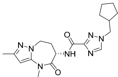
(S)-1-(cyclopentylmethyl)-N-(2,4-dimethyl-5-oxo-5,6,7,8-tetrahydro-4H-pyrazolo[1,5-a][1,3]diazepin-6-yl)-1H-1,2,4-triazole-3-carboxamide
