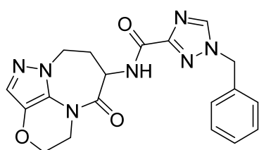
1-benzyl-N-(6-oxo-4,5,6,7,8,9-hexahydro-3-oxa-1,5a,9a-triazabenzocd]azulen-7-yl)-1H-1,2,4-triazole-3-carboxamide
