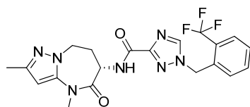
N-(6S)-2,4-dimethyl-5-oxo-7,8-dihydro-6H-pyrazolo[1,5-a][1,3]diazepin-6-yl-1-[[2-(trifluoromethyl)phenyl]methyl]-1,2,4-
