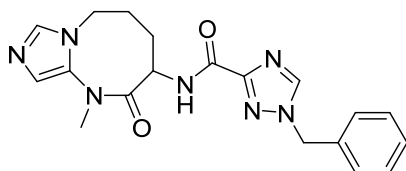
1-benzyl-N-(1-methyl-2-oxo-1,2,3,4,5,6-hexahydroimidazo[1,5-a][1,3]diazocin-3-yl)-1H-1,2,4-triazole-3-carboxamide
