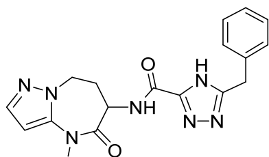
5-benzyl-N-(4-methyl-5-oxo-5,6,7,8-tetrahydro-4H-pyrazolo[1,5-a][1,3]diazepin-6-yl)-4H-1,2,4-triazole-3-carboxamide
