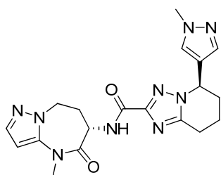
rac-(5R)-5-(1-methylpyrazol-4-yl)-N-[rac-(6S)-4-methyl-5-oxo-7,8-dihydro-6H-pyrazolo[1,5-a][1,3]diazepin-6-yl]-5,6,7,8-tetrahydro-[1,2,4]triazolo[1,5-a]pyridine-2-carboxamide
