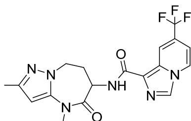
N-(2,4-dimethyl-5-oxo-5,6,7,8-tetrahydro-4H-pyrazolo[1,5-a][1,3]diazepin-6-yl)-7-(trifluoromethyl)imidazo[1,5-a]pyridine-1-carboxamide
