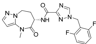
1-[(2,6-difluorophenyl)methyl]-N-[(6S)-4-methyl-5-oxo-7,8-dihydro-6H-pyrazolo[1,5-a][1,3]diazepin-6-yl]-1,2,4-triazole-3-carboxamide
