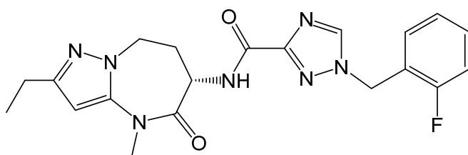
(S)-1-benzyl-N-(2-isopropyl-4-methyl-5-oxo-5,6,7,8-tetrahydro-4H-pyrazolo[1,5-a][1,3]diazepin-6-yl)-1H-1,2,4-triazole-3-carboxamide,
