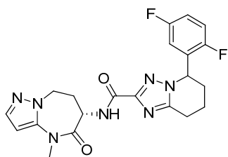
5-(2,5-difluorophenyl)-N-[rac-(6S)-4-methyl-5-oxo-7,8-dihydro-6H-pyrazolo[1,5-a][1,3]diazepin-6-yl]-5,6,7,8-tetrahydro-[1,2,4]triazolo[1,5-a]pyridine-2-carboxamide
