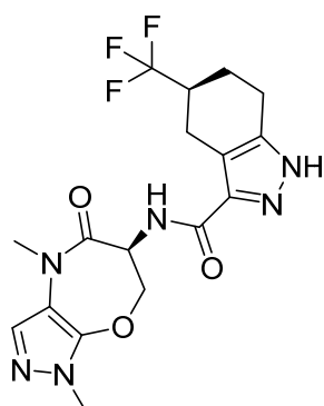
(S)-N-((S)-1,4-dimethyl-5-oxo-4,5,6,7-tetrahydro-1H-pyrazolo[3,4-b][1,4]oxazepin-6-yl)-5-(trifluoromethyl)-4,5,6,7-tetrahydro-1H-indazole-3-carboxamide
