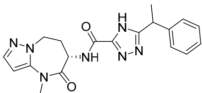
N-((S)-4-methyl-5-oxo-5,6,7,8-tetrahydro-4H-pyrazolo[1,5-a][1,3]diazepin-6-yl)-5-(1-phenylethyl)-4H-1,2,4-triazole-3-carboxamide
