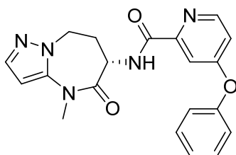
(S)-N-(4-methyl-5-oxo-5,6,7,8-tetrahydro-4H-pyrazolo[1,5-a][1,3]diazepin-6-yl)-4-phenoxycolinamide
