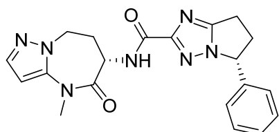
(R)-N-((S)-4-methyl-5-oxo-5,6,7,8-tetrahydro-4H-pyrazolo[1,5-a][1,3]diazepin-6-yl)-5-phenyl-6,7-dihydro-5H-pyrrolo[1,2-b][1,2,4]triazole-2-carboxamide
