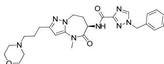
1-benzyl-N-[(6R)-4-methyl-2-(3-morpholinopropyl)-5-oxo-7,8-dihydro-6H-pyrazolo[1,5-a][1,3]diazepin-6-yl]-1,2,4-triazole-3-carboxamide
