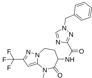
1-benzyl-N-(4-methyl-5-oxo-2-(trifluoromethyl)-5,6,7,8-tetrahydro-4H-pyrazolo[1,5-a][1,3]diazepin-6-yl)-1H-1,2,4-triazole-3-carboxamide
