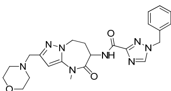
1-benzyl-N-[4-methyl-2-(morpholinomethyl)-5-oxo-7,8-dihydro-6H-pyrazolo[1,5-a][1,3]diazepin-6-yl]-1,2,4-triazole-3-carboxamide
