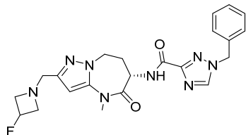
(S)-1-benzyl-N-(2-((3-fluoroazetidin-1-yl)methyl)-4-methyl-5-oxo-5,6,7,8-tetrahydro-4H-pyrazolo[1,5-a][1,3]diazepin-6-yl)-1H-1,2,4-triazole-3-carboxamide
