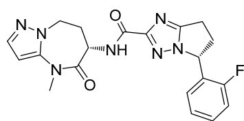
(R)-5-(2-fluorophenyl)-N-((S)-4-methyl-5-oxo-5,6,7,8-tetrahydro-4H-pyrazolo[1,5-a][1,3]diazepin-6-yl)-6,7-dihydro-5H-pyrrolo[1,2-b][1,2,4]triazole-2-carboxamide
