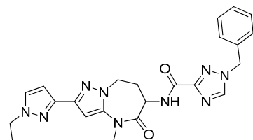
1-benzyl-N-[2-(1-ethylpyrazol-3-yl)-4-methyl-5-oxo-7,8-dihydro-6H-pyrazolo[1,5-a][1,3]diazepin-6-yl]-1,2,4-triazole-3-carboxamide
