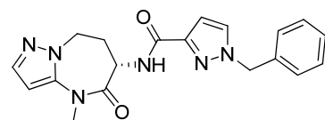
1-benzyl-N-[(6S)-4-methyl-5-oxo-7,8-dihydro-6H-pyrazolo[1,5-
