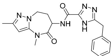
5-benzyl-N-(2,4-dimethyl-5-oxo-5,6,7,8-tetrahydro-4H-pyrazolo[1,5-a][1,3]diazepin-6-yl)-4H-1,2,4-triazole-3-carboxamide
