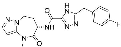
(S)-5-(4-fluorobenzyl)-N-(4-methyl-5-oxo-5,6,7,8-tetrahydro-4H-pyrazolo[1,5-a][1,3]diazepin-6-yl)-4H-1,2,4-triazole-3-carboxamide
