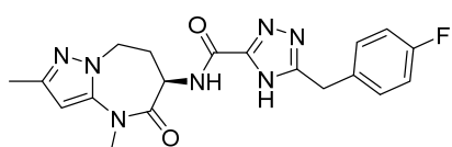
(R)-N-(2,4-dimethyl-5-oxo-5,6,7,8-tetrahydro-4H-pyrazolo[1,5-a][1,3]diazepin-6-yl)-5-(4-fluorobenzyl)-4H-1,2,4-triazole-3-carboxamide
