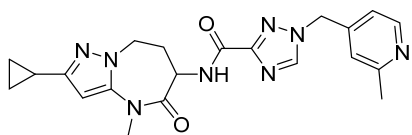
N-(2-cyclopropyl-4-methyl-5-oxo-5,6,7,8-tetrahydro-4H-pyrazolo[1,5-a][1,3]diazepin-6-yl)-1-((2-methylpyridin-4-yl)methyl)-1H-1,2,4-triazole-3-carboxamide
