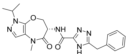
(S)-5-benzyl-N-(1-isopropyl-4-methyl-5-oxo-4,5,6,7-tetrahydro-1H-pyrazolo[3,4-b][1,4]oxazepin-6-yl)-4H-1,2,4-triazole-3-carboxamide
