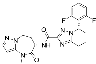
rac-(5S)-5-(2,6-difluorophenyl)-N-[rac-(6S)-4-methyl-5-oxo-7,8-dihydro-6H-pyrazolo[1,5-a][1,3]diazepin-6-yl]-5,6,7,8-tetrahydro-[1,2,4]triazolo[1,5-a]pyridine-2-carboxamide
