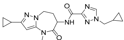
N-(2-cyclopropyl-4-methyl-5-oxo-5,6,7,8-tetrahydro-4H-pyrazolo[1,5-a][1,3]diazepin-6-yl)-1-(cyclopropylmethyl)-1H-1,2,4-triazole-3-carboxamide
