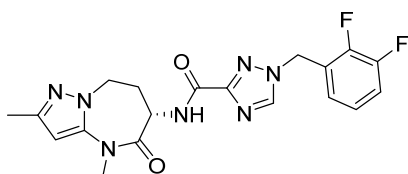
(S)-1-(2,3-difluorobenzyl)-N-(2,4-dimethyl-5-oxo-5,6,7,8-tetrahydro-4H-pyrazolo[1,5-a][1,3]diazepin-6-yl)-1H-1,2,4-triazole-3-carboxamide
