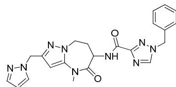
1-benzyl-N-[4-methyl-5-oxo-2-(pyrazol-1-ylmethyl)-7,8-dihydro-6H-pyrazolo[1,5-a][1,3]diazepin-6-yl]-1,2,4-triazole-3-carboxamide
