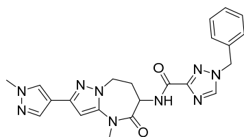
1-benzyl-N-(4-methyl-2-(1-methyl-1H-pyrazol-4-yl)-5-oxo-5,6,7,8-tetrahydro-4H-pyrazolo[1,5-a][1,3]diazepin-6-yl)-1H-1,2,4-triazole-3-carboxamide
