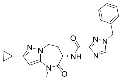
(S)-1-benzyl-N-(2-cyclopropyl-4-methyl-5-oxo-5,6,7,8-tetrahydro-4H-pyrazolo[1,5-a][1,3]diazepin-6-yl)-1H-1,2,4-triazole-3-carboxamide
