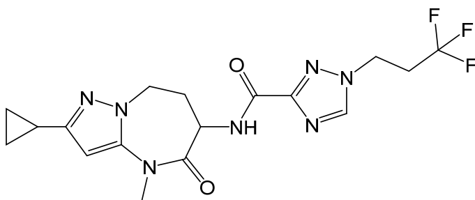
N-(2-cyclopropyl-4-methyl-5-oxo-5,6,7,8-tetrahydro-4H-pyrazolo[1,5-a][1,3]diazepin-6-yl)-1-(3,3,3-trifluoropropyl)-1H-1,2,4-triazole-3-carboxamide.
