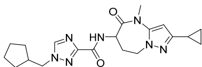
1-(cyclopentylmethyl)-N-(2-cyclopropyl-4-methyl-5-oxo-5,6,7,8-tetrahydro-4H-pyrazolo[1,5-a][1,3]diazepin-6-yl)-1H-1,2,4-triazole-3-carboxamide
