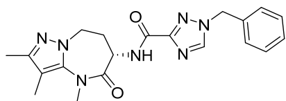
(S)-1-benzyl-N-(2,3,4-trimethyl-5-oxo-5,6,7,8-tetrahydro-4H-pyrazolo[1,5-a][1,3]diazepin-6-yl)-1H-1,2,4-triazole-3-carboxamide
