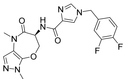
(S)-1-(3,4-difluorobenzyl)-N-(1,4-dimethyl-5-oxo-4,5,6,7-tetrahydro-1H-pyrazolo[3,4-b][1,4]oxazepin-6-yl)-1H-imidazole-4-carboxamide
