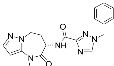
(S)-1-benzyl-N-(4-methyl-5-oxo-5,6,7,8-tetrahydro-4H-pyrazolo[1,5-a][1,3]diazepin-6-yl)-1H-1,2,4-triazole-3-carboxamide
