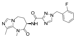
1-[(2-fluorophenyl)methyl]-N-(3R)-1,9-dimethyl-2-oxo-4,5-dihydro-3H-imidazo[1,5-a][1,3]diazepin-3-yl-1,2,4-triazole-3-carboxamide
