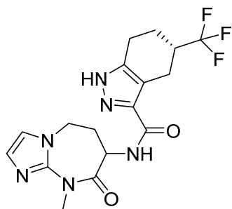
(5S)-N-(9-methyl-8-oxo-6,7,8,9-tetrahydro-5H-imidazo[1,2-a][1,3]diazepin-7-yl)-5-(trifluoromethyl)-4,5,6,7-tetrahydro-1H-indazole-3-carboxamide
