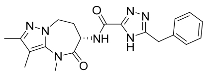
(S)-5-benzyl-N-(2,3,4-trimethyl-5-oxo-5,6,7,8-tetrahydro-4H-pyrazolo[1,5-a][1,3]diazepin-6-yl)-4H-1,2,4-triazole-3-carboxamide
