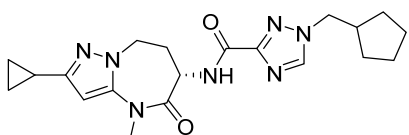
(S)-1-(cyclopentylmethyl)-N-(2-cyclopropyl-4-methyl-5-oxo-5,6,7,8-tetrahydro-4H-pyrazolo[1,5-a][1,3]diazepin-6-yl)-1H-1,2,4-triazole-3-carboxamide
