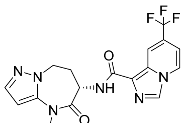
(S)-N-(4-methyl-5-oxo-5,6,7,8-tetrahydro-4H-pyrazolo[1,5-a][1,3]diazepin-6-yl)-7-(trifluoromethyl)imidazo[1,5-a]pyridine-1-carboxamide
