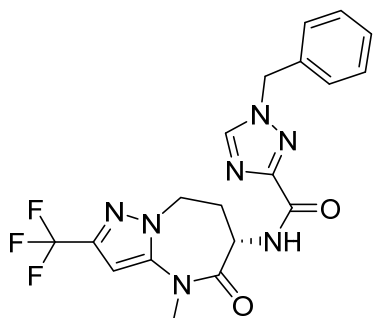
(S)-1-benzyl-N-(4-methyl-5-oxo-2-(trifluoromethyl)-5,6,7,8-tetrahydro-4H-pyrazolo[1,5-a][1,3]diazepin-6-yl)-1H-1,2,4-triazole-3-carboxamide
