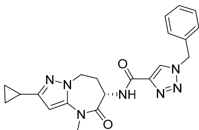
(S)-1-benzyl-N-(2-cyclopropyl-4-methyl-5-oxo-5,6,7,8-tetrahydro-4H-pyrazolo[1,5-a][1,3]diazepin-6-yl)-1H-1,2,3-triazole-4-carboxamide
