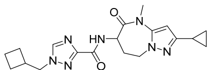
1-(cyclobutylmethyl)-N-(2-cyclopropyl-4-methyl-5-oxo-5,6,7,8-tetrahydro-4H-pyrazolo[1,5-a][1,3]diazepin-6-yl)-1H-1,2,4-triazole-3-carboxamide
