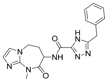
5-benzyl-N-(9-methyl-8-oxo-6,7,8,9-tetrahydro-5H-imidazo[1,2-a][1,3]diazepin-7-yl)-4H-1,2,4-triazole-3-carboxamide
