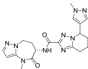
5-(1-methylpyrazol-4-yl)-N-[rac-(6S)-4-methyl-5-oxo-7,8-dihydro-6H-pyrazolo[1,5-a][1,3]diazepin-6-yl]-5,6,7,8-tetrahydro-[1,2,4]triazolo[1,5-a]pyridine-2-
