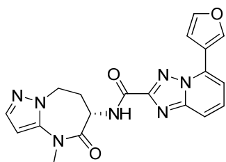
5-(3-furyl)-N-[rac-(6S)-4-methyl-5-oxo-7,8-dihydro-6H-pyrazolo[1,5-a][1,3]diazepin-6-yl]-[1,2,4]triazolo[1,5-a]pyridine-2-carboxamide
