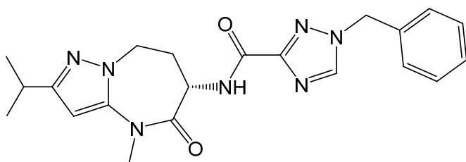
(S)-1-benzyl-N-(2-isopropyl-4-methyl-5-oxo-5,6,7,8-tetrahydro-4H-pyrazolo[1,5-a][1,3]diazepin-6-yl)-1H-1,2,4-triazole-3-carboxamide,
