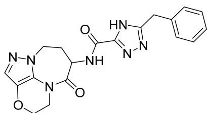
5-benzyl-N-(6-oxo-4,5,6,7,8,9-hexahydro-3-oxa-1,5a,9a-triazabenzocd]azulen-7-yl)-1H-1,2,4-triazole-3-carboxamide
