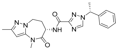
N-((S)-2,4-dimethyl-5-oxo-5,6,7,8-tetrahydro-4H-pyrazolo[1,5-a][1,3]diazepin-6-yl)-1-((R)-1-phenylethyl)-1H-1,2,4-triazole-3-carboxamide
