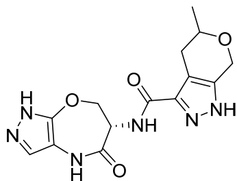
5-methyl-N-((S)-5-oxo-4,5,6,7-tetrahydro-1H-pyrazolo[3,4-b][1,4]oxazepin-6-yl)-1,4,5,7-tetrahydropyrano[3,4-c]pyrazole-3-carboxamide
