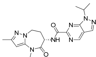
1-isopropyl-N-[(6S)-2,4-dimethyl-5-oxo-7,8-dihydro-6H-pyrazolo[1,5-a][1,3]diazepin-6-yl]pyrazolo[3,4-d]pyrimidine-6-carboxamide
