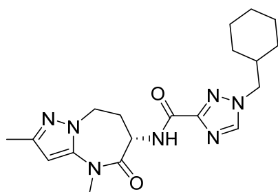
(S)-1-(cyclohexylmethyl)-N-(2,4-dimethyl-5-oxo-5,6,7,8-tetrahydro-4H-pyrazolo[1,5-a][1,3]diazepin-6-yl)-1H-1,2,4-triazole-3-carboxamide
