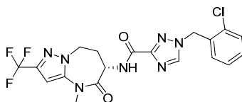
1-[(2-chlorophenyl)methyl]-N-(6S)-4-methyl-5-oxo-2-(trifluoromethyl)-7,8-dihydro-6H-pyrazolo[1,5-a][1,3]diazepin-6-yl-1,2,4-triazole-3-carboxamide
