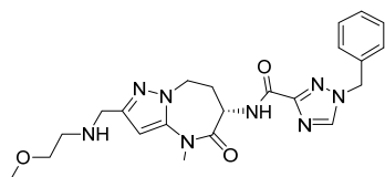
(S)-1-benzyl-N-(2-(((2-methoxyethyl)amino)methyl)-4-methyl-5-oxo-5,6,7,8-tetrahydro-4H-pyrazolo[1,5-a][1,3]diazepin-6-yl)-1H-1,2,4-triazole-3-carboxamide
