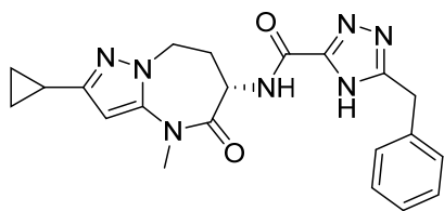
(S)-5-benzyl-N-(2-cyclopropyl-4-methyl-5-oxo-5,6,7,8-tetrahydro-4H-pyrazolo[1,5-a][1,3]diazepin-6-yl)-4H-1,2,4-triazole-3-carboxamide
