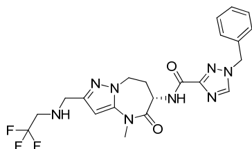
1-benzyl-N-[(6S)-4-methyl-5-oxo-2-[(2,2,2-trifluoroethylamino)methyl]-7,8-dihydro-6H-pyrazolo[1,5-a][1,3]diazepin-6-yl]-1,2,4-triazole-3-carboxamide
