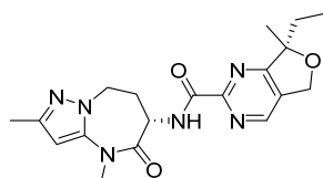
rac-(7S)-7-methyl-N-[rac-(6S)-2,4-dimethyl-5-oxo-7,8-dihydro-6H-pyrazolo[1,5-a][1,3]diazepin-6-yl]-7-(2,2,2-trifluoroethyl)-5H-furo[3,4-d]pyrimidine-2-carboxamide
