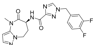
1-[(3,4-difluorophenyl)methyl]-N-[rac-(6S)-4-methyl-5-oxo-7,8-dihydro-6H-pyrazolo[1,5-a][1,3]diazepin-6-yl]-1,2,4-triazole-3-carboxamide
