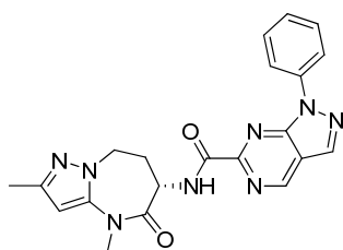
1-phenyl-N-[(6S)-2,4-dimethyl-5-oxo-7,8-dihydro-6H-pyrazolo[1,5-
