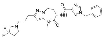
1-benzyl-N-[(6S)-2-[3-(3,3-difluoropyrrolidin-1-yl)propyl]-4-methyl-5-oxo-7,8-dihydro-6H-pyrazolo[1,5-a][1,3]diazepin-6-yl]-1,2,4-triazole-3-carboxamide
