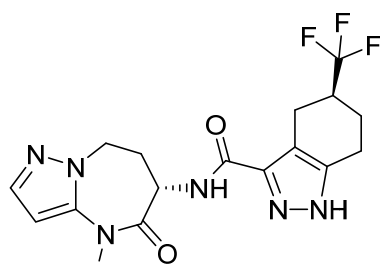
(S)-N-((S)-4-methyl-5-oxo-5,6,7,8-tetrahydro-4H-pyrazolo[1,5-a][1,3]diazepin-6-yl)-5-(trifluoromethyl)-4,5,6,7-tetrahydro-1H-indazole-3-carboxamide
