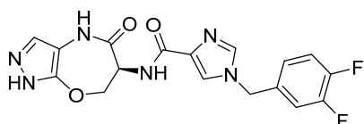
1-[(3,4-difluorophenyl)methyl]-N-[(6S)-5-oxo-1,4,6,7-tetrahydropyrazolo[3,4-b][1,4]oxazepin-6-yl]imidazole-4-carboxamide
