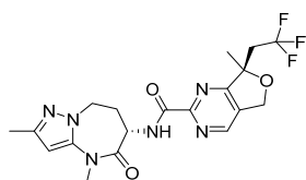
rac-(7R)-7-methyl-N-[rac-(6S)-2,4-dimethyl-5-oxo-7,8-dihydro-6H-pyrazolo[1,5-a][1,3]diazepin-6-yl]-7-(2,2,2-trifluoroethyl)-5H-furo[3,4-d]pyrimidine-2-carboxamide
