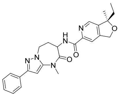
(3R)-3-ethyl-3-methyl-N-(4-methyl-5-oxo-2-phenyl-5,6,7,8-tetrahydro-4H-pyrazolo[1,5-a][1,3]diazepin-6-yl)-1,3-dihydrofuro[3,4-c]pyridine-6-carboxamide
