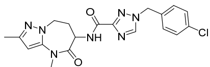
1-(4-chlorobenzyl)-N-(2,4-dimethyl-5-oxo-5,6,7,8-tetrahydro-4H-pyrazolo[1,5-a][1,3]diazepin-6-yl)-1H-1,2,4-triazole-3-carboxamide
