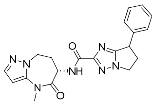
7-phenyl-N-[rac-(6S)-4-methyl-5-oxo-7,8-dihydro-6H-pyrazolo[1,5-a][1,3]diazepin-6-yl]-6,7-dihydro-5H-pyrrolo[1,2-b][1,2,4]triazole-2-carboxamide
