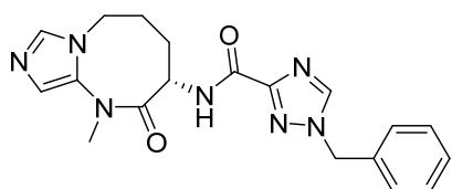
(S)-1-benzyl-N-(1-methyl-2-oxo-1,2,3,4,5,6-hexahydroimidazo[1,5-a][1,3]diazocin-3-yl)-1H-1,2,4-triazole-3-carboxamide
