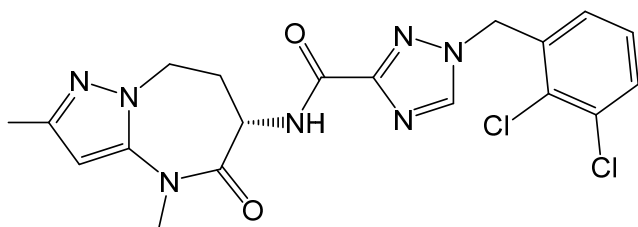
1-[(2,3-dichlorophenyl)methyl]-N-(6S)-2,4-dimethyl-5-oxo-7,8-dihydro-6H-pyrazolo[1,5-a][1,3]diazepin-6-yl-1H-1,2,4-triazole-3-carboxamide, and
