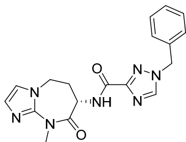
(S)-1-benzyl-N-(9-methyl-8-oxo-6,7,8,9-tetrahydro-5H-imidazo[1,2-a][1,3]diazepin-7-yl)-1H-1,2,4-triazole-3-carboxamide
