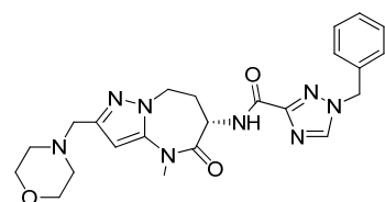
1-benzyl-N-[(6S)-4-methyl-2-(morpholinomethyl)-5-oxo-7,8-dihydro-6H-pyrazolo[1,5-a][1,3]diazepin-6-yl]-1,2,4-triazole-3-carboxamide
