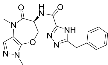
(S)-5-benzyl-N-(1,4-dimethyl-5-oxo-4,5,6,7-tetrahydro-1H-pyrazolo[3,4-b][1,4]oxazepin-6-yl)-4H-1,2,4-triazole-3-carboxamide
