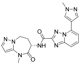
N-[(6S)-4-methyl-5-oxo-7,8-dihydro-6H-pyrazolo[1,5-a][1,3]diazepin-6-yl]-5-(1-methylpyrazol-4-yl)-[1,2,4]triazolo[1,5-a]pyridine-2-carboxamide
