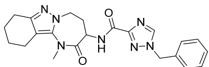
1-benzyl-N-(1-methyl-2-oxo-2,3,4,5,8,9,10,11-octahydro-1H-[1,3]diazepino[1,2-b]indazol-3-yl)-1H-1,2,4-triazole-3-carboxamide
