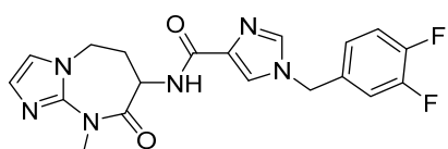
1-(3,4-difluorobenzyl)-N-(9-methyl-8-oxo-6,7,8,9-tetrahydro-5H-imidazo[1,2-a][1,3]diazepin-7-yl)-1H-imidazole-4-carboxamide
