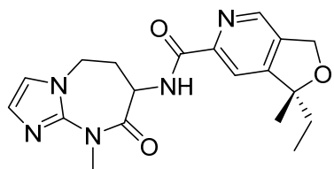
(1R)-1-ethyl-1-methyl-N-(9-methyl-8-oxo-6,7,8,9-tetrahydro-5H-imidazo[1,2-a][1,3]diazepin-7-yl)-1,3-dihydrofuro[3,4-c]pyridine-6-carboxamide
