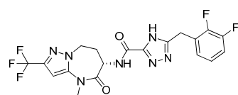
5-[(2,3-difluorophenyl)methyl]-N-(6S)-4-methyl-5-oxo-2-(trifluoromethyl)-7,8-dihydro-6H-pyrazolo[1,5-a][1,3]diazepin-6-yl-4H-1,2,4-triazole-3-carboxamide
