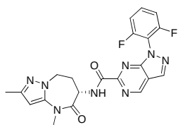
1-(2,6-difluorophenyl)-N-[(6S)-2,4-dimethyl-5-oxo-7,8-dihydro-6H-pyrazolo[1,5-a][1,3]diazepin-6-yl]pyrazolo[3,4-d]pyrimidine-6-carboxamide
