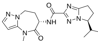
(5S)-5-isopropyl-N-[(6S)-4-methyl-5-oxo-7,8-dihydro-6H-pyrazolo[1,5-a][1,3]diazepin-6-yl]-6,7-dihydro-5H-pyrrolo[1,2-b][1,2,4]triazole-2-carboxamide
