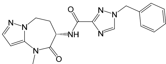
(S)-1-benzyl-N-(4-methyl-5-oxo-5,6,7,8-tetrahydro-4H-pyrazolo[1,5-a][1,3]diazepin-6-yl)-1H-1,2,4-triazole-3-carboxamide,
