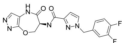
1-[(3,4-difluorophenyl)methyl]-N-[(6S)-5-oxo-1,4,6,7-tetrahydropyrazolo[3,4-b][1,4]oxazepin-6-yl]pyrazole-3-carboxamide
