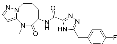
5-(4-fluorobenzyl)-N-(4-methyl-5-oxo-4,5,6,7,8,9-hexahydropyrazolo[1,5-a][1,3]diazocin-6-yl)-4H-1,2,4-triazole-3-carboxamide
