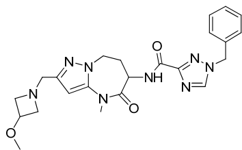
1-benzyl-N-[2-[(3-methoxyazetidin-1-yl)methyl]-4-methyl-5-oxo-7,8-dihydro-6H-pyrazolo[1,5-a][1,3]diazepin-6-yl]-1,2,4-triazole-3-carboxamide
