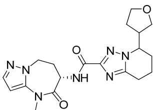
N-[(6S)-4-methyl-5-oxo-7,8-dihydro-6H-pyrazolo[1,5-a][1,3]diazepin-6-yl]-5-tetrahydrofuran-3-yl-5,6,7,8-tetrahydro-[1,2,4]triazolo[1,5-a]pyridine-2-carboxamide
