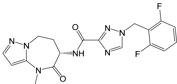
1-[(2,6-difluorophenyl)methyl]-N-[(6S)-4-methyl-5-oxo-7,8-dihydro-6H-pyrazolo[1,5-a][1,3]diazepin-6-yl]-1,2,4-triazole-3-carboxamide,
