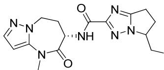
5-ethyl-N-[(6S)-4-methyl-5-oxo-7,8-dihydro-6H-pyrazolo[1,5-a][1,3]diazepin-6-yl]-6,7-dihydro-5H-pyrrolo[1,2-b][1,2,4]triazole-2-carboxamide
