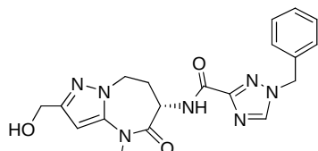
1-benzyl-N-[(6S)-2-(hydroxymethyl)-4-methyl-5-oxo-7,8-dihydro-6H-pyrazolo[1,5-a][1,3]diazepin-6-yl]-1,2,4-triazole-3-carboxamide
