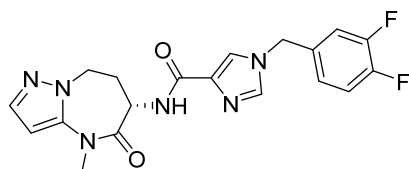
(S)-1-(3,4-difluorobenzyl)-N-(4-methyl-5-oxo-5,6,7,8-tetrahydro-4H-pyrazolo[1,5-a][1,3]diazepin-6-yl)-1H-imidazole-4-carboxamide
