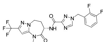
1-[(2,3-difluorophenyl)methyl]-N-(6S)-4-methyl-5-oxo-2-(trifluoromethyl)-7,8-dihydro-6H-pyrazolo[1,5-a][1,3]diazepin-6-yl-1,2,4-triazole-3-carboxamide
