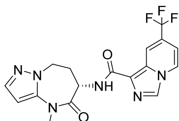
(S)-N-(4-methyl-5-oxo-5,6,7,8-tetrahydro-4H-pyrazolo[1,5-a][1,3]diazepin-6-yl)-7-(trifluoromethyl)imidazo[1,5-a]pyridine-1-carboxamide
