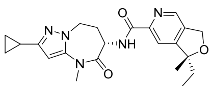
(R)-N-((S)-2-cyclopropyl-4-methyl-5-oxo-5,6,7,8-tetrahydro-4H-pyrazolo[1,5-a][1,3]diazepin-6-yl)-1-ethyl-1-methyl-1,3-dihydrofuro[3,4-c]pyridine-6-carboxamide
