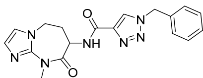
1-benzyl-N-(9-methyl-8-oxo-6,7,8,9-tetrahydro-5H-imidazo[1,2-a][1,3]diazepin-7-yl)-1H-1,2,3-triazole-4-carboxamide
