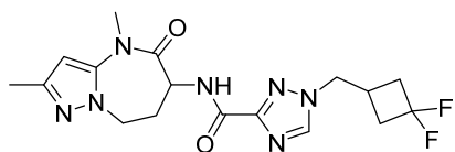
1-((3,3-difluorocyclobutyl)methyl)-N-(2,4-dimethyl-5-oxo-5,6,7,8-tetrahydro-4H-pyrazolo[1,5-a][1,3]diazepin-6-yl)-1H-1,2,4-triazole-3-carboxamide
