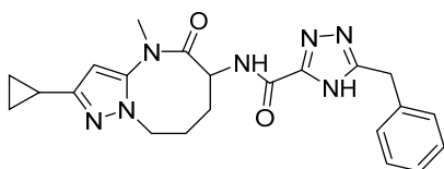
5-benzyl-N-(2-cyclopropyl-4-methyl-5-oxo-4,5,6,7,8,9-hexahydropyrazolo[1,5-a][1,3]diazocin-6-yl)-4H-1,2,4-triazole-3-carboxamide
