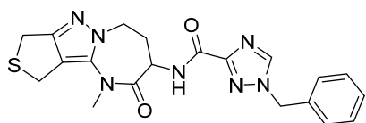
1-benzyl-N-(1-methyl-2-oxo-1,2,3,4,5,10-hexahydro-8H-thieno[3',4':3,4]pyrazolo[1,5-a][1,3]diazepin-3-yl)-1H-1,2,4-triazole-3-carboxamide
