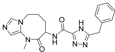
5-benzyl-N-(1-methyl-2-oxo-1,2,3,4,5,6-hexahydroimidazo[1,5-a][1,3]diazocin-3-yl)-4H-1,2,4-triazole-3-carboxamide
