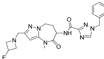
1-benzyl-N-[2-[(3-fluoroazetidin-1-yl)methyl]-4-methyl-5-oxo-7,8-dihydro-6H-pyrazolo[1,5-a][1,3]diazepin-6-yl]-1,2,4-triazole-3-carboxamide
