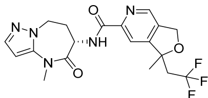
1-methyl-N-((S)-4-methyl-5-oxo-5,6,7,8-tetrahydro-4H-pyrazolo[1,5-a][1,3]diazepin-6-yl)-1-(2,2,2-trifluoroethyl)-1,3-dihydrofuro[3,4-c]pyridine-6-carboxamide
