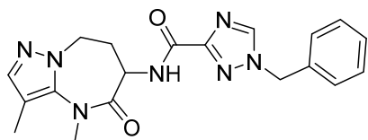
1-benzyl-N-(3,4-dimethyl-5-oxo-5,6,7,8-tetrahydro-4H-pyrazolo[1,5-a][1,3]diazepin-6-yl)-1H-1,2,4-triazole-3-carboxamide
