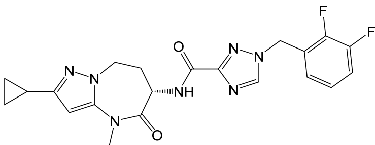
(S)-N-(2-cyclopropyl-4-methyl-5-oxo-5,6,7,8-tetrahydro-4H-pyrazolo[1,5-a][1,3]diazepin-6-yl)-1-(2,3-difluorobenzyl)-1H-1,2,4-triazole-3-carboxamide,
