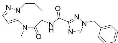
1-benzyl-N-(4-methyl-5-oxo-4,5,6,7,8,9-hexahydropyrazolo[1,5-a][1,3]diazocin-6-yl)-1H-1,2,4-triazole-3-carboxamide
