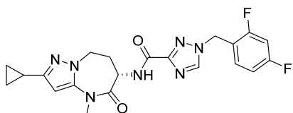
(S)-N-(2-cyclopropyl-4-methyl-5-oxo-5,6,7,8-tetrahydro-4H-pyrazolo[1,5-a][1,3]diazepin-6-yl)-1-(2,4-difluorobenzyl)-1H-1,2,4-triazole-3-carboxamide
