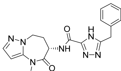
(S)-5-benzyl-N-(4-methyl-5-oxo-5,6,7,8-tetrahydro-4H-pyrazolo[1,5-a][1,3]diazepin-6-yl)-4H-1,2,4-triazole-3-carboxamide
