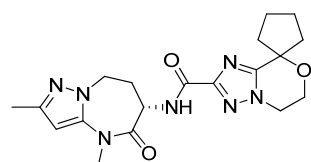
N-[(6S)-2,4-dimethyl-5-oxo-7,8-dihydro-6H-pyrazolo[1,5-a][1,3]diazepin-6-yl]spiro[5,6-dihydro-[1,2,4]triazolo[5,1-c][1,4]oxazine-8,1'-cyclopentane]-2-carboxamide
