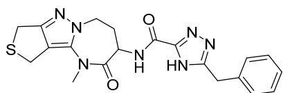
5-benzyl-N-(1-methyl-2-oxo-1,2,3,4,5,10-hexahydro-8H-thieno[3',4':3,4]pyrazolo[1,5-a][1,3]diazepin-3-yl)-4H-1,2,4-triazole-3-carboxamide
