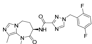
1-[(2,5-difluorophenyl)methyl]-N-(3R)-1,9-dimethyl-2-oxo-4,5-dihydro-3H-imidazo[1,5-a][1,3]diazepin-3-yl-1,2,4-triazole-3-carboxamide
