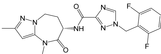
(S)-1-(2,6-difluorobenzyl)-N-(2,4-dimethyl-5-oxo-5,6,7,8-tetrahydro-4H-pyrazolo[1,5-a][1,3]diazepin-6-yl)-1H-1,2,4-triazole-3-carboxamide,
