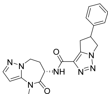
N-((S)-4-methyl-5-oxo-5,6,7,8-tetrahydro-4H-pyrazolo[1,5-a][1,3]diazepin-6-yl)-5-phenyl-5,6-dihydro-4H-pyrrolo[1,2-c][1,2,3]triazole-3-carboxamide
