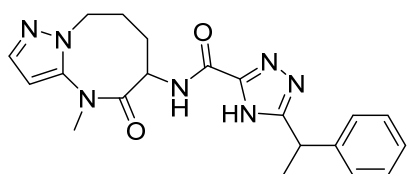
N-(4-methyl-5-oxo-4,5,6,7,8,9-hexahydropyrazolo[1,5-a][1,3]diazocin-6-yl)-5-(1-phenylethyl)-4H-1,2,4-triazole-3-carboxamide
