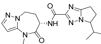
5-isopropyl-N-[(6S)-4-methyl-5-oxo-7,8-dihydro-6H-pyrazolo[1,5-a][1,3]diazepin-6-yl]-6,7-dihydro-5H-pyrrolo[1,2-b][1,2,4]triazole-2-carboxamide
