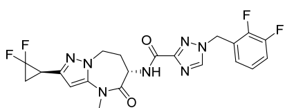
1-(2,3-difluorobenzyl)-N-((S)-2-((R)-2,2-difluorocyclopropyl)-4-methyl-5-oxo-5,6,7,8-tetrahydro-4H-pyrazolo[1,5-a][1,3]diazepin-6-yl)-1H-1,2,4-triazole-3-carboxamide
