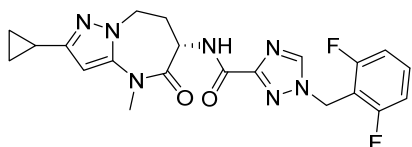
(S)-N-(2-cyclopropyl-4-methyl-5-oxo-5,6,7,8-tetrahydro-4H-pyrazolo[1,5-a][1,3]diazepin-6-yl)-1-(2,6-difluorobenzyl)-1H-1,2,4-triazole-3-carboxamide
