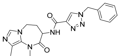
1-benzyl-N-(1,9-dimethyl-2-oxo-2,3,4,5-tetrahydro-1H-imidazo[1,5-a][1,3]diazepin-3-yl)-1H-1,2,3-triazole-4-carboxamide
