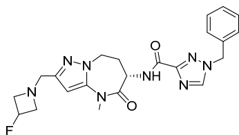
(S)-1-benzyl-N-(2-((3-fluoroazetidin-1-yl)methyl)-4-methyl-5-oxo-5,6,7,8-tetrahydro-4H-pyrazolo[1,5-a][1,3]diazepin-6-yl)-1H-1,2,4-triazole-3-carboxamide
