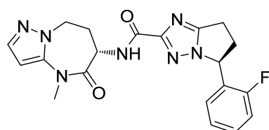
(S)-5-(2-fluorophenyl)-N-((S)-4-methyl-5-oxo-5,6,7,8-tetrahydro-4H-pyrazolo[1,5-a][1,3]diazepin-6-yl)-6,7-dihydro-5H-pyrrolo[1,2-b][1,2,4]triazole-2-carboxamide
