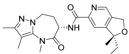
(R)-1-ethyl-1-methyl-N-((S)-2,3,4-trimethyl-5-oxo-5,6,7,8-tetrahydro-4H-pyrazolo[1,5-a][1,3]diazepin-6-yl)-1,3-dihydrofuro[3,4-c]pyridine-6-carboxamide
