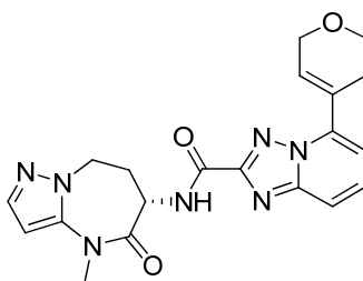
5-(3,6-dihydro-2H-pyran-4-yl)-N-[(6S)-4-methyl-5-oxo-7,8-dihydro-6H-pyrazolo[1,5-a][1,3]diazepin-6-yl]-[1,2,4]triazolo[1,5-a]pyridine-2-carboxamide
