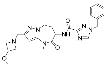
1-benzyl-N-[2-[(3-methoxyazetidin-1-yl)methyl]-4-methyl-5-oxo-7,8-dihydro-6H-pyrazolo[1,5-a][1,3]diazepin-6-yl]-1,2,4-triazole-3-carboxamide
