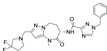
(S)-1-benzyl-N-(2-((3,3-difluoropyrrolidin-1-yl)methyl)-4-methyl-5-oxo-5,6,7,8-tetrahydro-4H-pyrazolo[1,5-a][1,3]diazepin-6-yl)-1H-1,2,4-triazole-3-carboxamide
