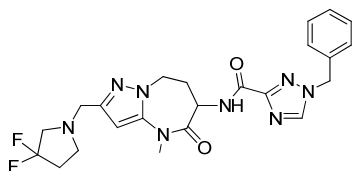
1-benzyl-N-[2-[(3,3-difluoropyrrolidin-1-yl)methyl]-4-methyl-5-oxo-7,8-dihydro-6H-pyrazolo[1,5-a][1,3]diazepin-6-yl]-1,2,4-triazole-3-carboxamide
