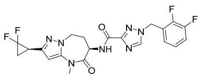
1-(2,3-difluorobenzyl)-N-((R)-2-((R)-2,2-difluorocyclopropyl)-4-methyl-5-oxo-5,6,7,8-tetrahydro-4H-pyrazolo[1,5-a][1,3]diazepin-6-yl)-1H-1,2,4-triazole-3-carboxamide
