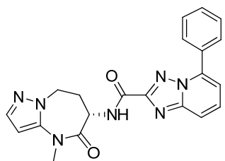
N-[(6S)-4-methyl-5-oxo-7,8-dihydro-6H-pyrazolo[1,5-a][1,3]diazepin-6-yl]-5-phenyl-[1,2,4]triazolo[1,5-a]pyridine-2-carboxamide
