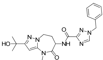
1-benzyl-N-[2-(1-hydroxy-1-methyl-ethyl)-4-methyl-5-oxo-7,8-dihydro-6H-pyrazolo[1,5-a][1,3]diazepin-6-yl]-1,2,4-triazole-3-carboxamide
