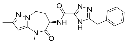
(R)-5-benzyl-N-(2,4-dimethyl-5-oxo-5,6,7,8-tetrahydro-4H-pyrazolo[1,5-a][1,3]diazepin-6-yl)-4H-1,2,4-triazole-3-carboxamide
