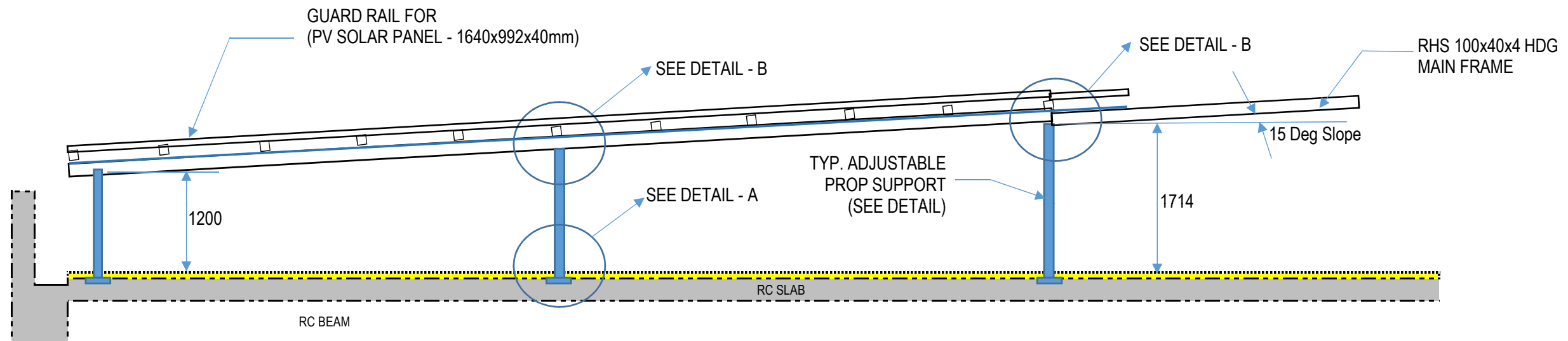
SECTIONAL VIEW OF HDB HOUSING FLAT ROOF
