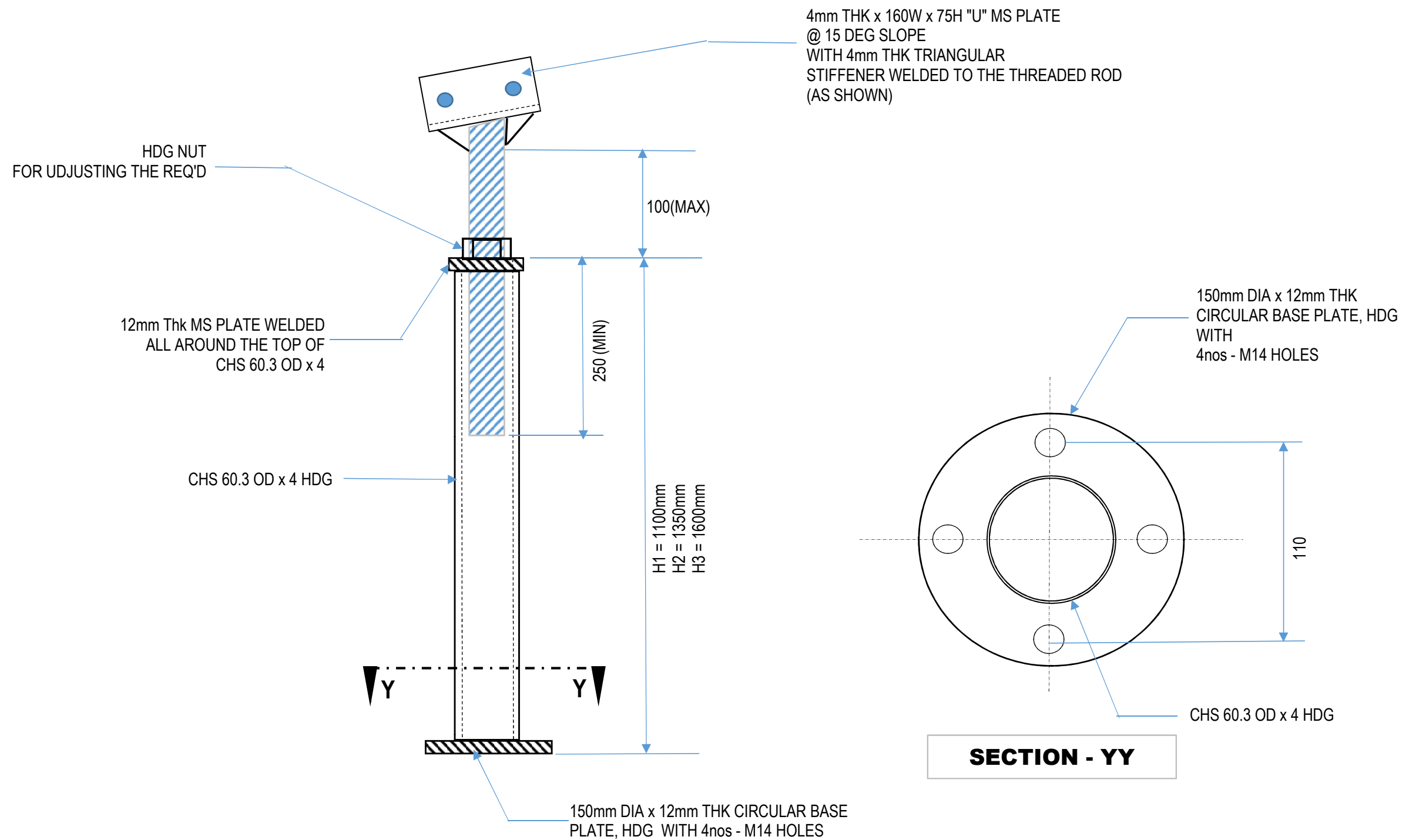
TYP. DETAIL OF ADJUSTABLE PROP SUPPORT
