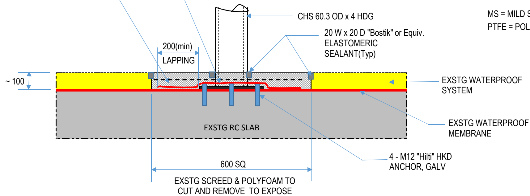
DETAIL - A
