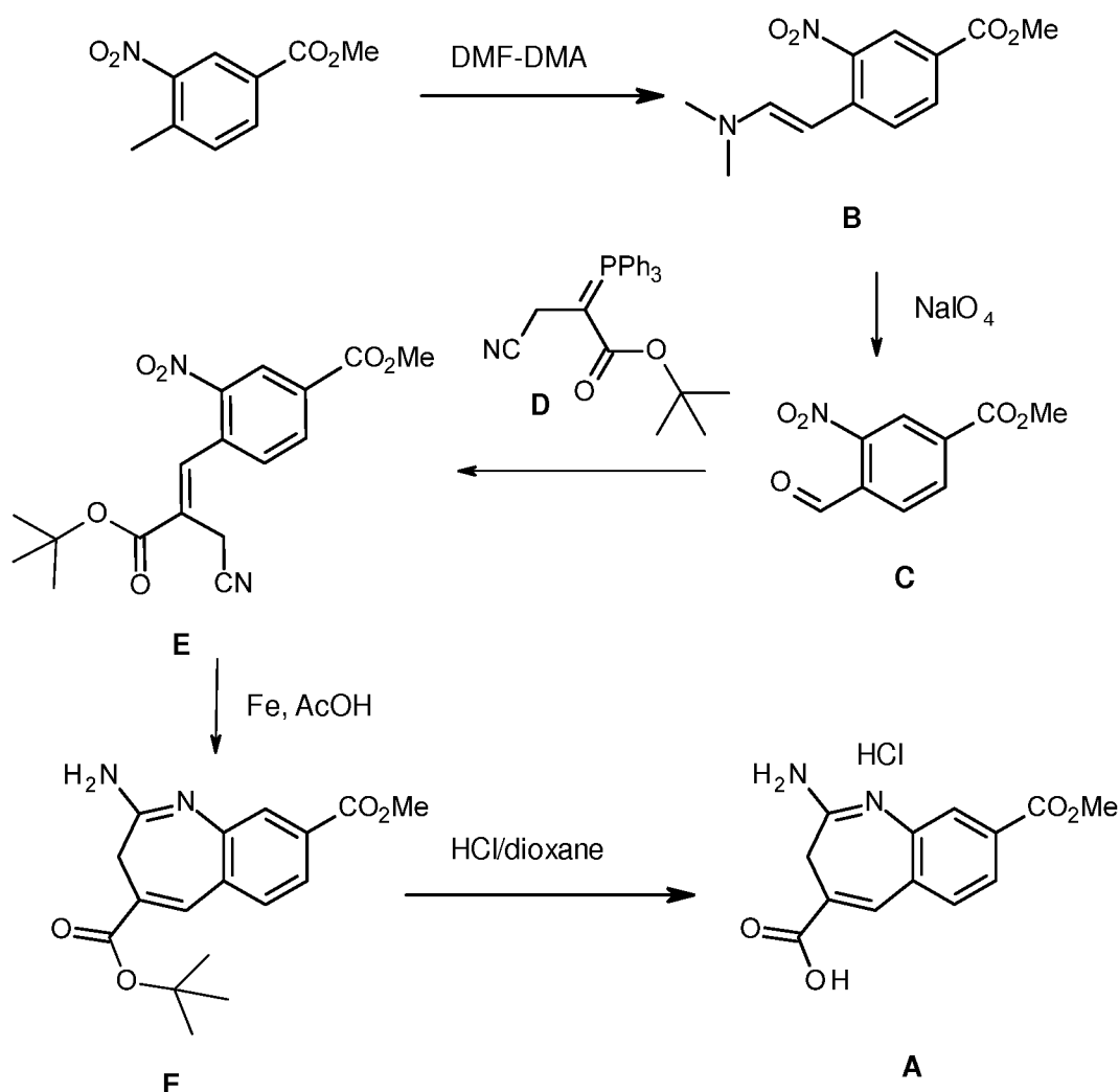
Scheme 2
