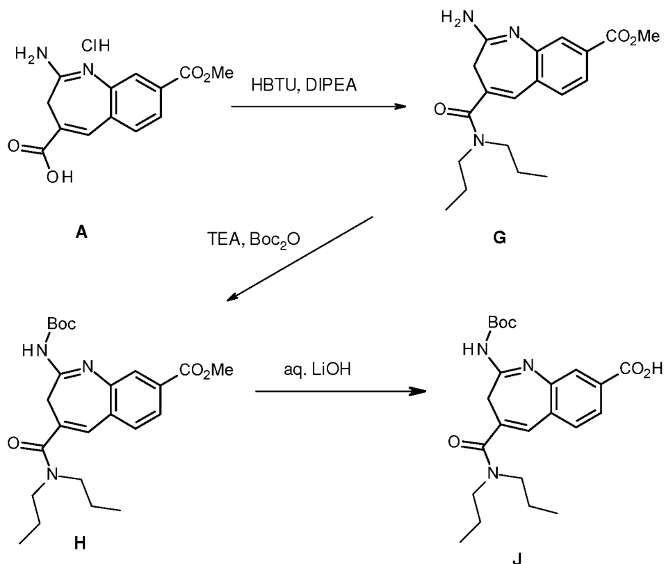
Scheme 3
