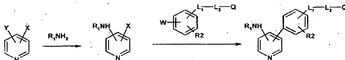
Scheme 4
