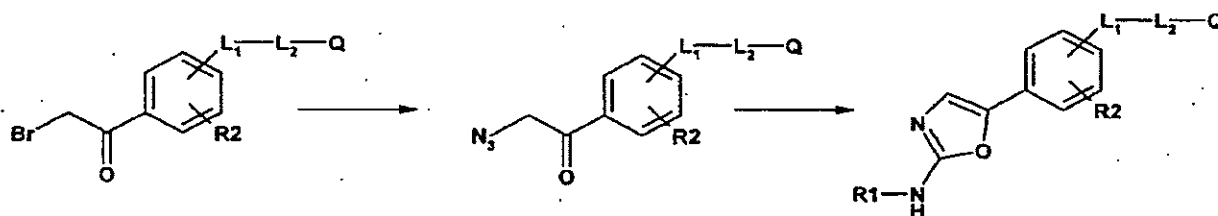
Scheme 3
