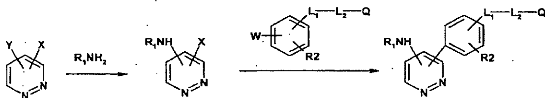
Scheme 5
