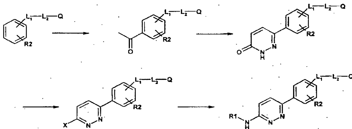
Scheme 6
