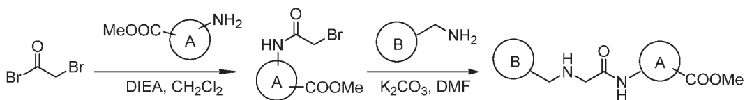
Scheme 8
