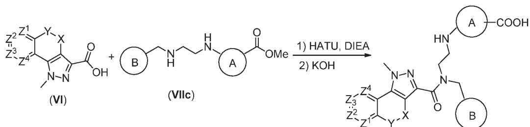
Scheme 3
