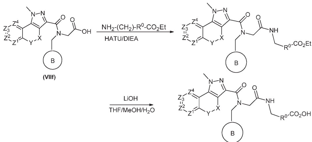
Scheme 6
