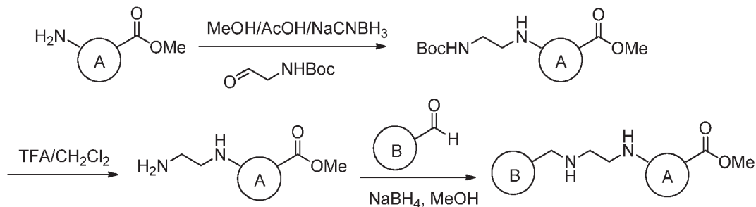
Scheme 10
