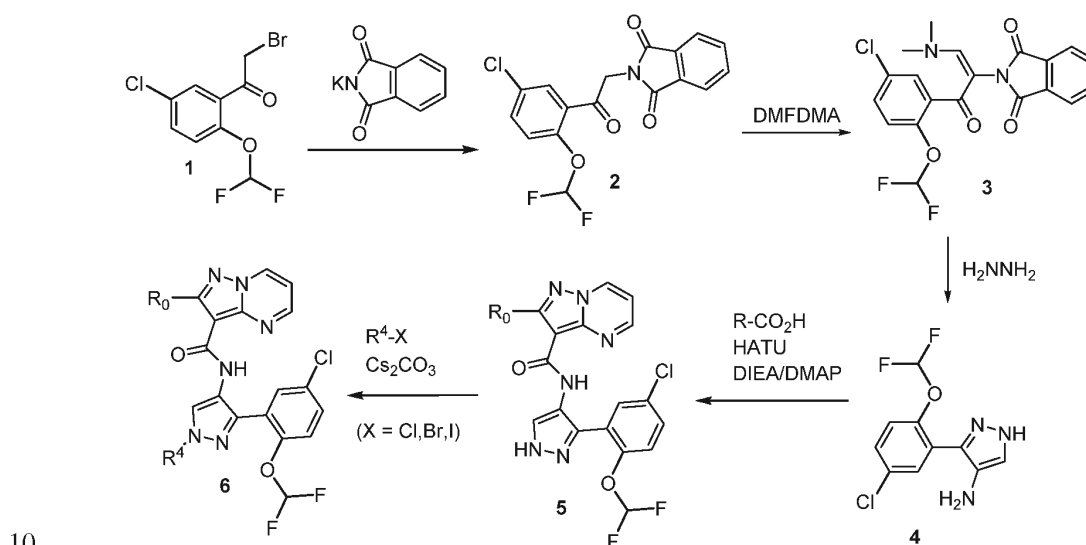
Reaction Scheme 3
