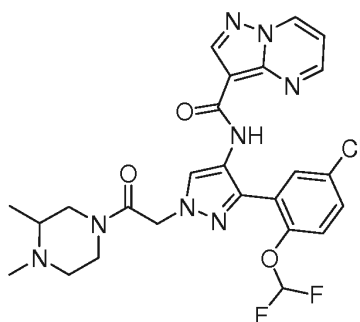
N-[3-[5-chloro-2-(difluoromethoxy)phenyl]-1-[2-(3,4-dimethylpiperazin-1-yl)-2-oxoethyl]-1H-pyrazol-4-yl]pyrazolo[1,5-a]pyrimidine-3-carboxamide
