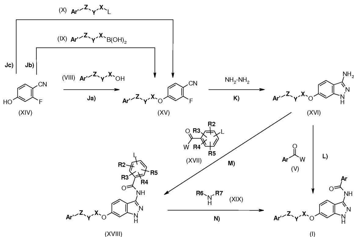
Scheme 2
