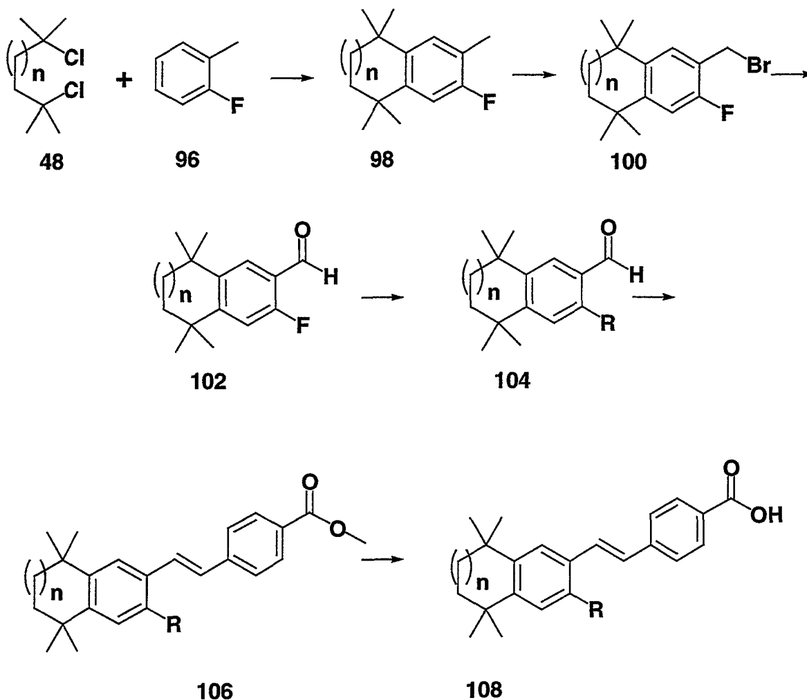
SCHEME 4
