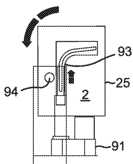
Step 2: intermediate step of the dispensing process
