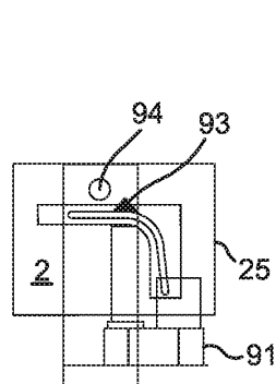
Step 1: beginning of the dispensing process
