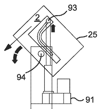
Step 3: end of the dispensing process
