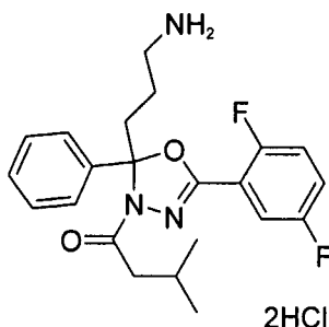
1-(2-(3-aminopropyl)-5-(2,5-difluorophenyl)-2-phenyl-1,3,4-oxadiazol-3(2H)-yl)-3-methylbutan-1-one dihydrochloride
