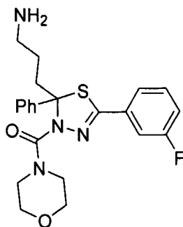
[2-(3-Aminopropyl)-5-(3-fluorophenyl)-2-phenyl-[1,3,4]thiadiazol-3-yl]-morpholin-4-yl-methanone
