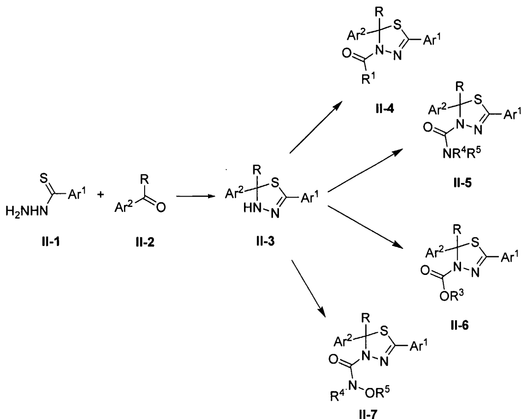
Scheme II
