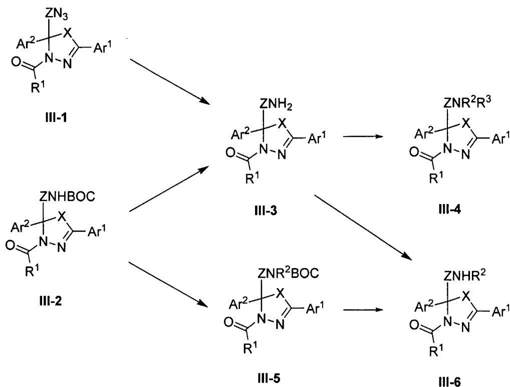
Scheme III
