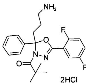
1-(2-(3-aminopropyl)-5-(2,5-difluorophenyl)-2-phenyl-1,3,4-oxadiazol-3(2H)-yl)-2,2-dimethylpropan-1-one dihydrochloride
