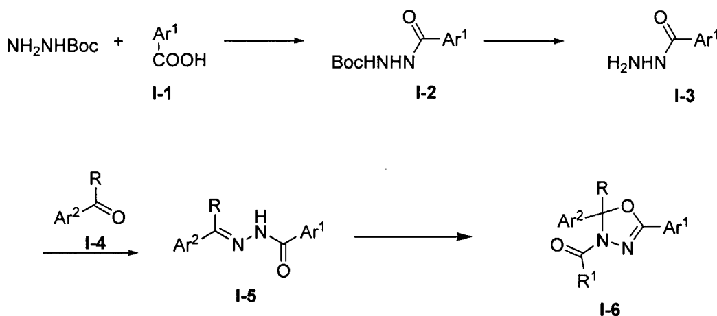
Scheme I
