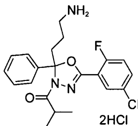
1-(2-(3-aminopropyl)-5-(5-chloro-2-fluorophenyl)-2-phenyl-1,3,4-oxadiazol-3(2H)-yl)-2-methylpropan-1-one dihydrochloride
