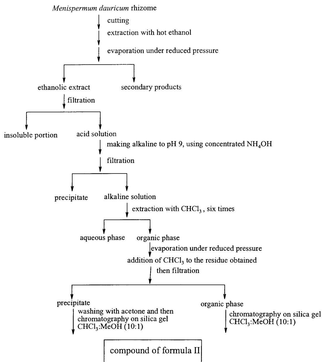
Figure 1 : Extraction of the compound of formula II
