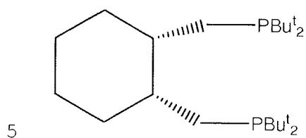
cis- 1, 2-bis (di-tert-butylphosphinomethyl) cyclohexane
