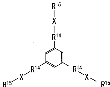
Structural formula (8)
