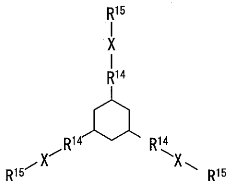
Structural formula (9)
