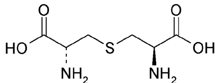
Lanthionine
