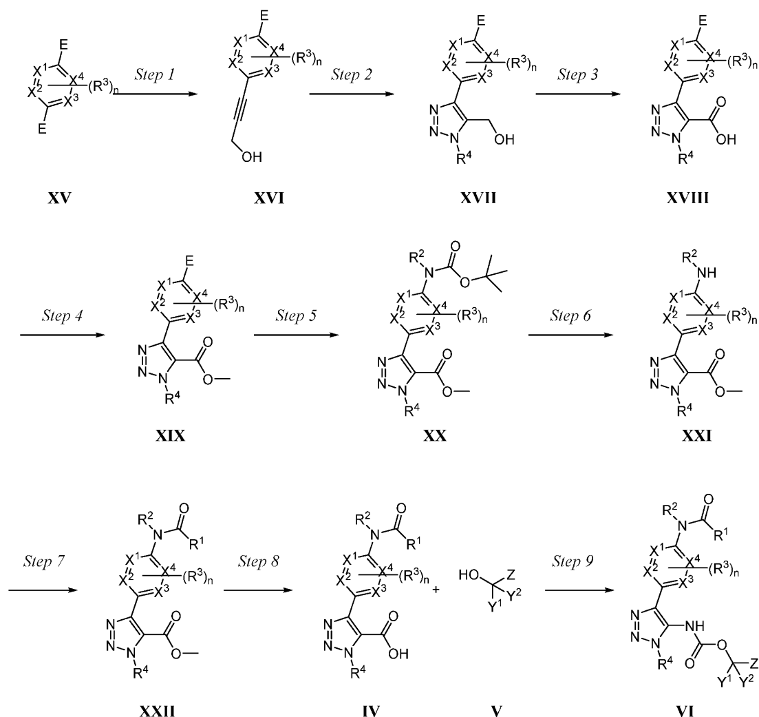
Scheme D
