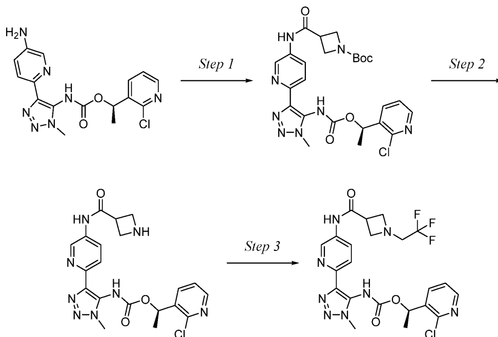
Compound 309
