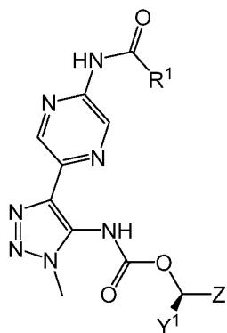
(IIIm)
