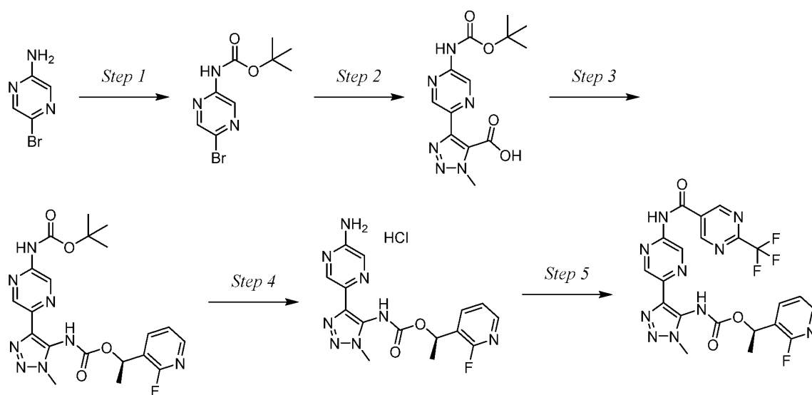
Compound 325
