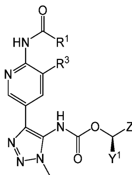
(IIc)
