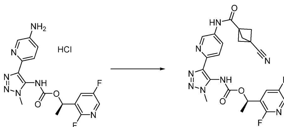
Compound 162
