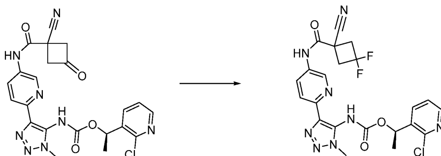
Compound 186
