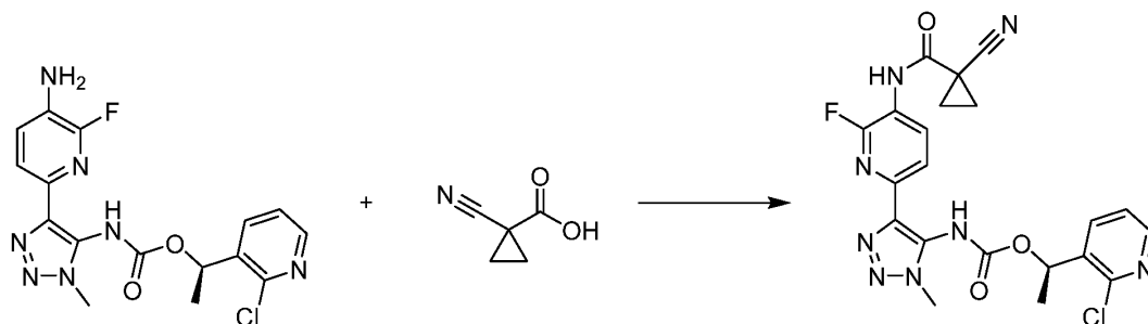
Compound 316
