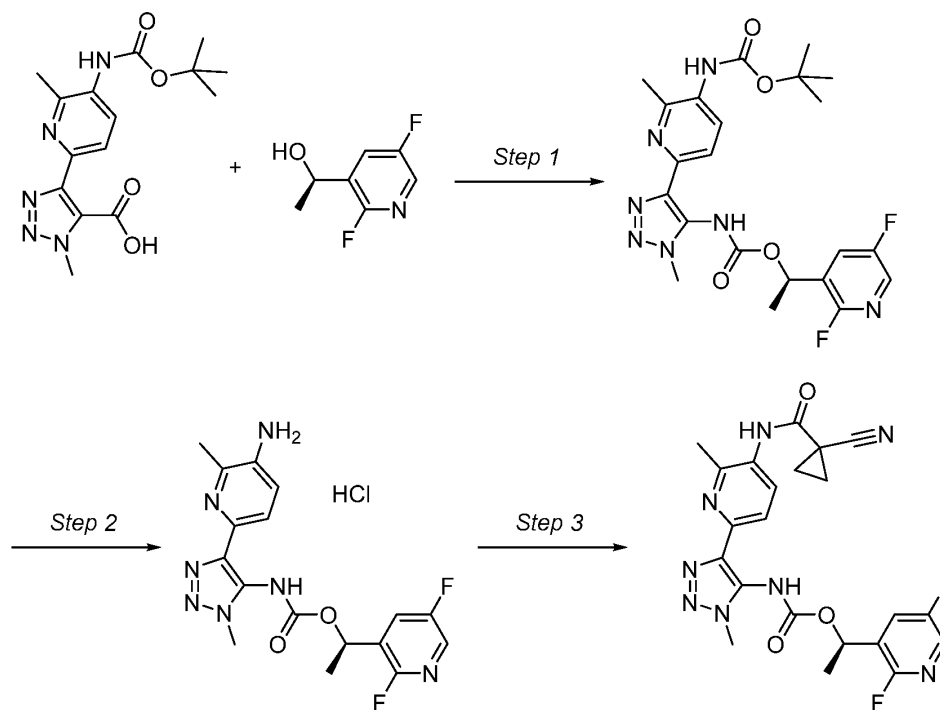
Compound 313
