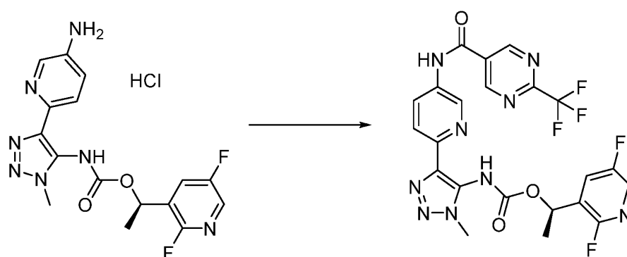
Compound 251
