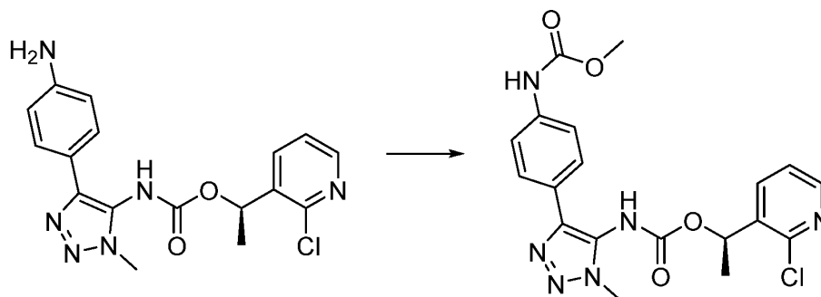
Compound 7
