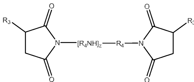
Formula (IV)
