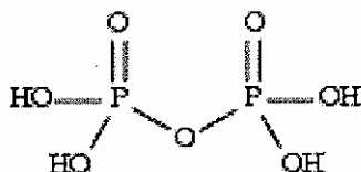
Pyrophosphoric acid
