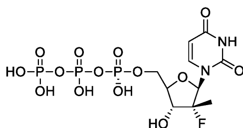
2'-Deoxy-2'- \alpha -fluoro- \beta -C-methyluridine-5'-triphosphate
