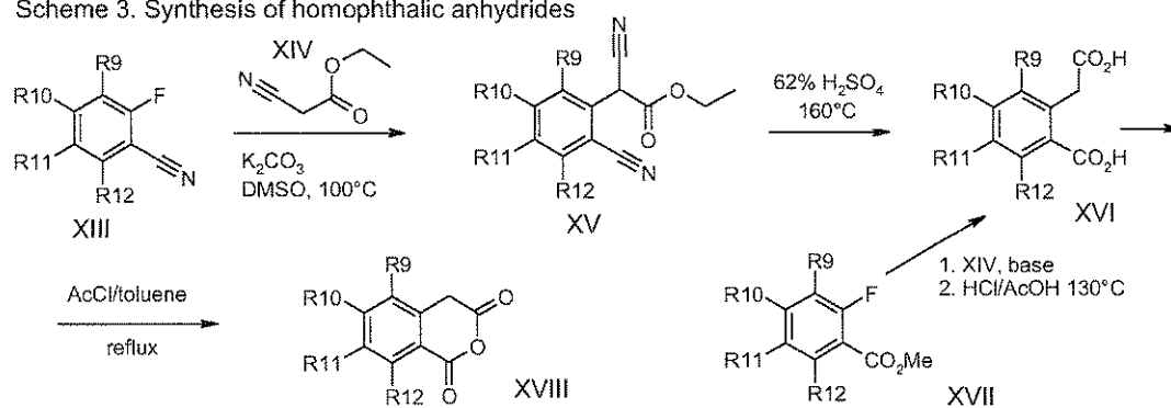
Scheme 3. Synthesis of homophthalic anhydrides
