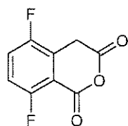
5,8-Difluoro-isochroman-1,3-dione.
