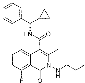
10 2j 8-Fluoro-2-isobutylamino-3-methyl-1-oxo-1,2-dihydro-isoquinoline-4-carboxylic acid ((S)-cyclopropyl-phenyl-methyl)-amide.
