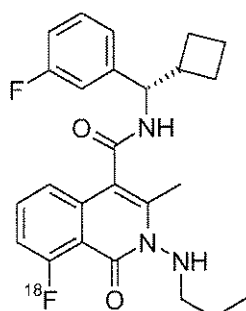
5 8-( 18 F)-Fluoro-3-methyl-1-oxo-2-propylamino-1,2-dihydro-isoquinoline-4-carboxylic acid [(S)-cyclobutyl-(3-fluoro-phenyl)-methyl]-amide
