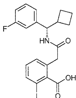
2-([(S)-Cyclobutyl-(3-fluoro-phenyl)-methyl]-carbamoyl)-methyl)-6-iodo-benzoic acid.
