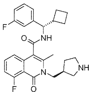
5c 8-Fluoro-3-methyl-1-oxo-2-(S)-1-pyrrolidin-3-ylmethyl-1,2-dihydro-isoquinoline-4-carboxylic acid [(S)-cyclobutyl-(3-fluoro-phenyl)-methyl]-amide.
