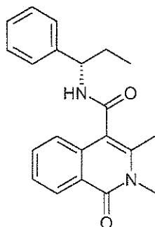
1y 2,3-Dimethyl-1-oxo-1,2-dihydro-isoquinoline-4-carboxylic acid ((S)-1-phenyl-propyl)-amide.
