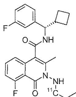
5 8-Fluoro-3-methyl-1-oxo-2-((1- 11 C)-propylamino)-1,2-dihydro-isoquinoline-4-carboxylic acid [(S)-cyclobutyl-(3-fluoro-phenyl)-methyl]-amide
