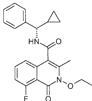
1u 2-Ethoxy-8-fluoro-3-methyl-1-oxo-1,2-dihydro-isoquinoline-4-carboxylic acid ((S)-cyclopropyl-phenyl-methyl)-amide.
