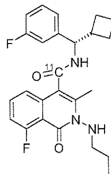
10 8-Fluoro-3-methyl-1-oxo-2-propylamino-1,2-dihydro-isoquinoline-4-( 11 C)-carboxylic acid [(S)-cyclobutyl-(3-fluoro-phenyl)-methyl]-amide
