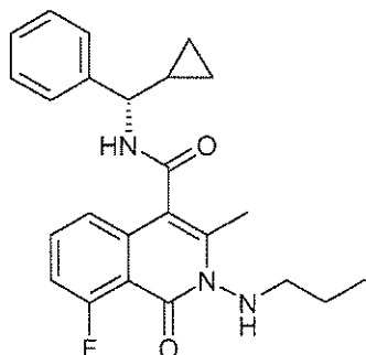
2k 8-Fluoro-3-methyl-1-oxo-2-propylamino-1,2-dihydro-isoquinoline-4-carboxylic acid ((S)-cyclopropyl-phenyl-methyl)-amide.
