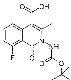
2-tert-Butoxycarbonylamino-8-fluoro-3-methyl-1-oxo-1,2-dihydro-isoquinoline-4-carboxylic acid.
