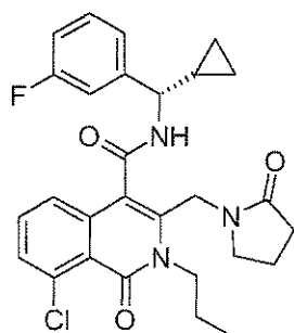
6d 8-Chloro-1-oxo-3-(2-oxo-pyrrolidin-1-ylmethyl)-2-propyl-1,2-dihydro-isoquinoline-4-carboxylic acid [(S)-cyclopropyl-(3-fluoro-phenyl)-methyl]-amide.
