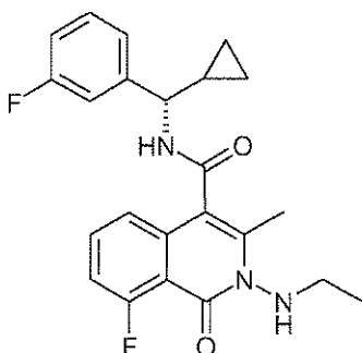
10 2p 2-Ethylamino-8-fluoro-3-methyl-1-oxo-1,2-dihydro-isoquinoline-4-carboxylic acid [(S)-cyclopropyl-(3-fluoro-phenyl)-methyl]-amide.
