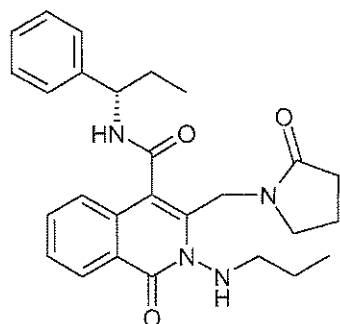
2o 1-Oxo-3-(2-oxo-pyrrolidin-1-ylmethyl)-2-propylamino-1,2-dihydro-isoquinoline-4-carboxylic acid ((S)-1-phenyl-propyl)-amide.
