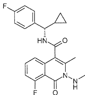
10 2v 8-Fluoro-3-methyl-2-methylamino-1-oxo-1,2-dihydro-isoquinoline-4-carboxylic acid [(S)-cyclopropyl-(4-fluoro-phenyl)-methyl]-amide.
