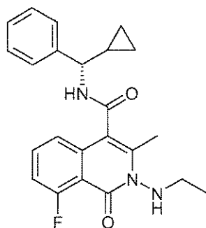
2i 2-Ethylamino-8-fluoro-3-methyl-1-oxo-1,2-dihydro-isoquinoline-4-carboxylic acid ((S)-cyclopropyl-phenyl-methyl)-amide.
