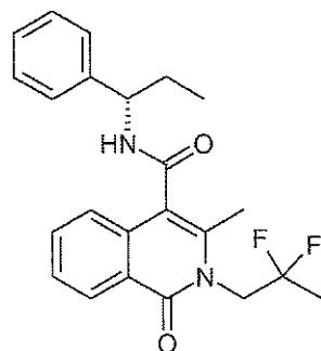
10 1aa 2-(2,2-Difluoro-propyl)-3-methyl-1-oxo-1,2-dihydro-isoquinoline-4-carboxylic acid ((S)-1-phenyl-propyl)-amide.
