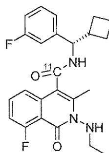
2-Ethylamino-8-fluoro-3-methyl-1-oxo-1,2-dihydro-isoquinoline-4-( 11 C)-carboxylic acid [(S)-cyclobutyl-(3-fluoro-phenyl)-methyl]-amide
