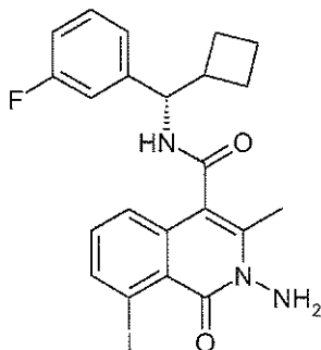
2-Amino-8-iodo-3-methyl-1-oxo-1,2-dihydro-isoquinoline-4-carboxylic acid [(S)-cyclobutyl-(3-fluoro-phenyl)-methyl]-amide.
