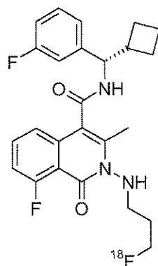
8-Fluoro-2-(3-( ^{18}\text{F} )-fluoro-propylamino)-3-methyl-1-oxo-1,2-dihydro-isoquinoline-4-carboxylic acid [(S)-cyclobutyl-(3-fluoro-phenyl)-methyl]-amide
