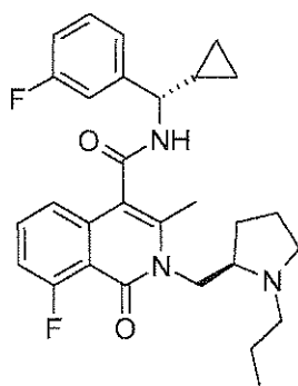
7g 8-Fluoro-3-methyl-1-oxo-2-(( R )-1-propyl-pyrrolidin-2-ylmethyl)-1,2-dihydro-isoquinoline-4-carboxylic acid [( S )-cyclopropyl-(3-fluoro-phenyl)-methyl]-amide.
