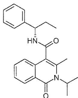
1z 2-Isopropyl-3-methyl-1-oxo-1,2-dihydro-isoquinoline-4-carboxylic acid ((S)-1-phenyl-propyl)-amide.
