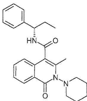
Ig 3-Methyl-1-oxo-2-piperidin-1-yl-1,2-dihydro-isoquinoline-4-carboxylic acid ((S)-1-phenyl-propyl)-amide.
