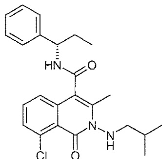
2m 8-Chloro-2-isobutylamino-3-methyl-1-oxo-1,2-dihydro-isoquinoline-4-carboxylic acid ((S)-1-phenyl-propyl)-amide.
