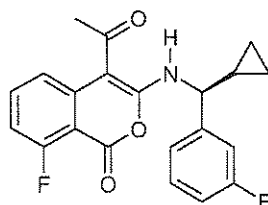
4-Acetyl-3-([(S)-cyclopropyl-(3-fluoro-phenyl)-methyl]-amino)-8-fluoro-isochromen-1-one.
