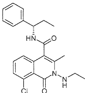
2h 8-Chloro-2-ethylamino-3-methyl-1-oxo-1,2-dihydro-isoquinoline-4-carboxylic acid ((S)-1-phenyl-propyl)-amide.
