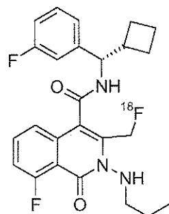
10 8-Fluoro-3-( 18 F)-fluoromethyl-1-oxo-2-propylamino-1,2-dihydro-isoquinoline-4-carboxylic acid [(S)-cyclobutyl-(3-fluoro-phenyl)-methyl]-amide
