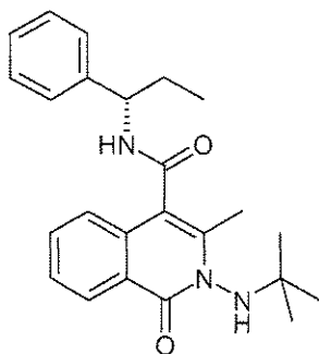
Ih 2-tert-Butylamino-3-methyl-1-oxo-1,2-dihydro-isoquinoline-4-carboxylic acid ((S)-1-phenyl-propyl)-amide.
