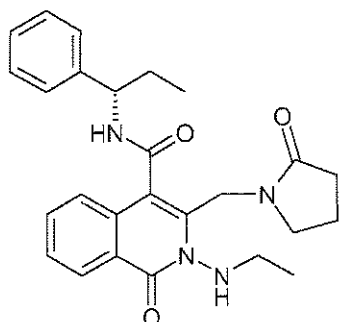
2n 2-Ethylamino-1-oxo-3-(2-oxo-pyrrolidin-1-ylmethyl)-1,2-dihydro-isoquinoline-4-carboxylic acid ((S)-1-phenyl-propyl)-amide.
