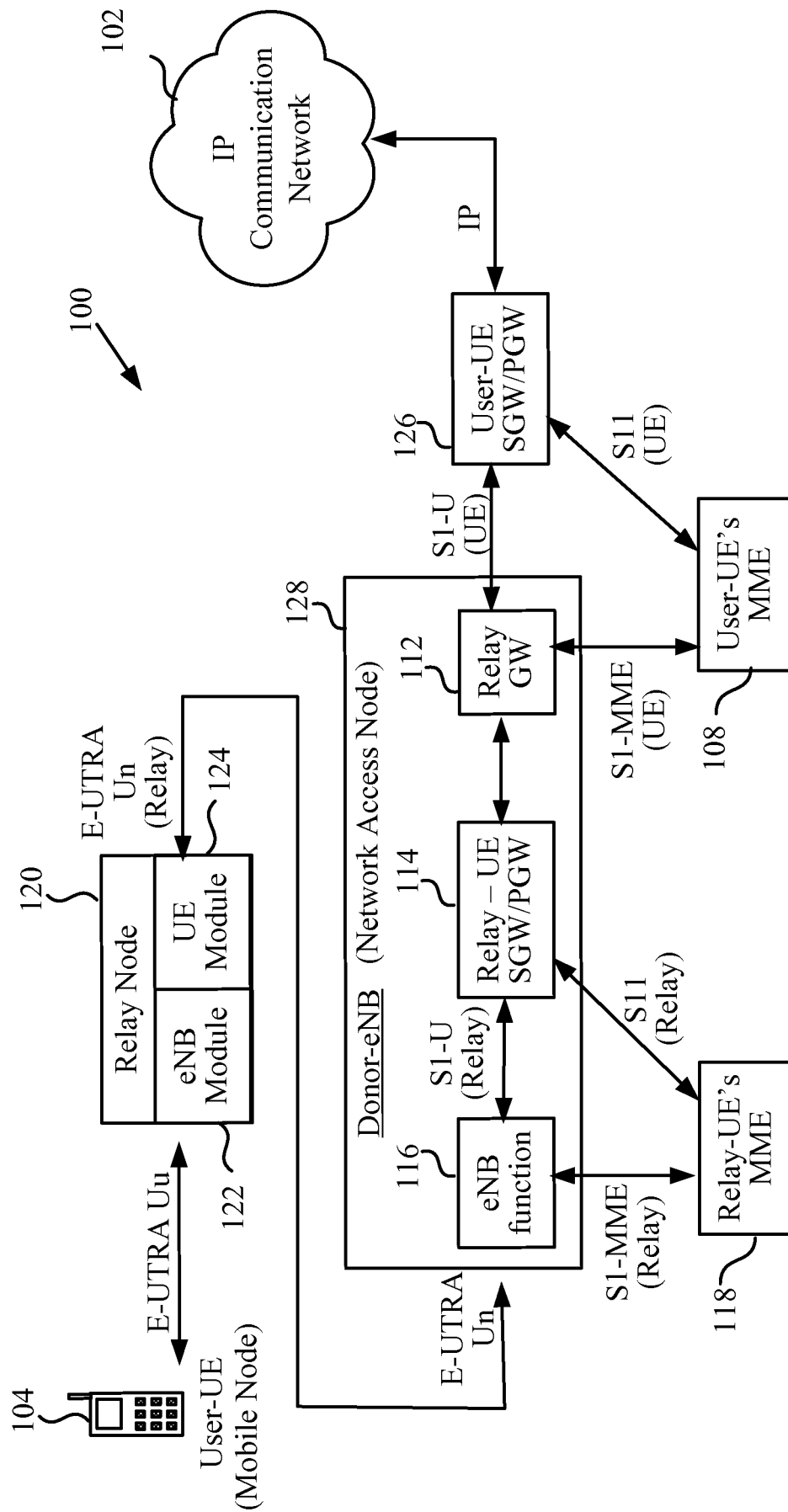
EXEMPLARY COMMUNICATION NETWORK WITH RELAY NODE
