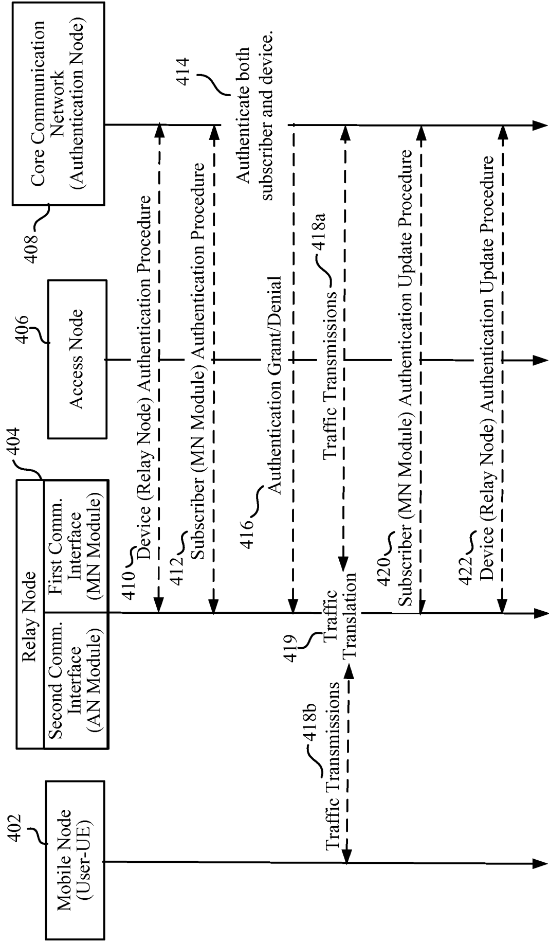
FIG. 4 RELAY NODE AUTHENTICATION SCHEME
