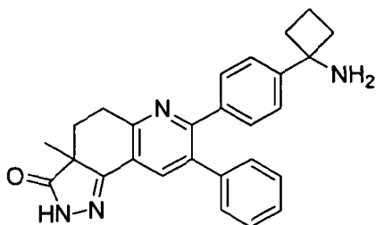
7-(4-(1-aminocyclobutyl)phenyl)-3a-methyl-8-phenyl-4,5-dihydro-2H-pyrazolo[3,4-f]quinolin-3(3aH)-one
