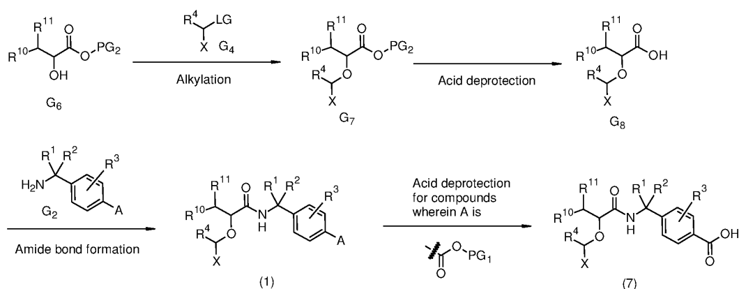
Scheme 2
