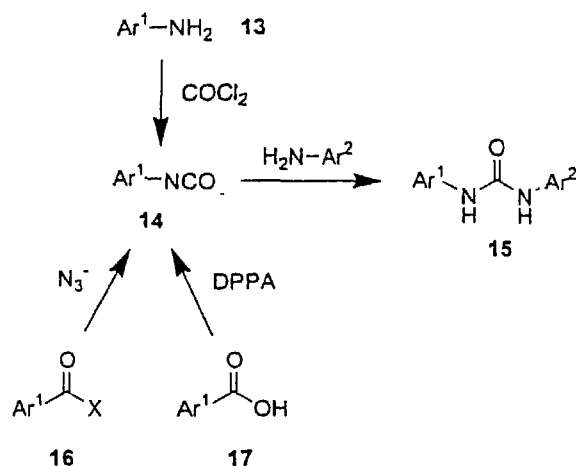
Scheme IV Selected Methods of Non-Symmetrical Urea Formation
