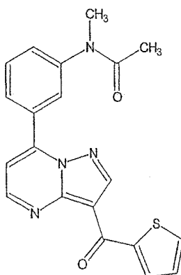
Indiplon
