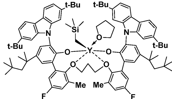
Inventive Metal-Ligand Complex 4
