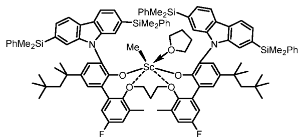
Inventive Metal-Ligand Complex 8
