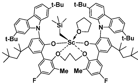
Inventive Metal-Ligand Complex 5
