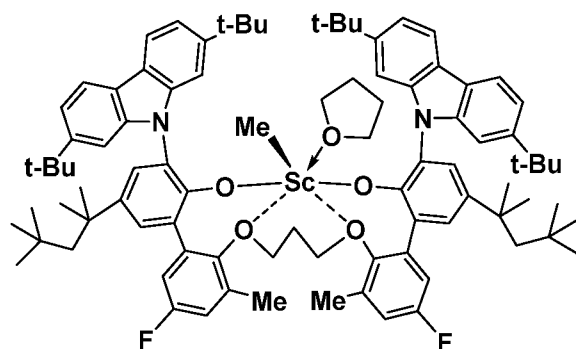
Inventive Metal-Ligand Complex 7
