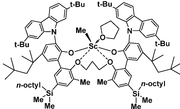
Inventive Metal-Ligand Complex 6
