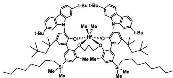
Comparative Metal-Ligand Complex 1 (C1)
