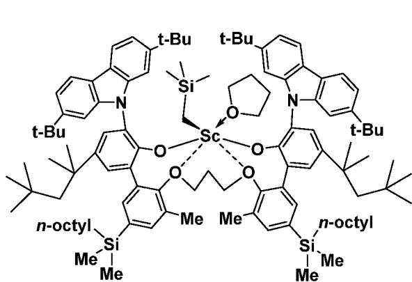
Inventive Metal-Ligand Complex 1
