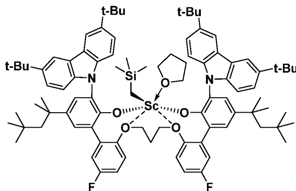
Inventive Metal-Ligand Complex 2
