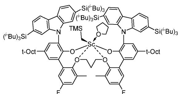
Inventive Metal-Ligand Complex 9
