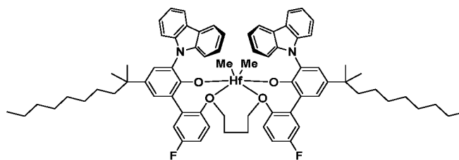
Comparative Metal-Ligand Complex 2 (C2)
