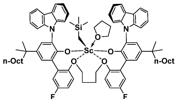
Inventive Metal-Ligand Complex 3
