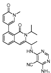
Compound 359,
