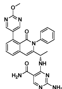
Compound 11,
