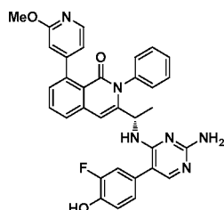
Compound 159,
