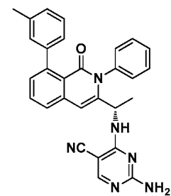
Compound 46,
