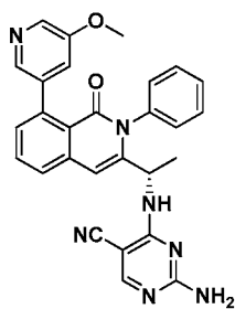
Compound 9,
