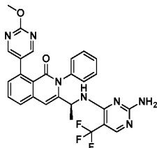
Compound 12,
