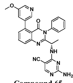
Compound 65,
