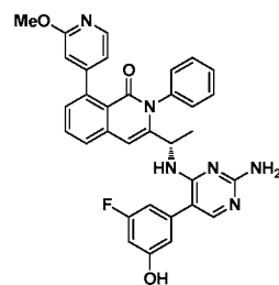
Compound 161,
