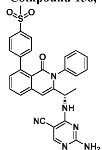
Compound 165,
