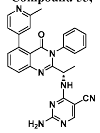
Compound 62,
