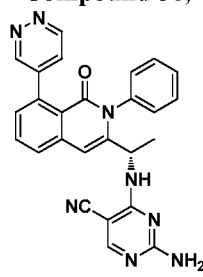
Compound 57,
