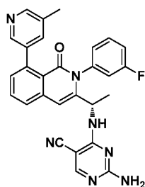
Compound 26,
