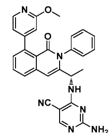
Compound 49,
