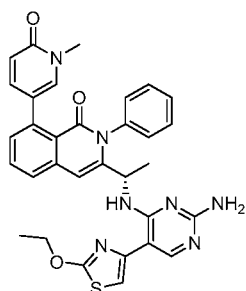
Compound 138,
