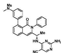
Compound 153,
