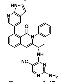
Compound 47,
