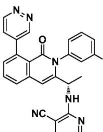
Compound 30,
