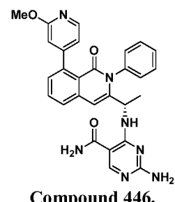
Compound 446,
