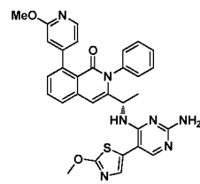
Compound 140,
