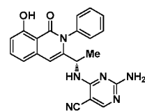
Compound 145,
