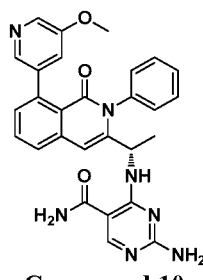
Compound 10,
