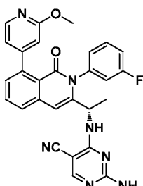
Compound 28,
