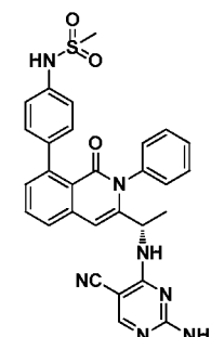
Compound 167,
