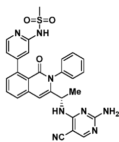
Compound 443,
