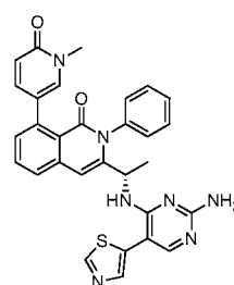
Compound 387,
