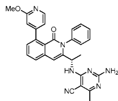
Compound 364,
