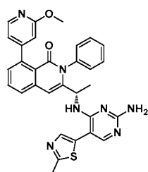
Compound 181,
