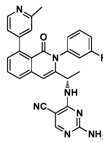
Compound 24,
