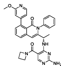
Compound 154,
