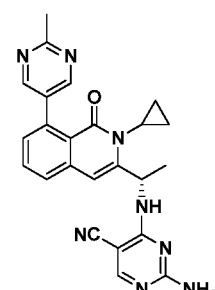
Compound 445,
