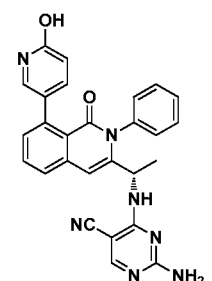
Compound 156,
