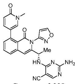
Compound 338,
