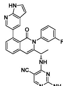
Compound 25,
