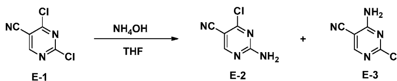
Method E':
