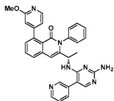
Compound 133,
