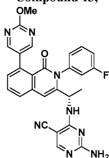
Compound 22,
