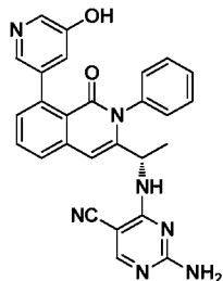
Compound 13,
