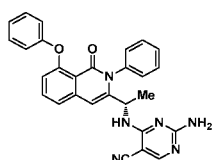
Compound 151,
