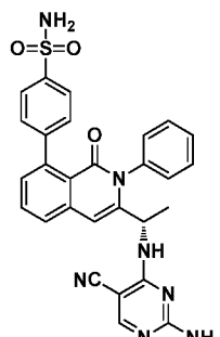
Compound 45,
