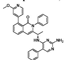
Compound 179,
