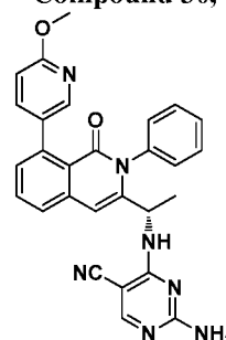
Compound 35,
