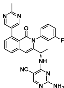
Compound 20,
