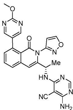
Compound 337,
