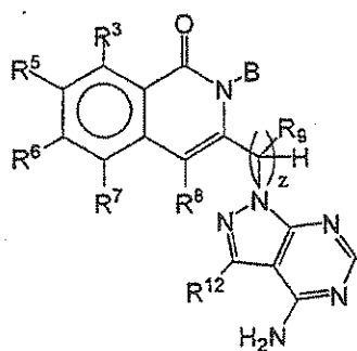
Formula VI-B
