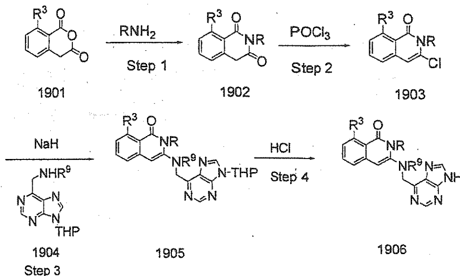
Reaction Scheme 19:
