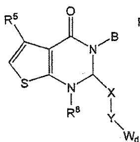
Formula 9-AH
