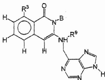
Formula 6-D
