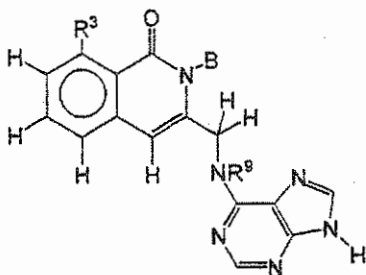
Formula 6-C2
