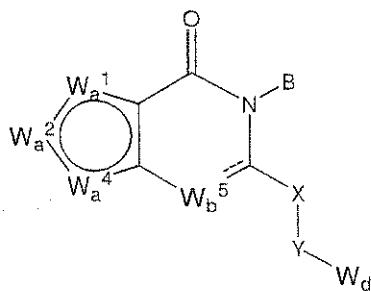
Formula IX
