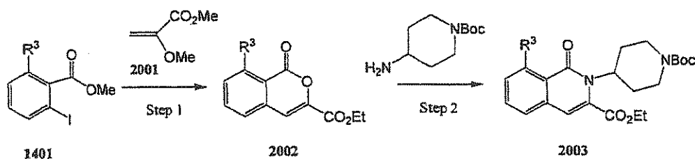
Reaction Scheme 20:
