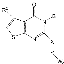
Formula XIII
