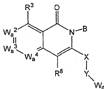
Formula 2-B
