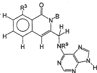
Formula VI-B
