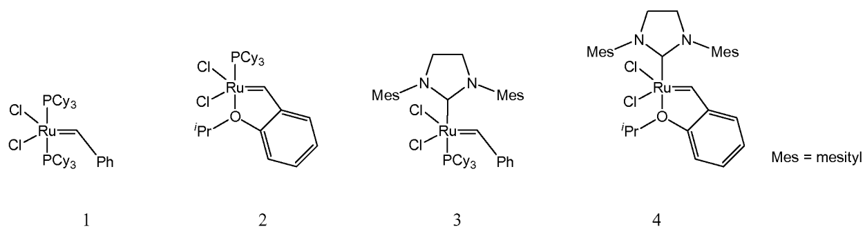
Figure 1. Typical Grubbs' Catalysts
