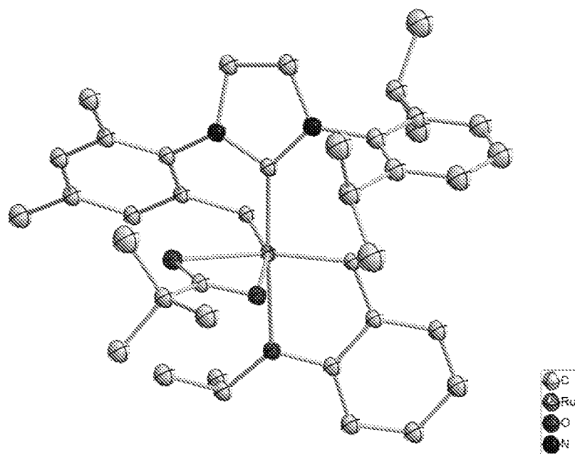
Figure 6. X-ray crystal structure of complex 11
