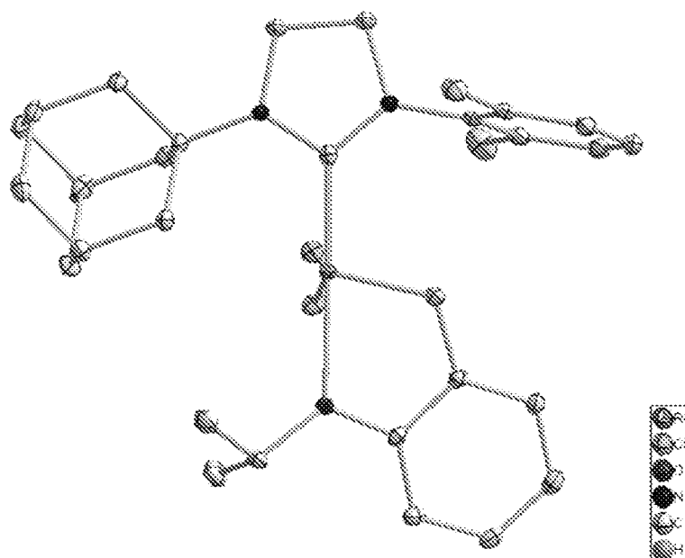
Figure 8. X-ray crystal structure of complex 18b
