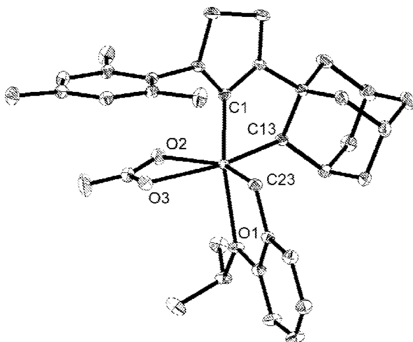
Figure 12. X-ray crystal structure of complex 22e
