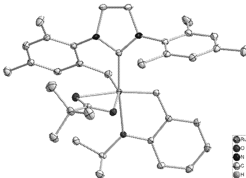
Figure 4. X-ray crystal structure of complex 7a
