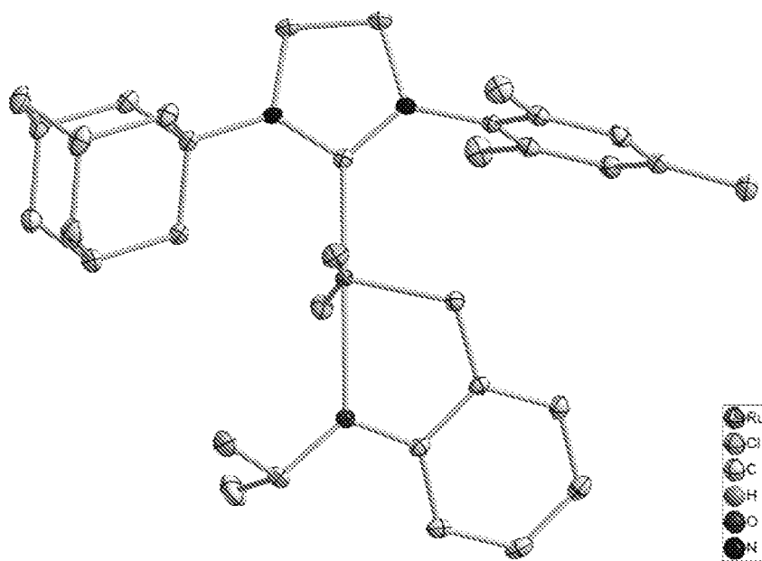
Figure 7. X-ray crystal structure of complex 18a
