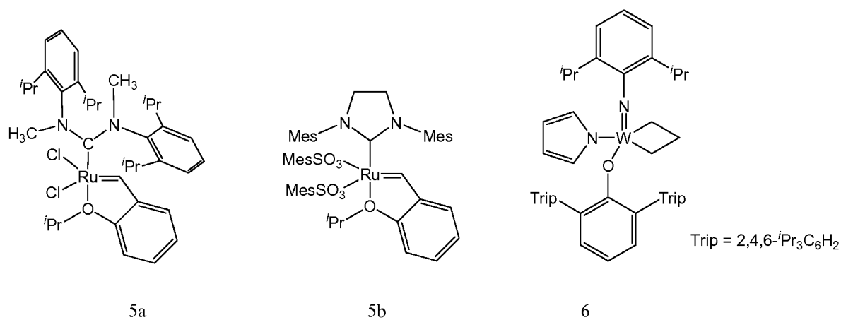
Figure 2. Recently Reported Olefin Metathesis Catalysts
