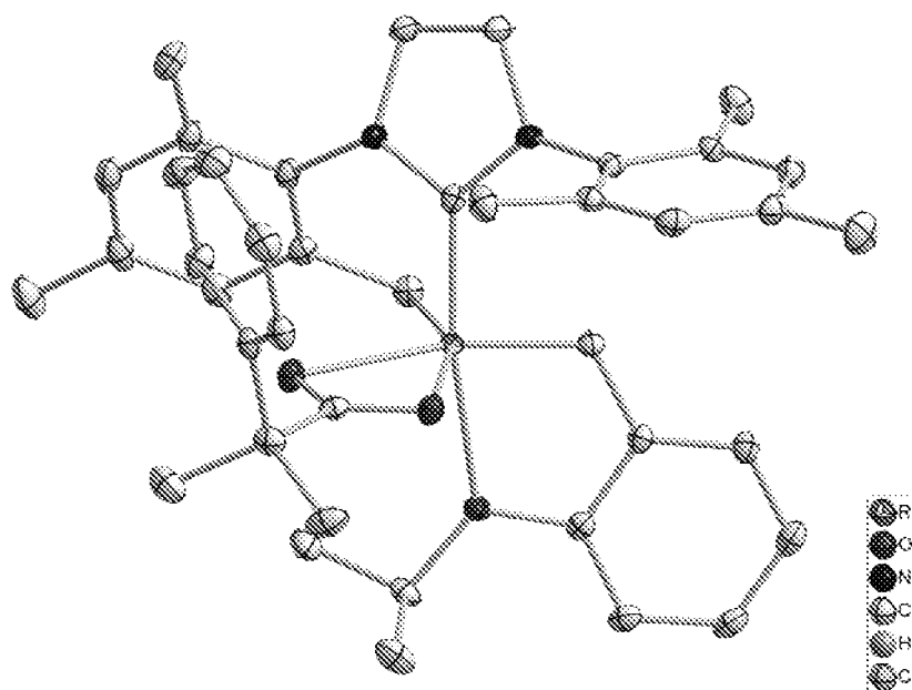
Figure 5. X-ray crystal structure of complex 7b
