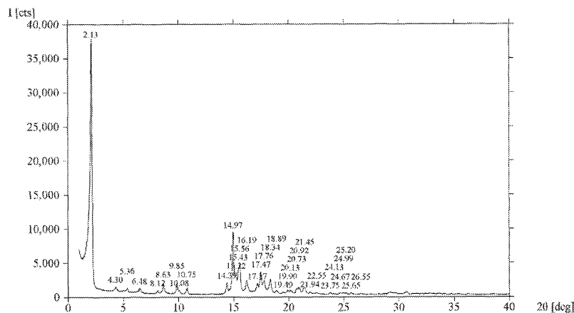
Figure 1 – Form I XRPD Diffractogram
