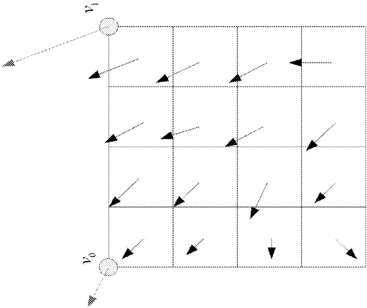
Affine subblock motion vector field
