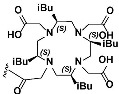
tetra-(S,S,S,S)-iBu-DOTA
