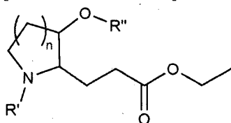
[Chemical Formula 3-D]
