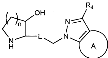
[Chemical Formula 1-5]
