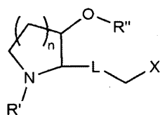
[Chemical Formula 1-B]
