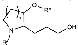
[Chemical Formula 3-F]
