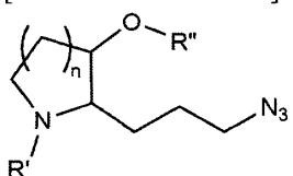
[Chemical Formula 3-G]
