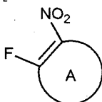
[Chemical Formula 2-C]
