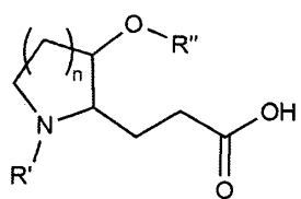
[Chemical Formula 3-E]
