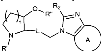
[Chemical Formula 2-D]
