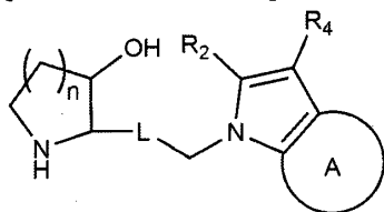
[Chemical Formula 1-3]
