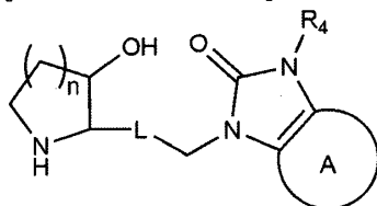
[Chemical Formula 1-4]
