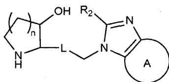
[Chemical Formula 2-A]
