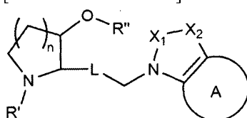
[Chemical Formula 1-C]
