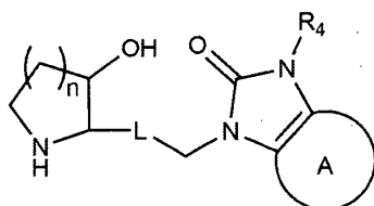
[Chemical Formula 1-4]
