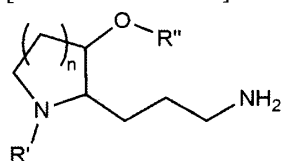
15 [Chemical Formula 3-A]
