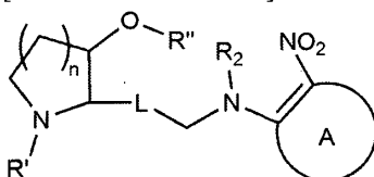
[Chemical Formula 2-D]
