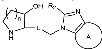
[Chemical Formula 1-2]
