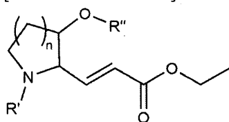
[Chemical Formula 3-C]
