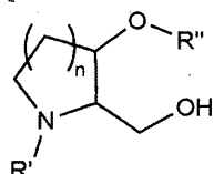
[Chemical Formula 3-B]
