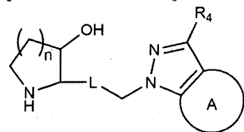
[Chemical Formula 1-5]
