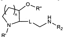
[Chemical Formula 2-B]
