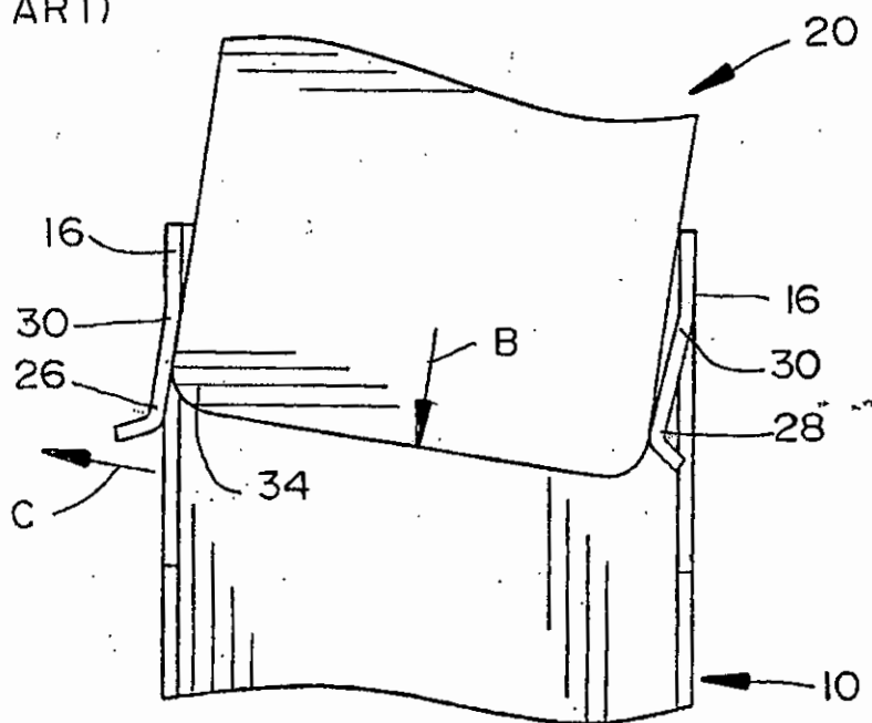
FIG.8 (PRIOR ART)
