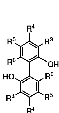
Structure III
