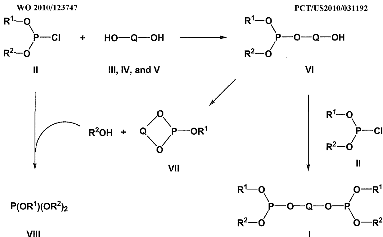
Scheme I
