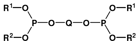
Structure I
