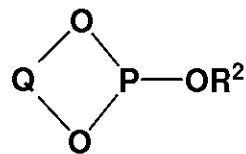
Structure VIb
