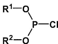
Structure II
