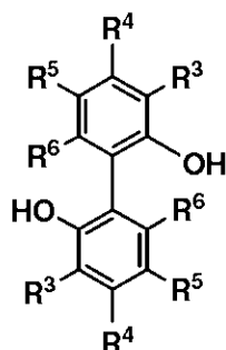
Structure III
