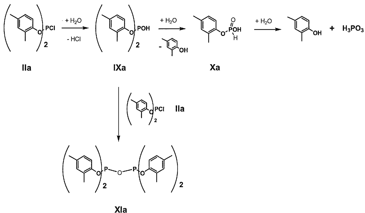
Scheme IV
