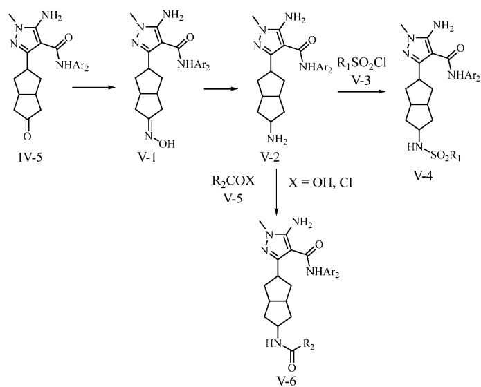
Scheme V
