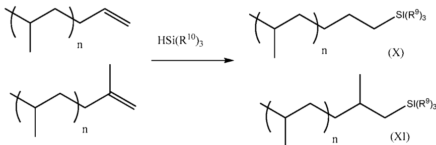
Scheme V
