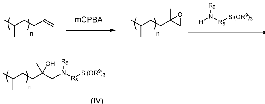
Scheme IV
