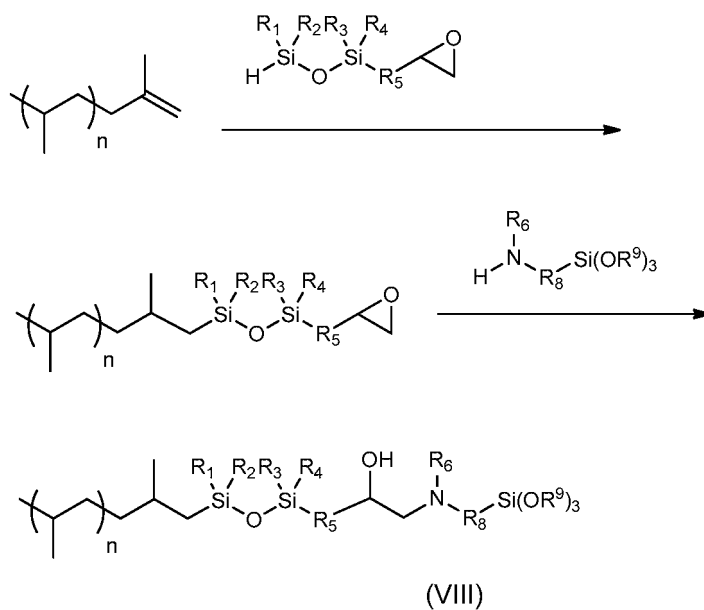
Scheme III
