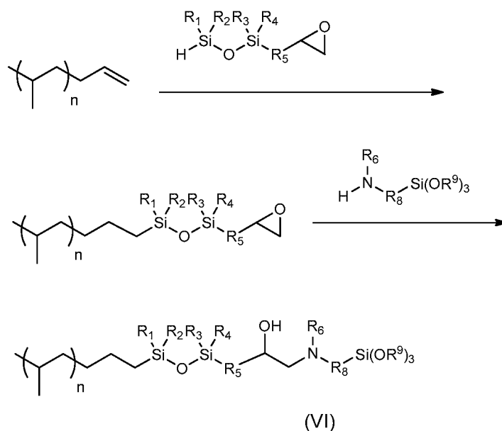
Scheme I
