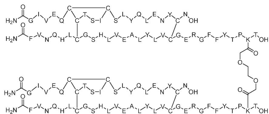
Dimer 3;
