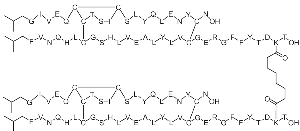
Dimer 65;
