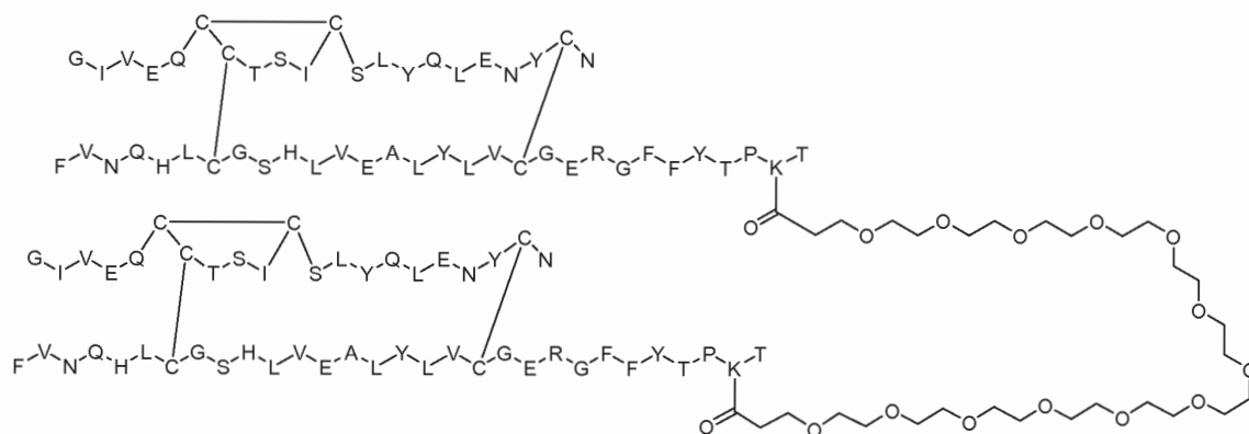
Dimer 6;
