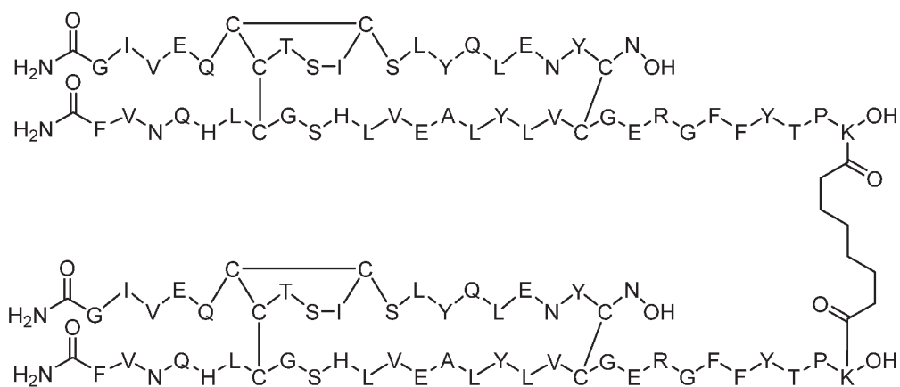
Dimer 28;
