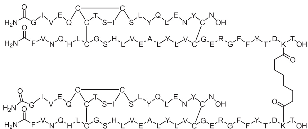
Dimer 83;
