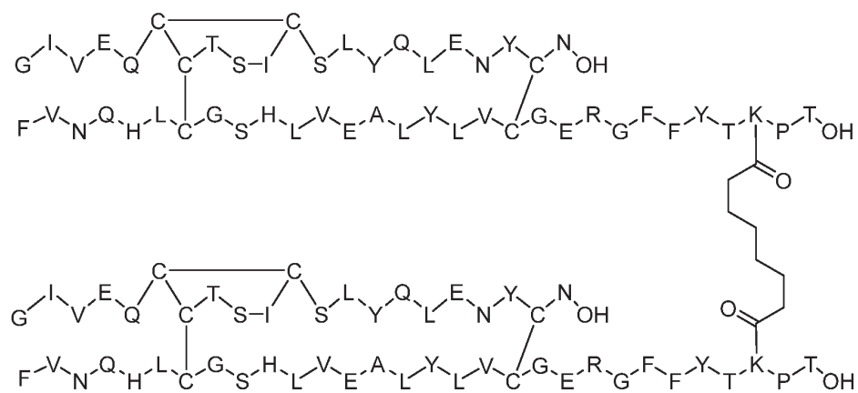
Dimer 18;
