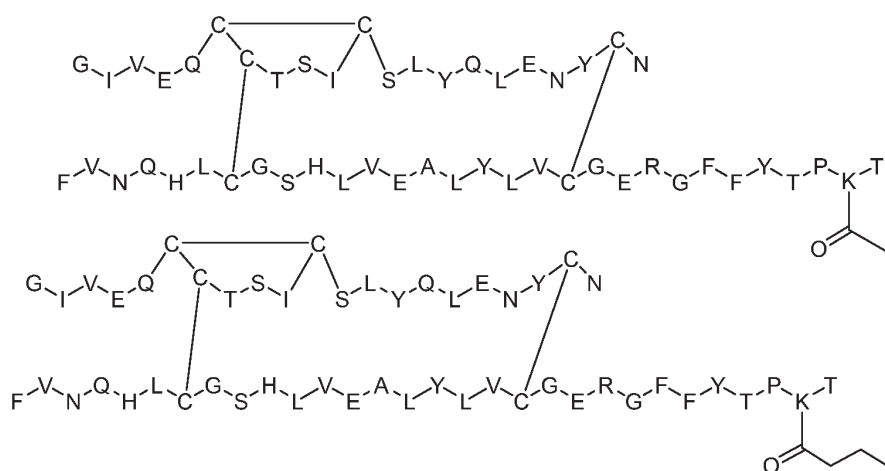
Dimer 9;
