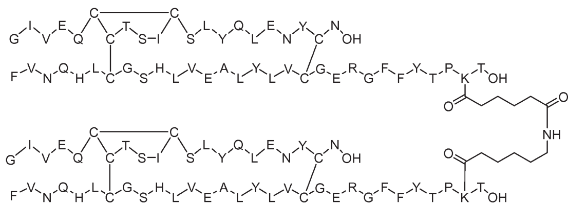
Dimer 22;
