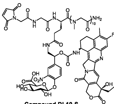
Compound DL10-S
