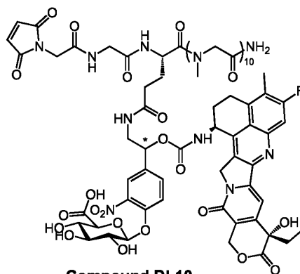
Compound DL10
