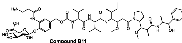
Compound B11
