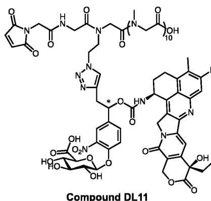
Compound DL11
