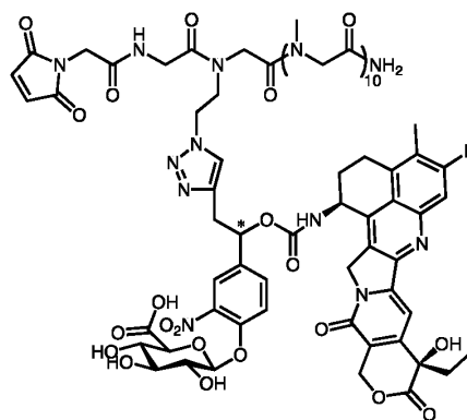
Compound DL2
