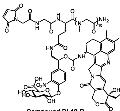
Compound DL10-R
