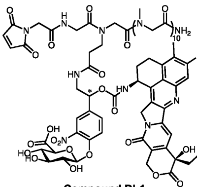
Compound DL1
