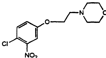
Compound 35
