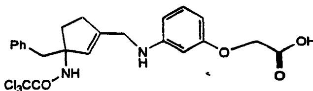
Cpd 45
