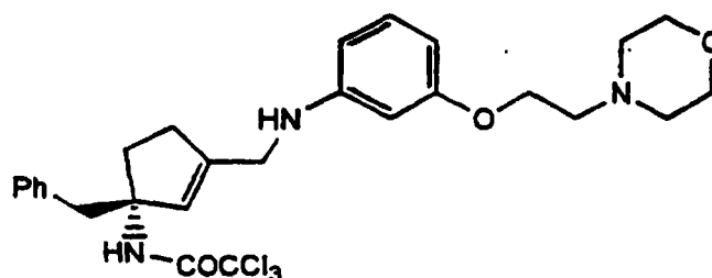
Cpd. 6b
