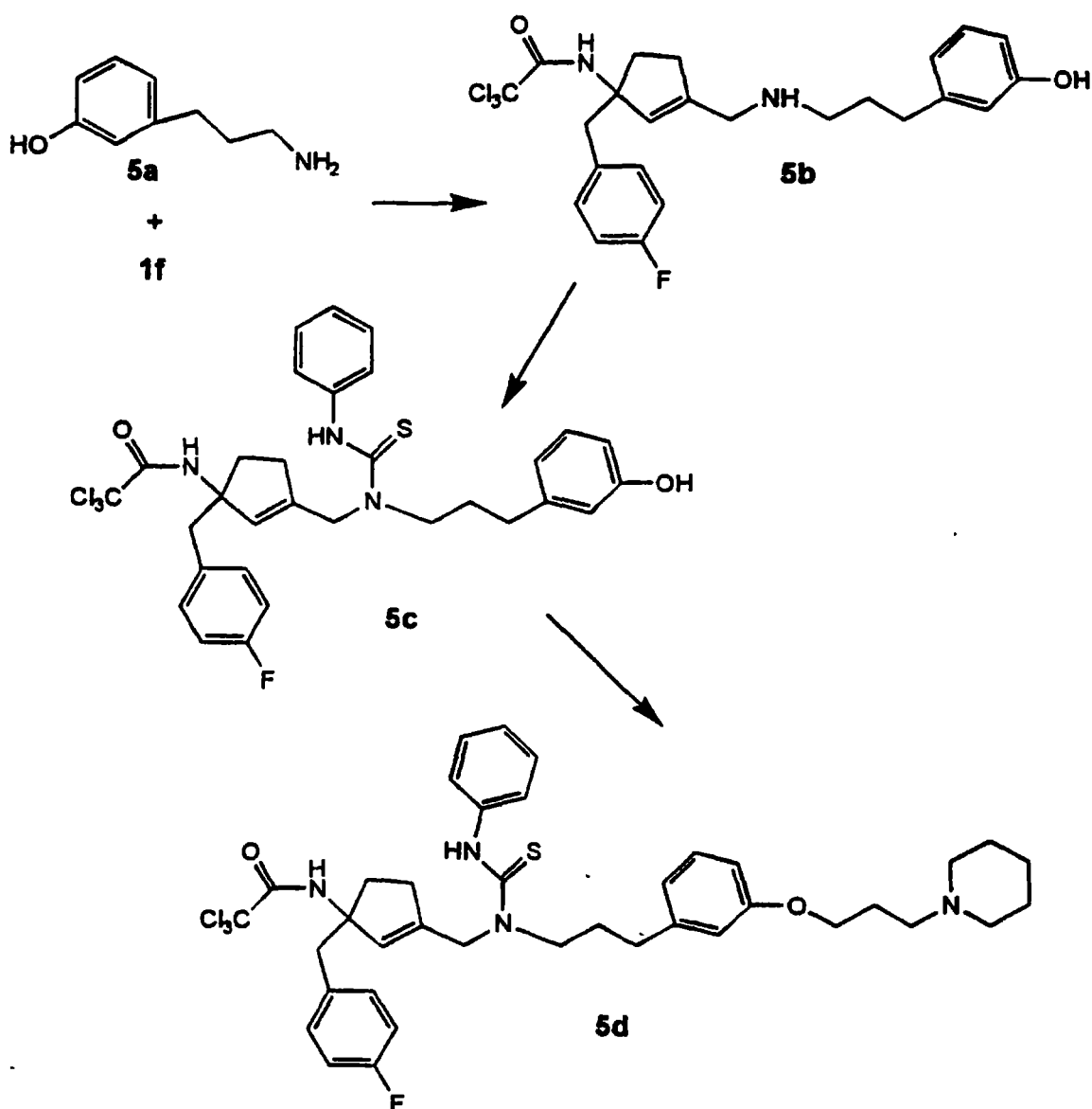
Scheme 5
