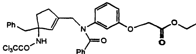
Cpd 46
