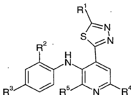
Formula (IIa)
