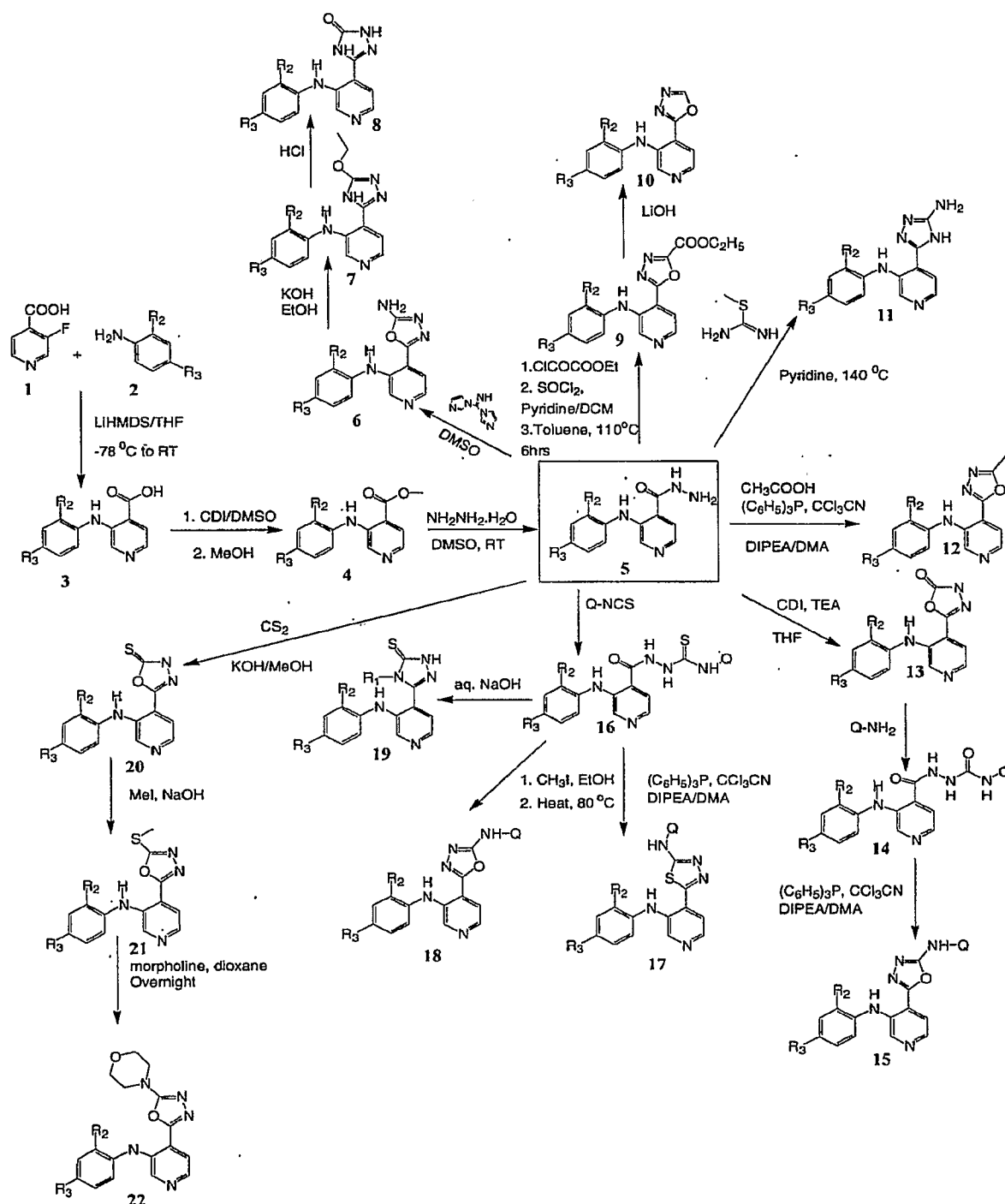
Scheme 1
