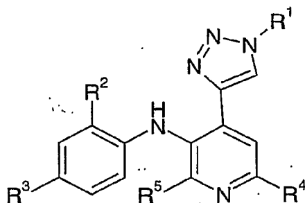
Formula (IIb)
