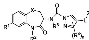
Formula I-10
