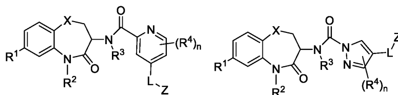
Formula I-5
