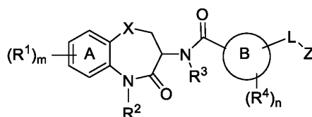
5 Formula I
