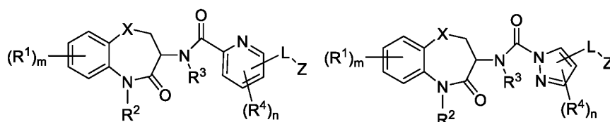
Formula I-3
