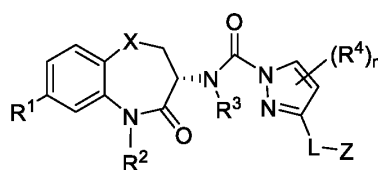
Formula I-13
