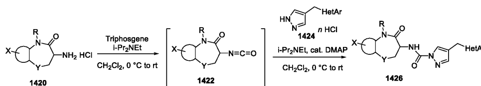
Scheme 8
