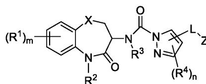
Formula I-4
