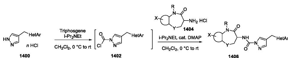
Scheme 7
