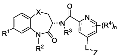
Formula I-9
