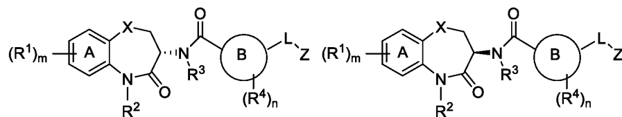
Formula I-1
