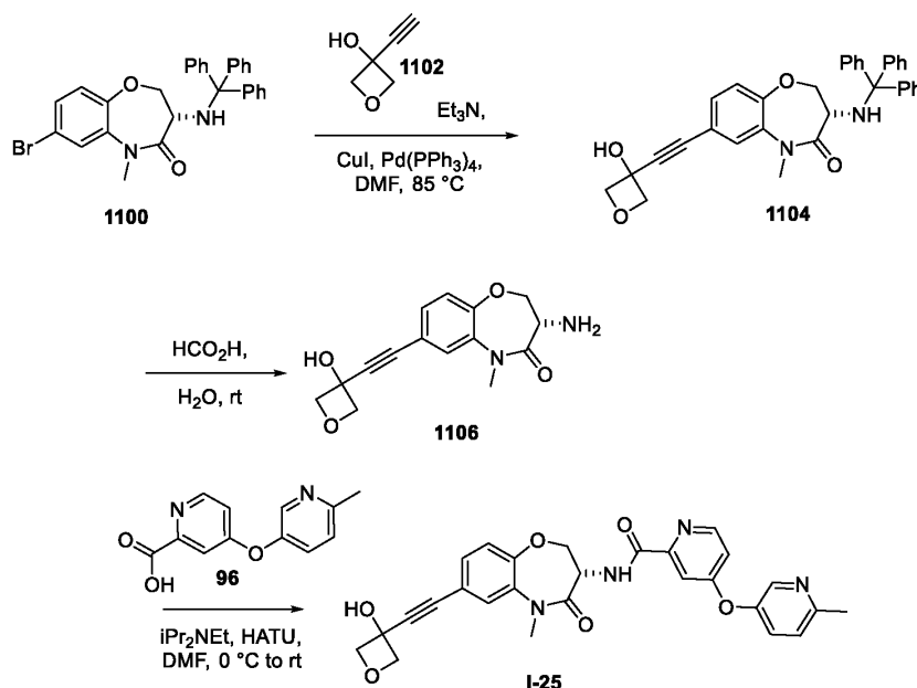
Scheme 12
