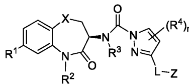
Formula I-12
