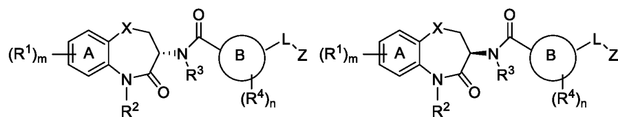
Formula I-1
