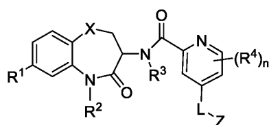
Formula I-5
