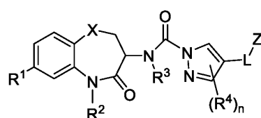
Formula I-6
