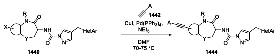
Scheme 9
