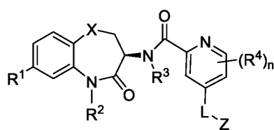
Formula I-7
