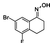
Scheme 13
