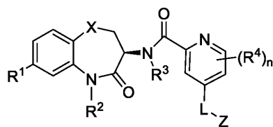
Formula I-7
