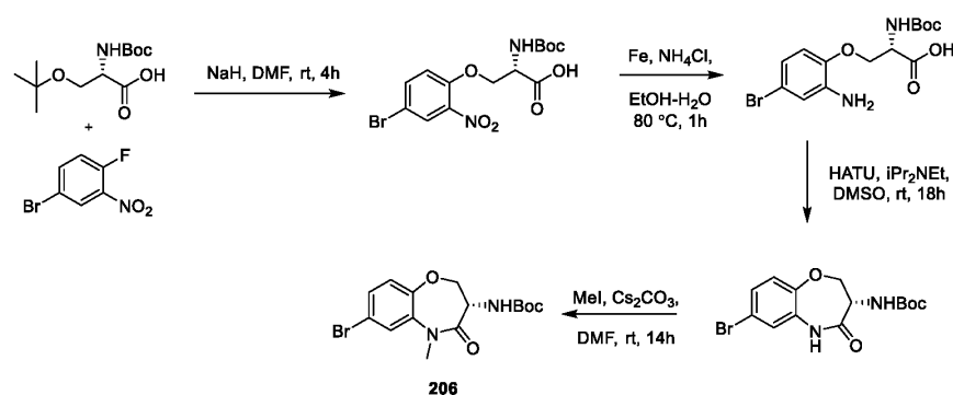
Scheme 6B
