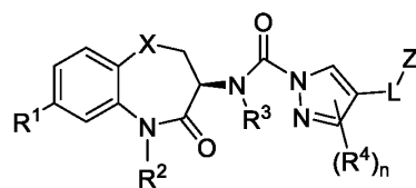
Formula I-8
