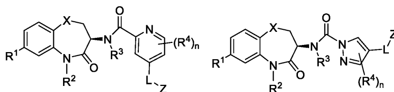
Formula I-7
