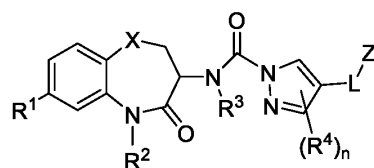
Formula I-6
