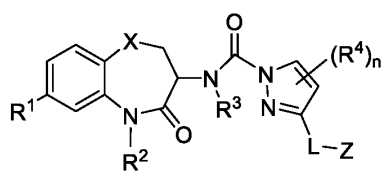
Formula I-11
