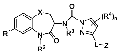
Formula I-11
