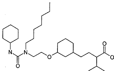
cis/diastereomer mixture
