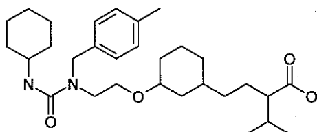
cis/diastereomer mixture
