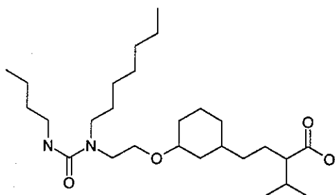
cis/diastereomer mixture
