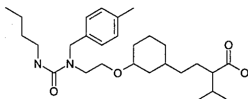
cis/diastereomer mixture
