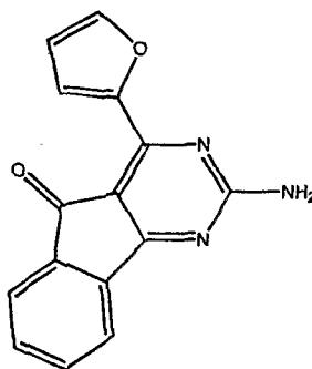
2-amino-4-furan-2-yl-indeno[1,2-d]pyrimidin-5-one
