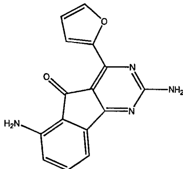
2,6-diamino-4-furan-2-yl-indeno[1,2-d]pyrimidin-5-one
