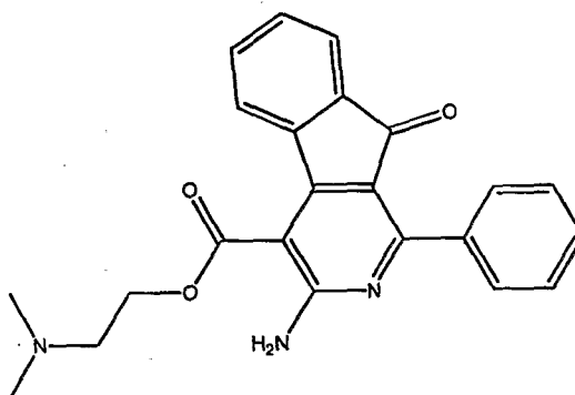
5 9H-indeno[2,1-c]pyridine-4-carboxylic acid, 3-amino-1-phenyl-9-oxo-, 2-dimethylamino-ethyl ester
