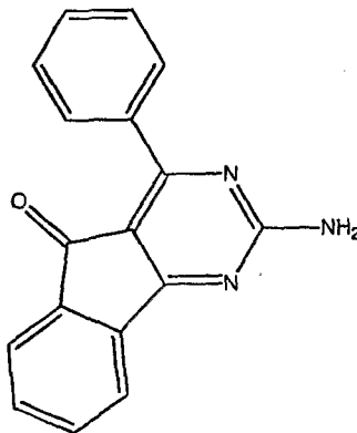
2-amino-4-phenyl-indeno[1,2-d]pyrimidin-5-one
