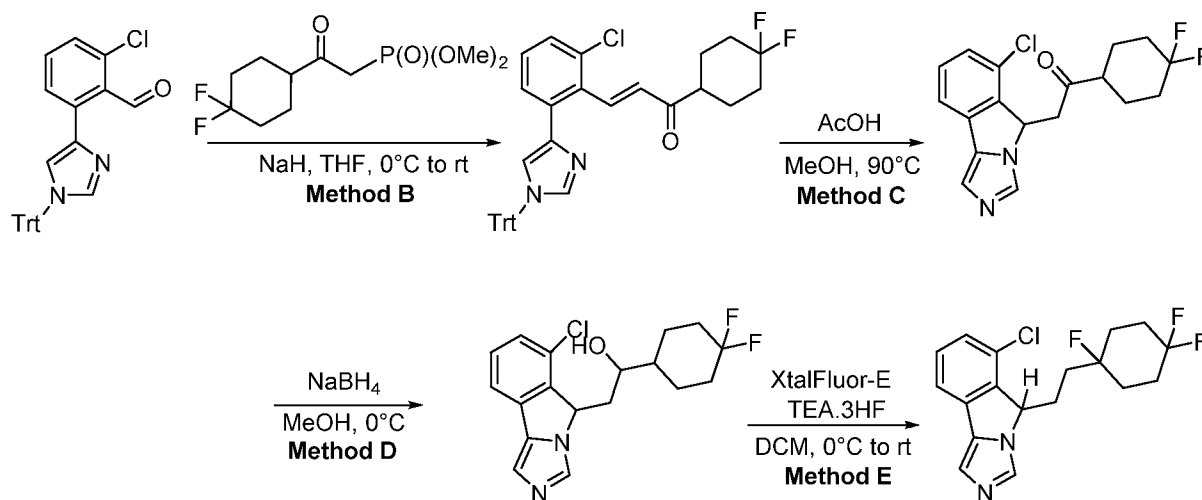
Compound 72a and b
