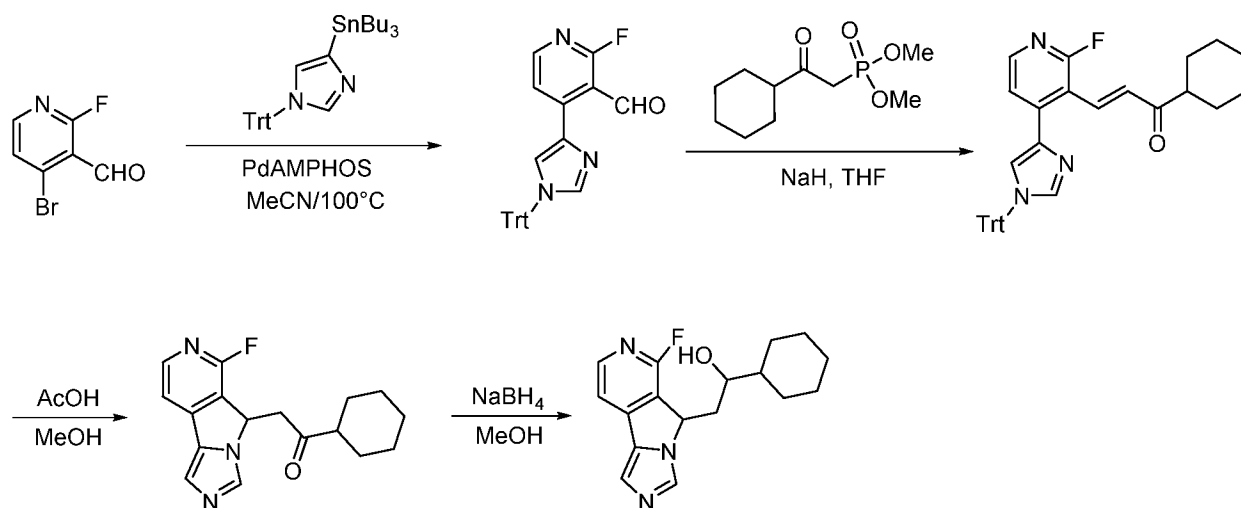
Compound 2a and 2b
