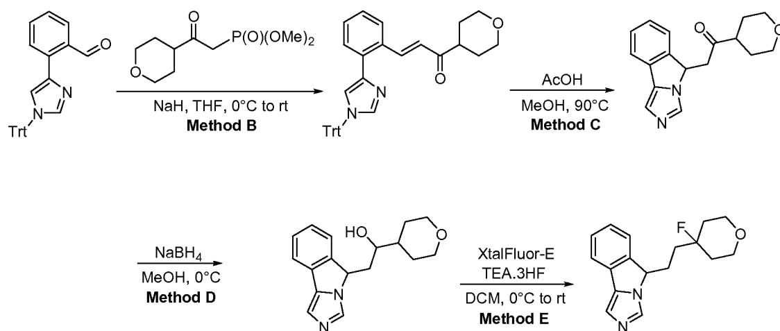
Compound 94a and 94b
