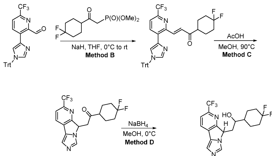
Compounds 77a, b, c, d
