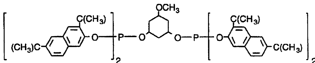
Ligand S
