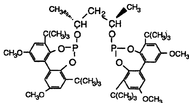
Ligand M
