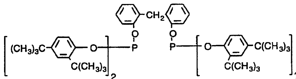
Ligand U
