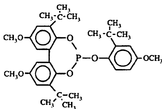
Ligand A
