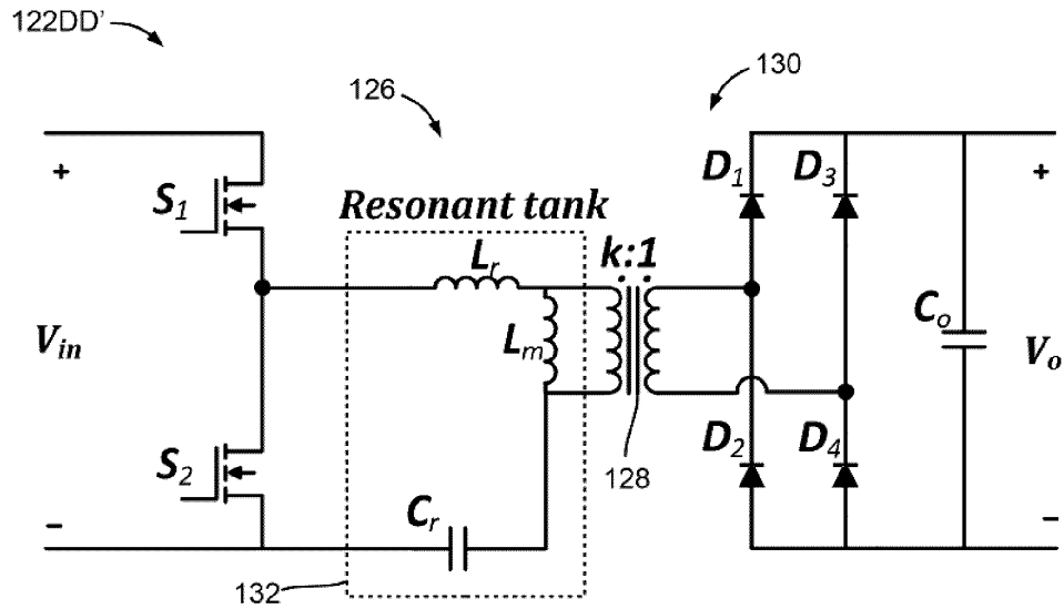
FIG. 11 (Prior Art)
