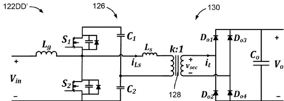
FIG. 12 (Prior Art)
