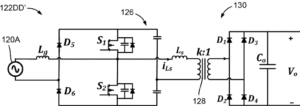
FIG. 13 (Prior Art)
